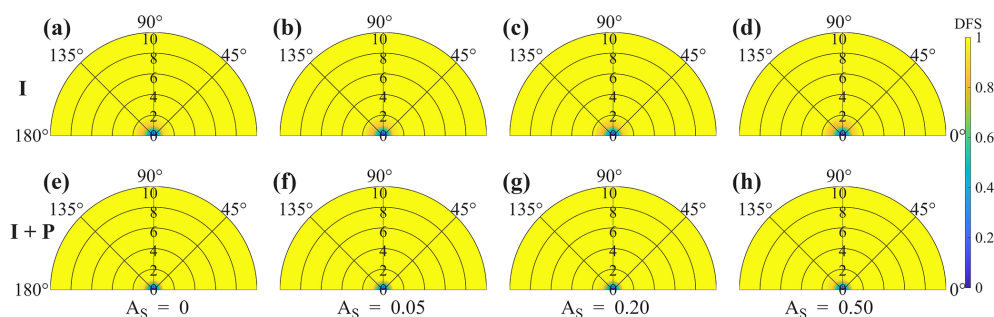
Figure 6. Same as Fig. 2, but with VZA = 80°.
