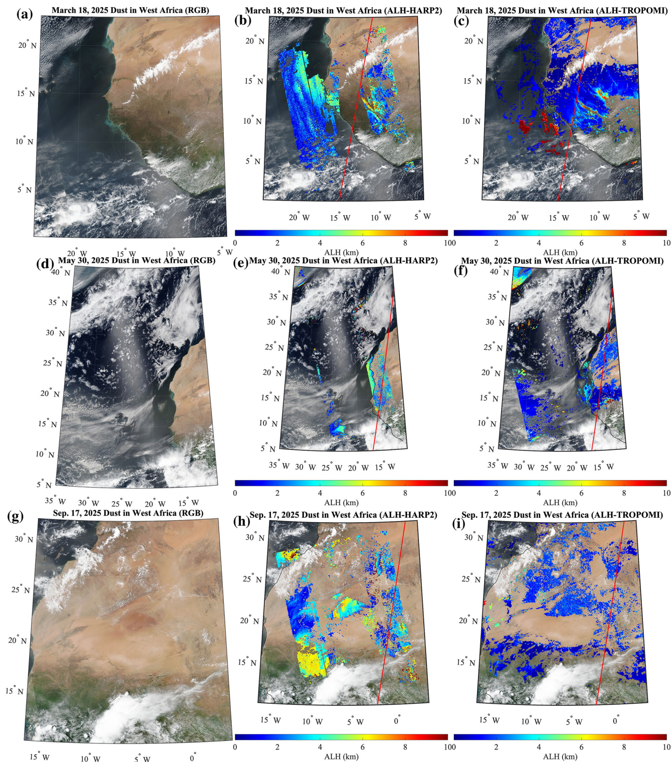
Figure 10. Examples of retrieval for dust cases. The first column (a, d, g) presents the corresponding true-color images from VIIRS/Suomi-NPP. The second column (b, e, h) displays the HARP2-derived ALH relative to sea level with the red line representing the EarthCARE track. The third column (c, f, i) presents the TROPOMI Level 2 ALH product.
