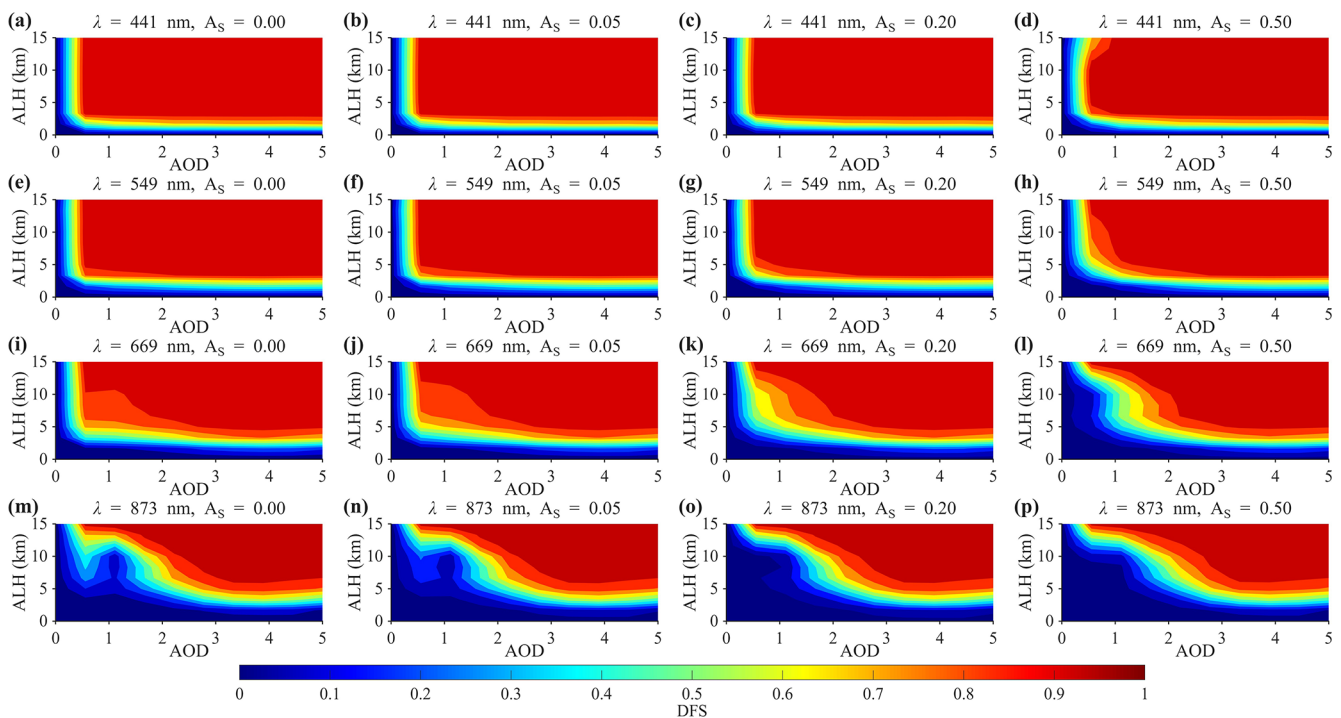
Figure 1. Characteristics of ALH-AOD 441 -DFS distributions derived from radiance under different spectral bands and surface reflectance conditions. The simulations were conducted for smoke aerosols, with AOD 441 ranging from 0 to 5 as the common reference aerosol loading parameter. For all subplots, the x-axis represents AOD 441 . Rows correspond to wavelengths of 441, 549, 669, and 873 nm, respectively, while columns represent different surface reflectance conditions ( A_s = 0.00, 0.05, 0.20, 0.50 ). Colors indicate the DFS values of ALH, ranging from 0 to 1.
