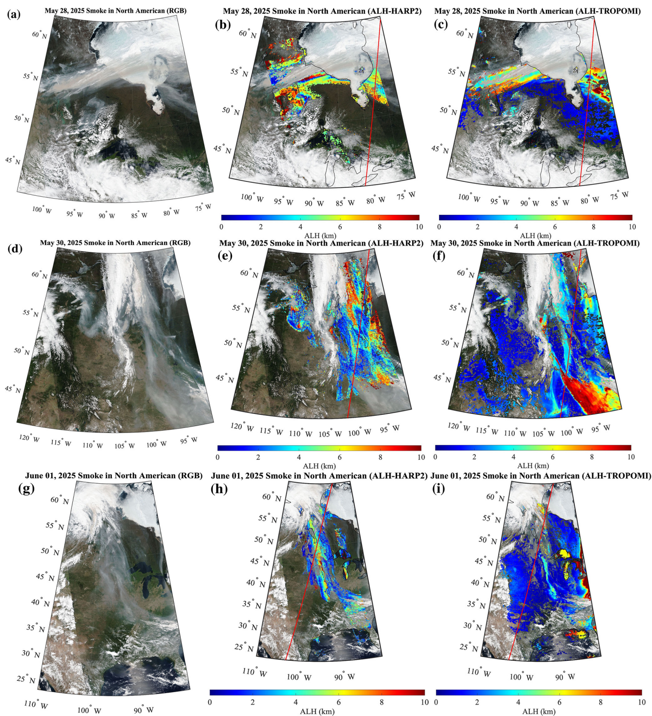
Figure 8. Examples of retrieval for smoke cases. The first column (a, d, g) presents the corresponding true-color images from VIIRS/Suomi-NPP. The second column (b, e, h) displays the HARP2-derived ALH relative to sea level with the red line representing the EarthCARE track. The third column (c, f, i) presents the TROPOMI Level 2 ALH product.
