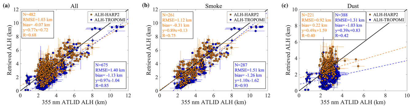
Figure 13. Comparison of the ALH-HARP2, ALH-TROPOMI with the corresponding ATLID in all cases on a pixel-by-pixel measurement value. (a) Scatter plots of matched ALH-HARP2 (orange markers) and ALH-TROPOMI (blue markers) against ATLID observations, including all matched pixel pairs from all cases. (b) Same as panel (a), but only including the smoke aerosol cases. (c) Same as panel (a), but only including the dust cases. The dashed lines in the scatter plots represent the linear regression fits. The one-to-one reference line (black solid line), the number of samples ( N ), the linear regression equation, and the correlation coefficient ( R ) are also indicated in the figure. Error bars for both the retrieved ALH and the ATLID-observed ALH represent the standard deviation of values aggregated within a 10 \text{ km} \times 10 \text{ km} spatial window.
