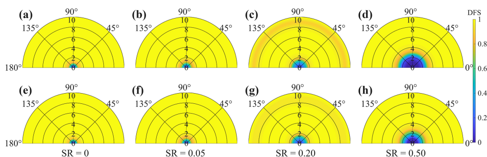
Figure 2. Comparison of ALH-DFS distributions under different combinations of observational information ( I vs. I + P ) and surface reflectance conditions. The DFS values were calculated by varying ALH (radial axis: 0–10 km) and RAA (angular axis: 0–180°), while other parameters were fixed at VZA = 0^\circ , SZA = 40^\circ , and AOD = 0.3 . The top row shows DFS calculated using radiance ( I ) only, while the bottom row shows DFS obtained by combining radiance and polarization information ( I + P ). Columns correspond to different surface reflectance values ( A_s = 0.00, 0.05, 0.20, 0.50 ).
