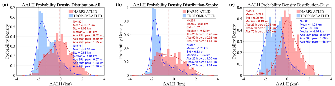
Figure 14. Histograms and statistical metrics of the differences between ALH-HARP2, ALH-TROPOMI, and ATLID observations at the co-located are presented. The statistics include the total number of data points ( N ), mean, standard deviation, and median, with the dashed line representing the median value. Panel (a) includes all cases, while panels (b) and (c) correspond to smoke and dust cases, respectively.
