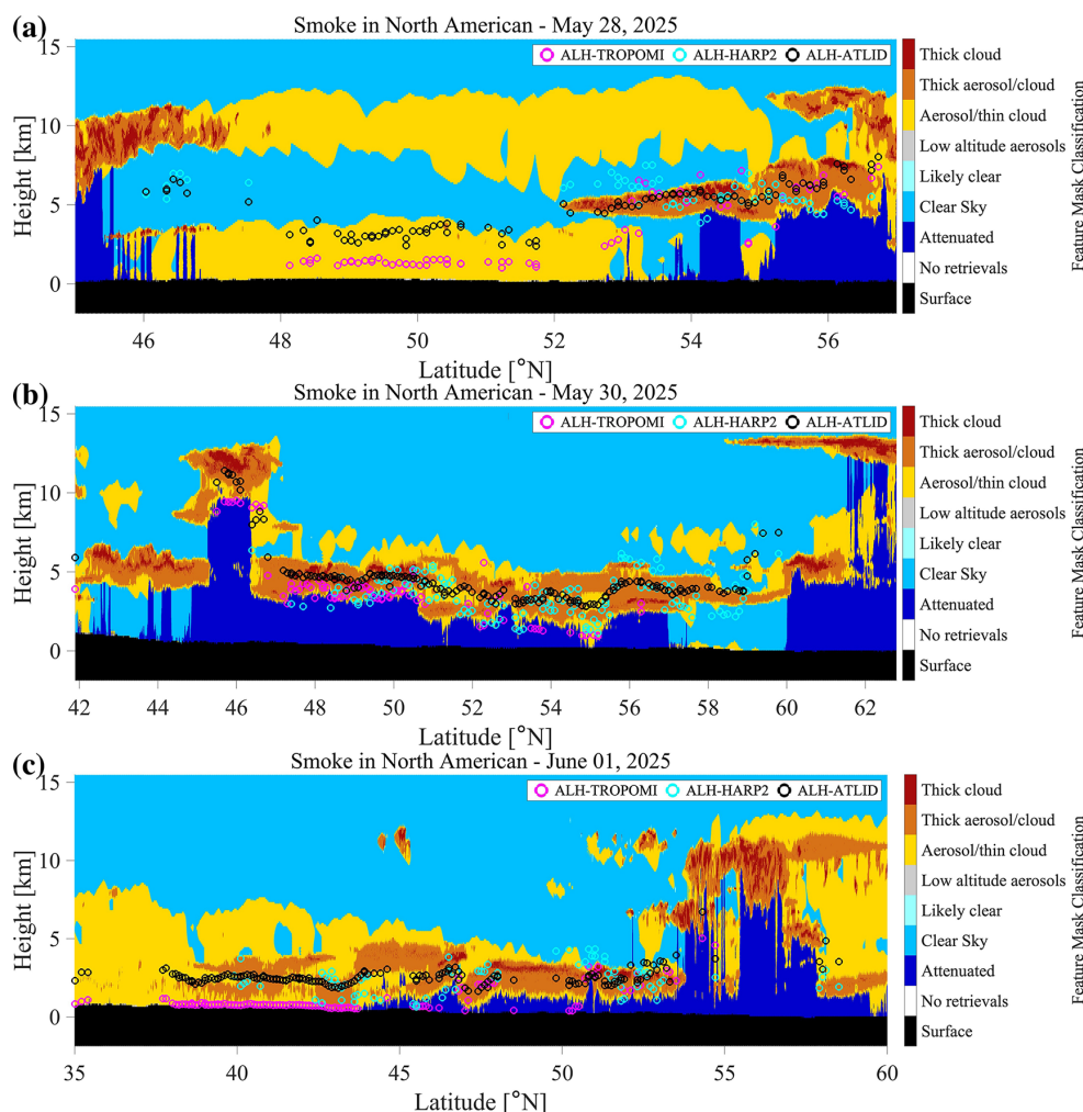
Figure 9. Comparison of ALH-HARP2 and ALH-TROPOMI with the corresponding ATLID measurements for smoke cases on the feature classification curtain plot. Panels (a)–(c) present comparisons of ALH-HARP2 and ALH-TROPOMI with ATLID in three smoke cases, respectively.
