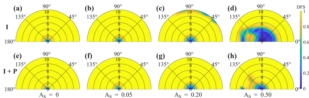
Figure 4. Same as Fig. 2, but with VZA = 40^\circ .
