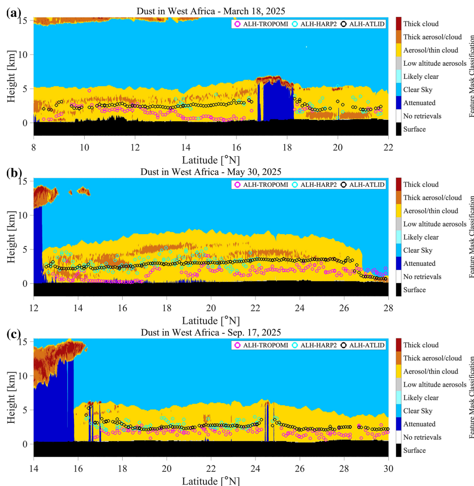
Figure 11. Comparison of ALH-HARP2 and ALH-TROPOMI with the corresponding ATLID measurements for dust cases on the feature classification curtain plot. Panels (a)–(c) present comparisons of ALH-HARP2 and ALH-TROPOMI with ATLID in three dust cases, respectively.
