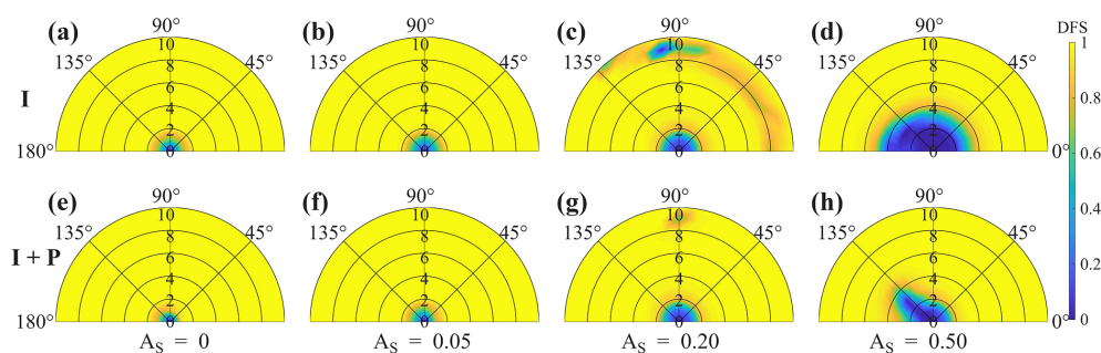
Figure 3. Same as Fig. 2, but with VZA = 20^\circ .
