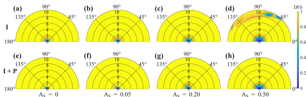
Figure 5. Same as Fig. 2, but with VZA = 60°.
