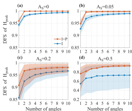
Figure 7. Influence of the number of viewing angles and polarization information on the DFS under different surface reflectance conditions A_s . Panels (a)–(d) correspond to surface reflectance values of 0, 0.05, 0.20, and 0.50, respectively. Red curves represent joint observations of radiance and polarization ( I + P ), while blue curves correspond to radiance-only ( I ) observations. Shaded areas indicate the variation of DFS due to SZA changes within the range of 25 to 60°.
