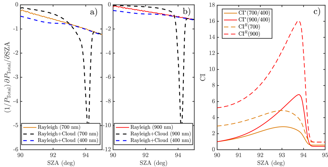
Figure 7. (a) Variation of \left(\frac{1}{P_{\text{Total}}(\lambda, \text{SZA})} \cdot \frac{\partial P_{\text{Total}}(\lambda, \text{SZA})}{\partial \text{SZA}}\right) with SZA for a purely Rayleigh atmosphere at 700 nm, and for an atmosphere including Rayleigh scattering and a cloud layer at 16 km (as in Fig. 5) at 400 and 700 nm. Panel (b) shows the same comparison as panel (a), but for 900 nm instead of 700 nm. Panel (c) compares \text{CI}^* and \text{CI}^R for the same cloud scenario as in panels (a) and (b). For \text{CI}^* , \lambda_1 = 400 nm and \lambda_2 = 700 and 900 nm are used, while \text{CI}^R is computed at \lambda = 700 and 900 nm.
