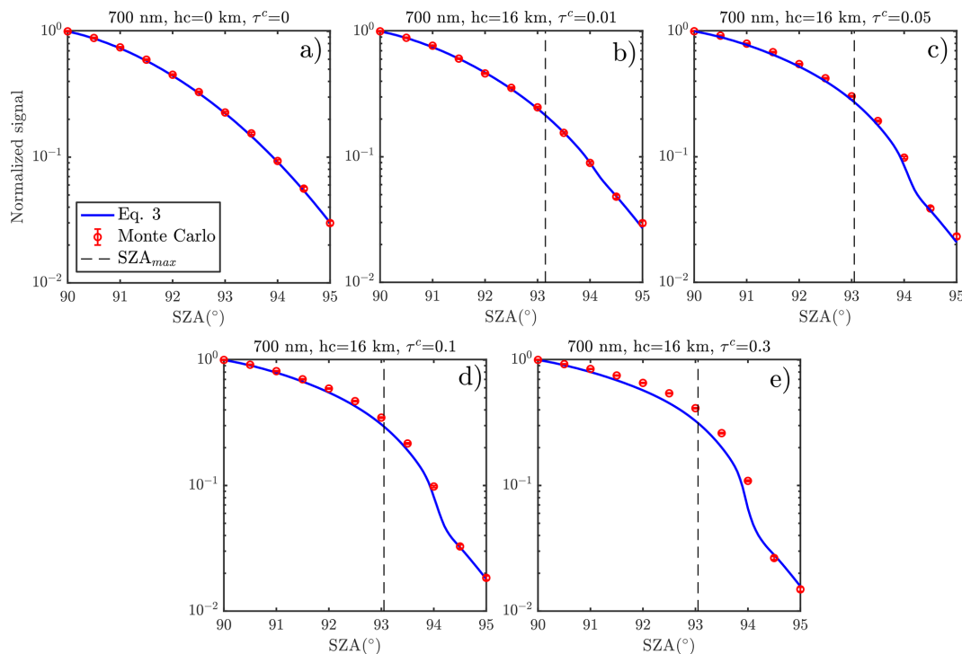
Figure 10. Same as in Fig. 8, but with the cloud height fixed at h_C = 16 km and the cloud optical depth varied as follows: \tau^c = 0 (a), 0.01 (b), 0.05 (c), 0.1 (d), and 0.3 (e). All other parameters are identical to those used in Fig. 8. No dashed line is shown in (a), since no cloud is present and therefore no SZA_{max} can be defined.
