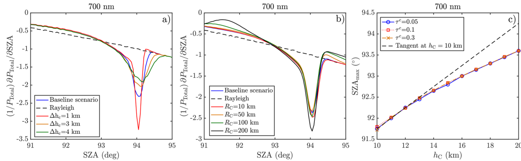
Figure 12. Sensitivity of SZA_{max} to cloud parameters: (a) variation with cloud geometrical thickness \Delta h_C , (b) variation with cloud horizontal scale R_C , and (c) relationship between cloud height and SZA_{max} for different cloud optical depths. The black dashed line in panel (c) represents the tangent to the \tau_C = 0.05 curve at h_C = 10 km.
