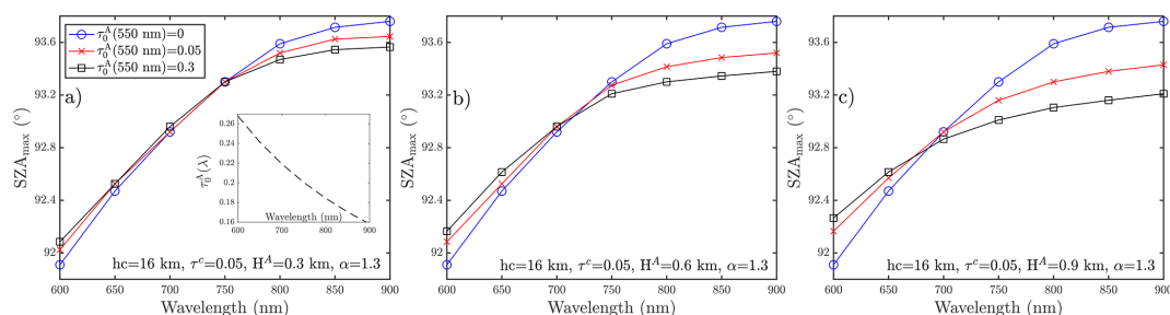
Figure 13. Variation of SZA_{max} with wavelength derived from CI^R for a cloud layer located at h_C = 16 km with optical depth \tau_C = 0.05 . Results are shown for different aerosol scenarios characterized by \tau_0^A(550 \text{ nm}) = 0 (blue line), 0.05 (red line), and 0.3 (black line), and for three aerosol scale heights: H^A = 0.3 km (a), 0.6 km (b), and 0.9 km (c). The spectral dependence of \tau_0^A is parameterized using an Ångström exponent \alpha = 1.3 , whose corresponding curve is shown in the inset of (a).
