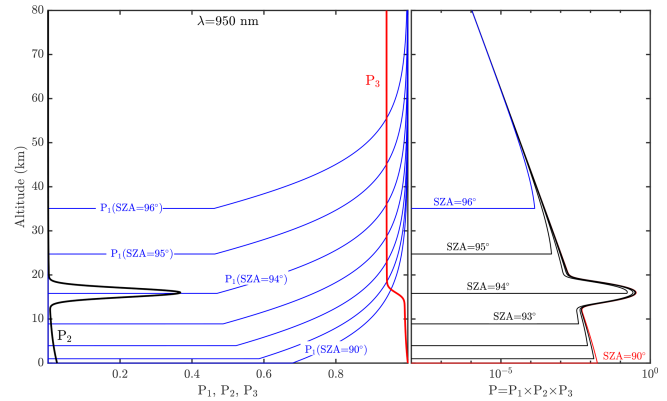
Figure 3. Same as Fig. 2, but at 950 nm.
