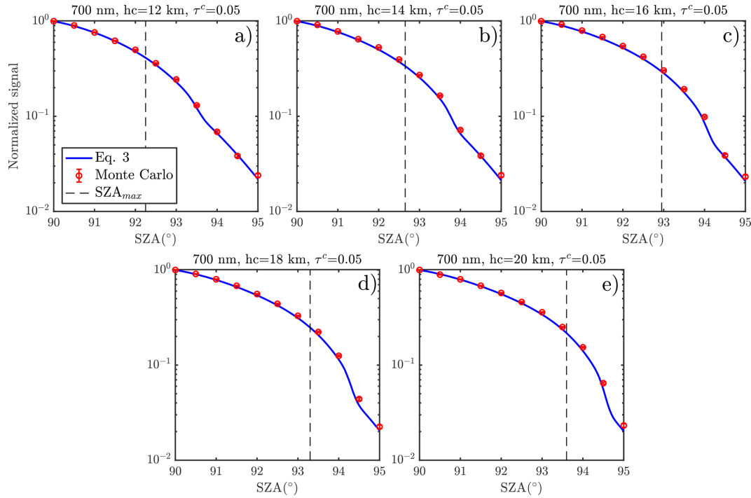
Figure 8. Normalized zenith intensity as a function of SZA for different cloud heights: h_C = 12 km (a), 14 km (b), 16 km (c), 18 km (d), and 20 km (e). All simulations were performed at 700 nm, with cloud optical thickness \tau_C = 0.05 , horizontal scale R_C = 20 km, and cloud geometrical thickness \Delta h_C = 2 km. Monte Carlo simulations are shown as red dots, while the single-scattering model is represented by the blue solid lines. The black dashed line indicates the value of SZA_{max} corresponding to each cloud scenario, assuming \lambda_1 = 400 nm.
