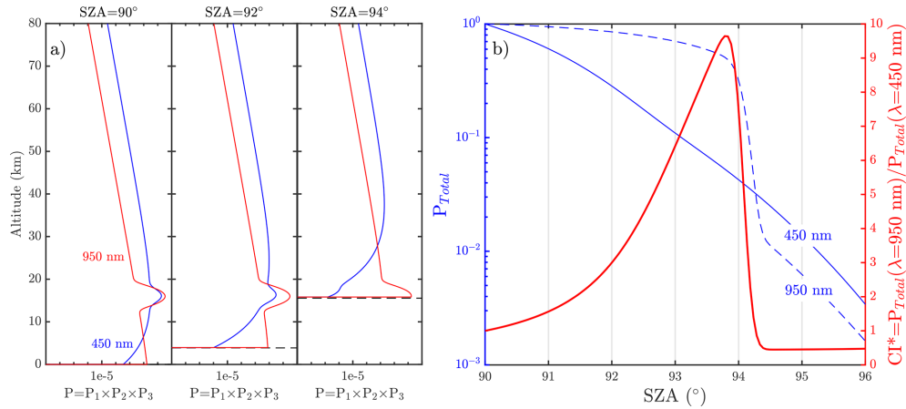
Figure 4. (a) Vertical profiles of P at 450 nm (blue lines) and 950 nm (red lines) for SZA = 90, 92, and 94°. The atmospheric scenario is the same as in Figs. 2 and 3. (b) Variation of P_{Total} at 450 nm (blue solid line) and 950 nm (blue dashed line) with SZA for the atmospheric conditions of Figs. 2 and 3. The red solid line represents CI^* obtained from P_{Total} at 450 and 950 nm.
