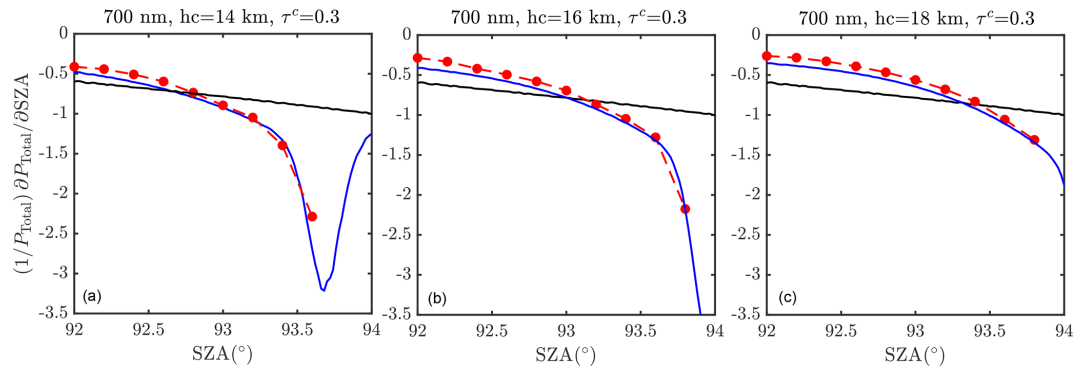
Figure 11. Comparison of the variation of \left(\frac{1}{P_{\text{Total}}(\lambda, \text{SZA})} \frac{\partial P_{\text{Total}}(\lambda, \text{SZA})}{\partial \text{SZA}}\right) with SZA computed using the Monte Carlo model (red dots) and the SSM (blue solid lines) at 700 nm, for a pure Rayleigh atmosphere (black line) and different cloud scenarios with \tau_C = 0.3 : h_C = 14 km (a), 16 km (b), and 18 km (c). All other parameters are identical to those used in Fig. 8.
