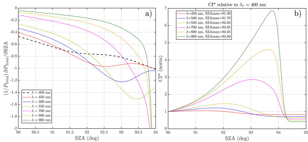
Figure 5. Variation of \left(\frac{1}{P_{Total}(\lambda, SZA)} \cdot \frac{\partial P_{Total}(\lambda, SZA)}{\partial SZA}\right) with SZA at 400, 450, 500, 550, 700, 800 and 900 nm for the atmospheric conditions of Figs. 2 and 3. Panel (b) shows the corresponding CI^* signals for the same atmospheric conditions as in panel (a), with \lambda_1 = 400 nm fixed and \lambda_2 = 450, 500, 550, 700, 800 , and 900 nm.
