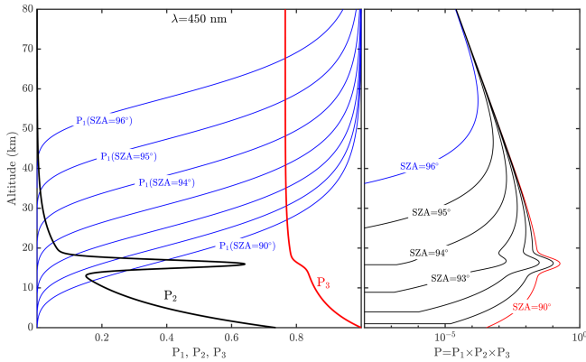
Figure 2. Variation of P_1 , P_2 , P_3 , and P with altitude at 450 nm for different SZAs (90, 91, 92, 93, 94, 95, and 96°), considering a cloud layer located at an altitude of 16 km, with a geometrical thickness of 2 km and a total optical depth of 0.05. The P_2 curves (left panel) were normalized by P_{\text{Total}} at \text{SZA} = 90^\circ .
