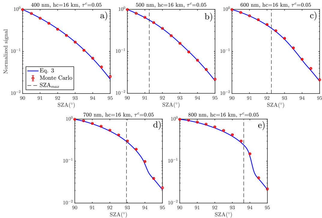
Figure 9. Similar simulations to those shown in Fig. 8, but keeping the cloud height fixed at h_C = 16 km and varying the wavelength: 400 nm (a), 500 nm (b), 600 nm (c), 700 nm (d), and 800 nm (e). The remaining parameters are kept identical to those in Fig. 8. No dashed line is shown in (a), since \lambda_1 = \lambda_2 = 400 nm and therefore SZA_{max} is not defined.
