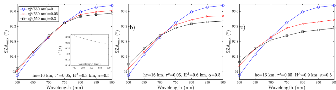
Figure 14. Same as in Fig. 13, but with an Ångström exponent \alpha = 0.5 .
