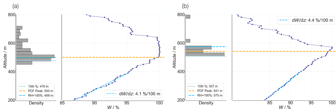
Figure 3. First ceilometer cloud returns for 30 min before and after the radiosonde launch time (grey histograms) and the relative humidity profiles measured by the radiosondes (blue profiles, data every 10 m). Also shown on the ceilometer cloud base height histograms are the 10th percentile (solid light blue line), the first major peak of the distribution calculated from a Gaussian kernel density estimate (orange dashed line), and the height at which relative humidity would reach 100 % when extrapolating from a linear regression fit to the observed profile from 200–400 m (turquoise dashed line), as described in the text. Panel (a) is around the radiosonde launched on 29 January 2020 at 06:44 UTC (02:44 a.m. local Barbados time) and panel (b) is 1 February 2020 at 00:25 UTC (08:25 p.m. local Barbados time). These are two cases where radiosonde relative humidity reached 100 % below 1000 m.
