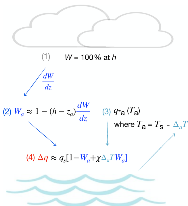
Figure 2. Schematic overview of the methodology highlighting the main error sources: (1) estimating cloud base height, h , at which W = 100\% is assumed and then extrapolating W downward to z_a using (2) a fixed relative humidity lapse rate \frac{dW}{dz} , which is then converted to q_a as described in the text with a fixed \Delta_a T = 1.0\text{ K} .
