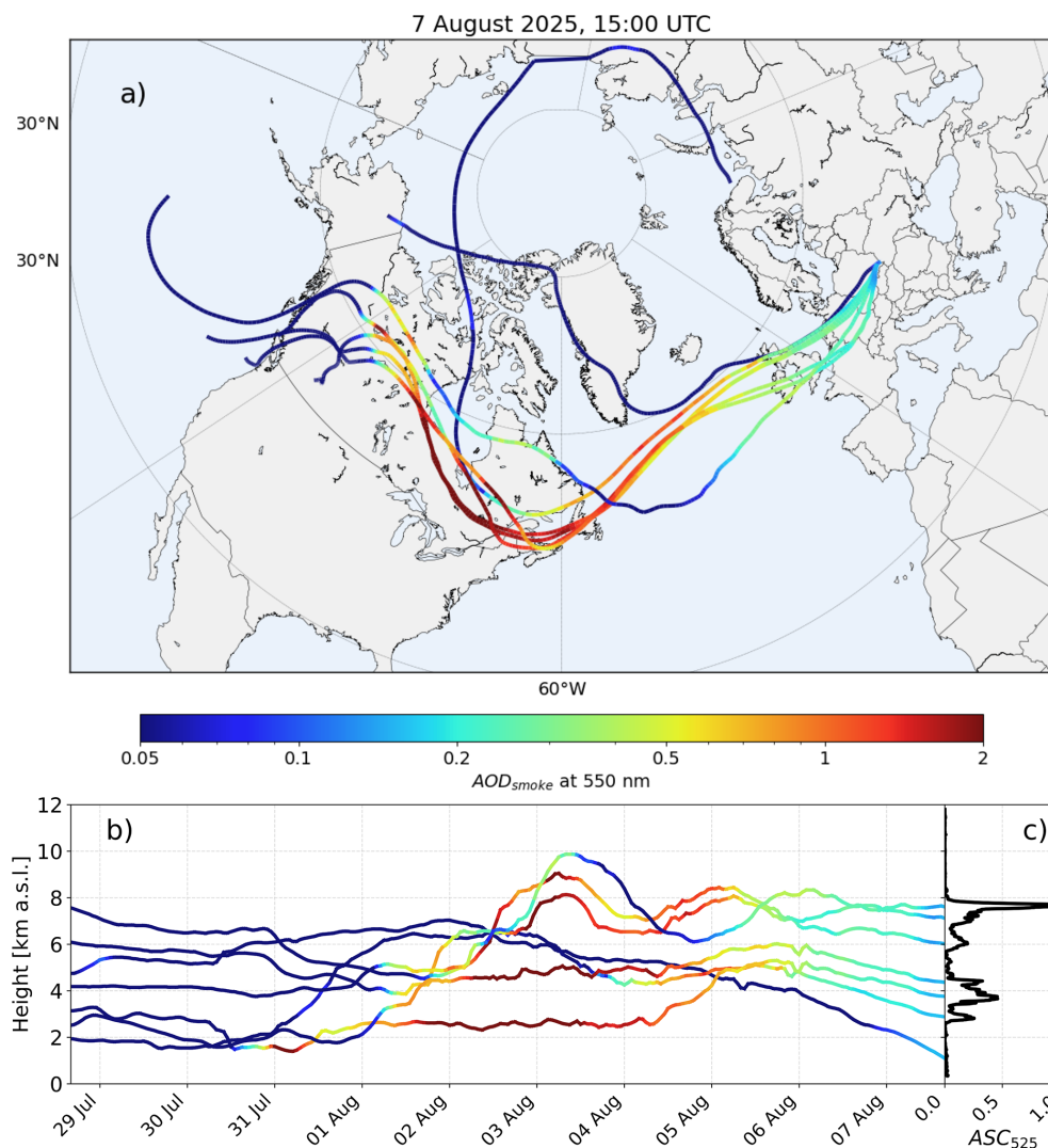
Figure 6. LAGRANTO 10 d backtrajectories starting on 7 August 2025 at 15:00 UTC. Panels (a) and (b) show the geographical distribution and the vertical cross-section of the selected trajectories, respectively. Line colours represent ICAP AOD smoke at 550 nm. Panel (c) shows the normalised profile of ASC 525 measured by the AeroSonde.
