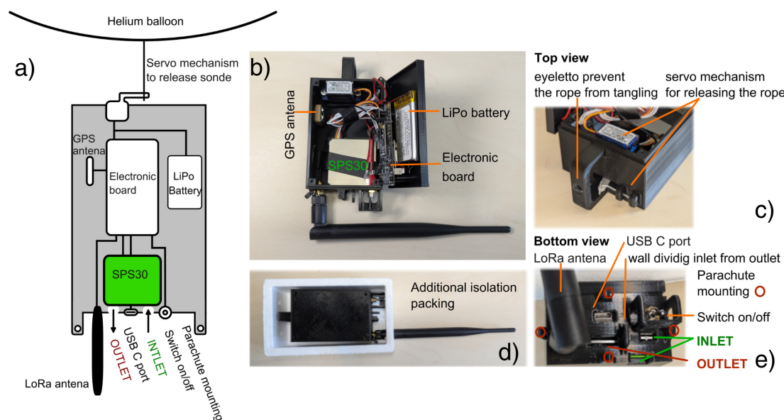
Figure 1. Diagram of the AeroSonde construction showing labeled main components (a) and AeroSonde setup shown from multiple angles (b–e).
