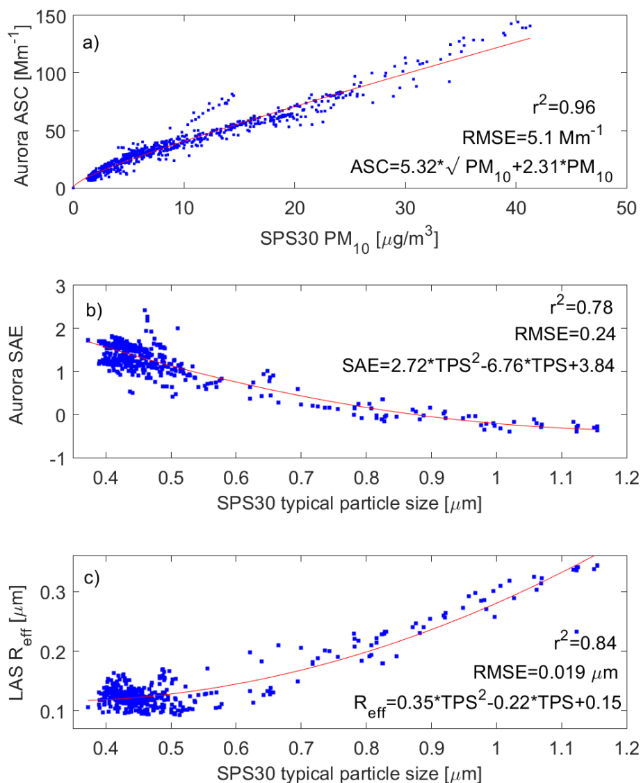
Figure 2. Scatter plot and regression fit (red lines) of the 1 h mean (a) the \text{PM}_{10} from SPS30 and ASC at 525 nm from Aurora 4000, (b) SPS30 typical particle size [ \mu\text{m} ] and SAE from Aurora 4000, and (c) SPS30 typical particle size and effective radius from LAS 3340, both in [ \mu\text{m} ]. Data from five SPS30 sensors are averaged and visible as one point.
