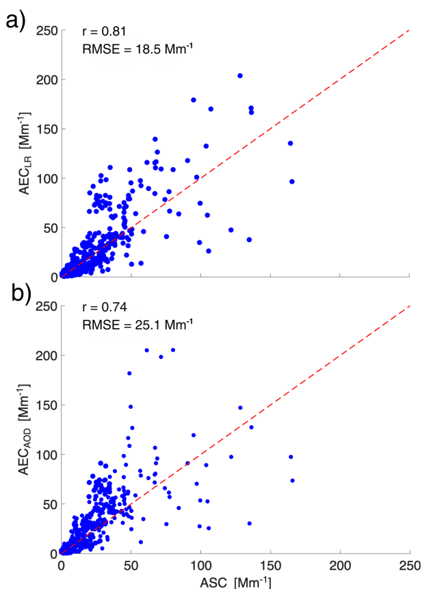
Figure 4. Scatter plots of aerosol optical coefficients averaged within 100 m vertical intervals. The x axis shows the ASC at 525 nm retrieved from AeroSonde measurements, while the y axis presents the AEC at 532 nm derived from lidar observations. Panel (a) displays AEC retrieved using the Klett LR approach ( AEC_{LR} ), and panel (b) shows AEC from Klett AOD ( AEC_{AOD} ). For each panel, the Pearson correlation coefficient ( r ) and the root mean square error (RMSE) are reported.
