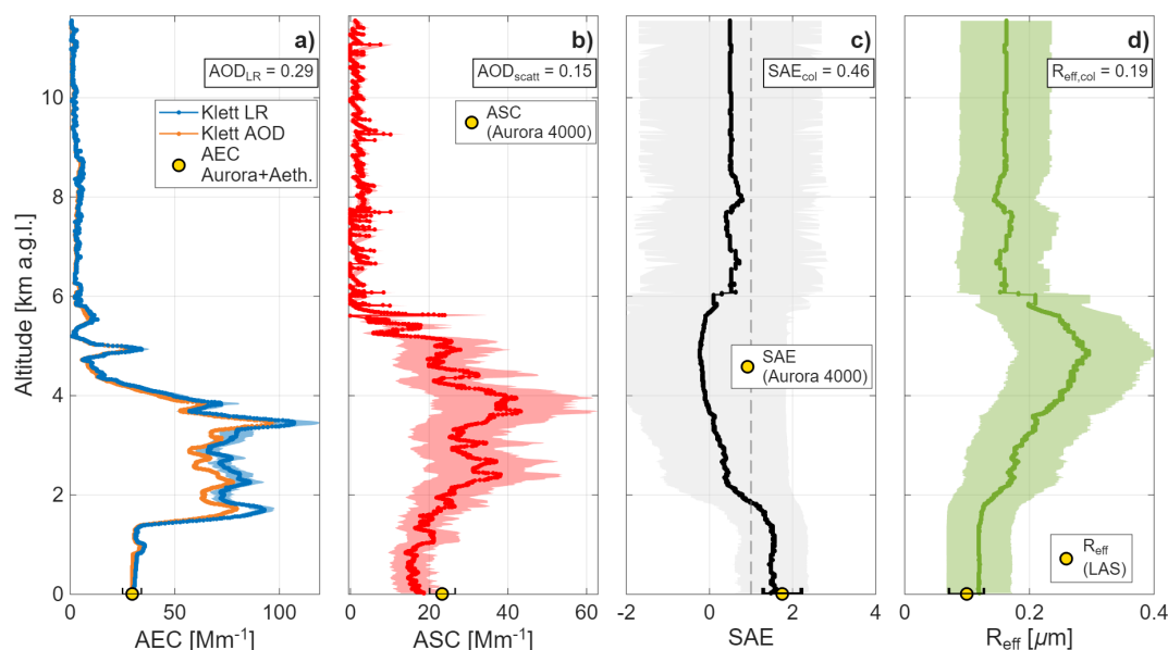
Figure 11. Results of the measurements on 29 August 2025, 15:20–16:30 UTC. Same variables as in Fig. 8.
