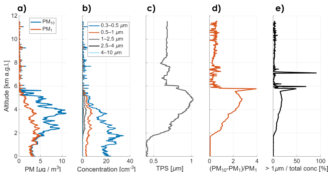
Figure 10. Vertical profiles of raw data obtained by AeroSonde during measurements on 29 August 2025, 15:20–16:30 UTC. Same variables as in Fig. 7
