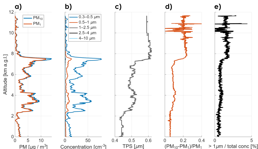
Figure 7. Vertical profiles of raw data obtained by AeroSonde during measurements on 7 August 2025, 15:20–16:30 UTC. Panel (a) shows mass concentrations of \text{PM}_{10} and \text{PM}_1 . Panel (b) presents particle number concentrations for selected size ranges (0.3–0.5, 0.5–1, 1–2.5, 2.5–4, and 4–10 \mu\text{m} ). Panel (c) shows the typical particles size parameter (TPS). Panel (d) displays the coarse-to-fine mass ratio expressed as (\text{PM}_{10} - \text{PM}_1) / \text{PM}_1 . Panel (e) presents the contribution of particles larger than 1 \mu\text{m} to the total number concentration.
