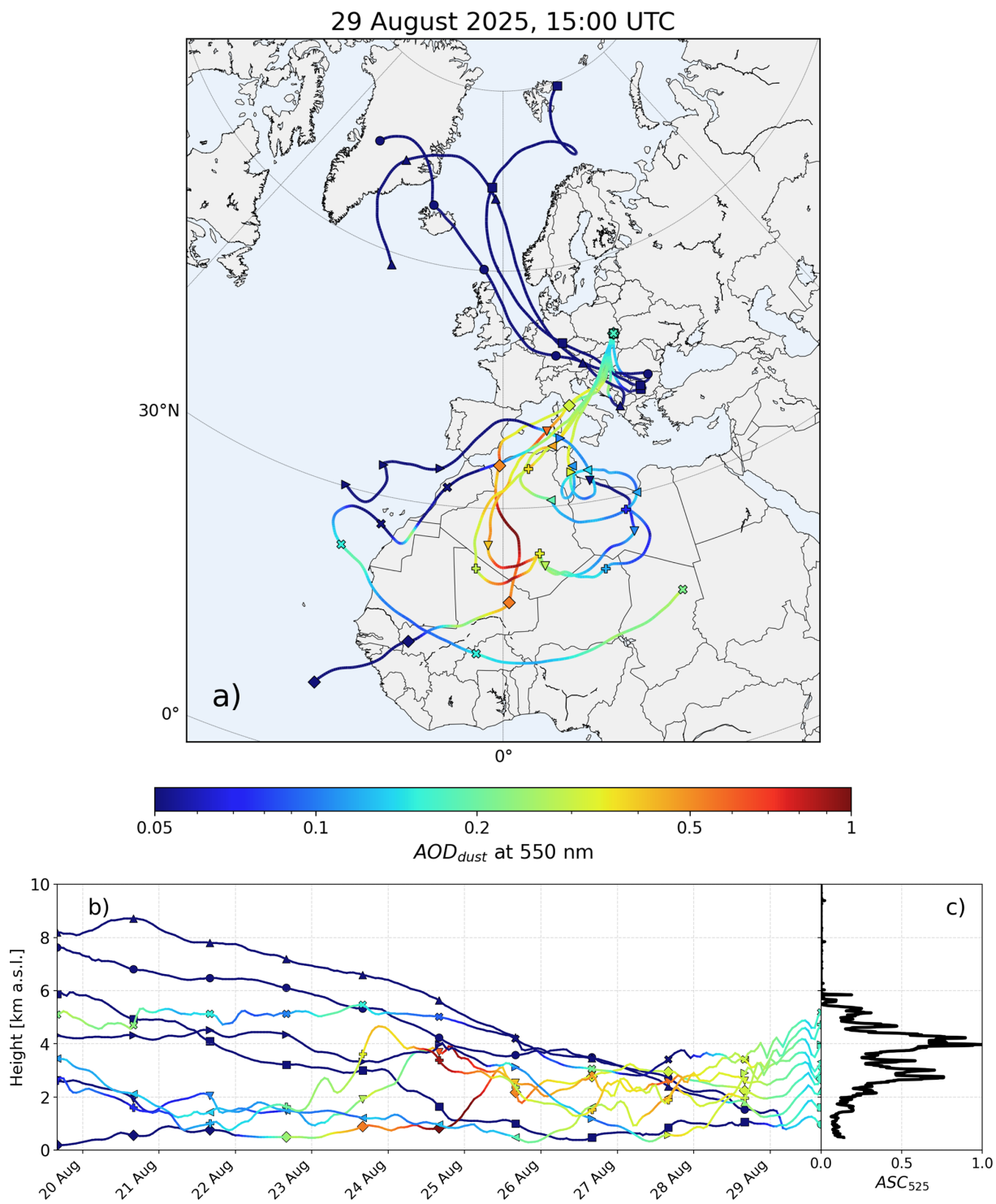
Figure 9. LAGRANTO 10 d backtrajectories starting on 29 August 2025 at 15:00 UTC. Panels (a) and (b) show the geographical distribution and the vertical cross-section of the selected trajectories, respectively. Line colours represent ICAP AOD_{dust} at 550 nm, and, for clarity, each trajectory is marked with distinct symbols. Panel (c) shows the normalised profile of ASC_{525} measured by the AeroSonde.
