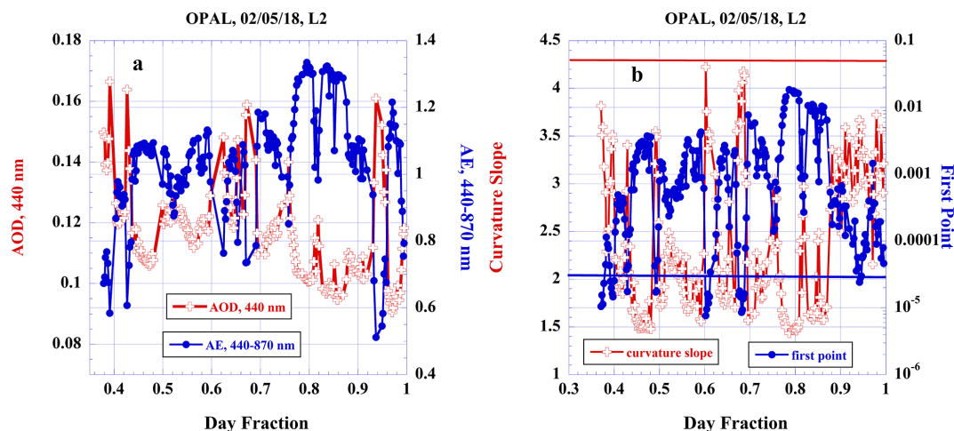
Figure 3. Temporal dependence of level 2 AOD measured at OPAL AERONET site on 2 May 2018 (a), slope of the curvature and the first point of curvature calculated from CCS (3.3) measurements (b).
