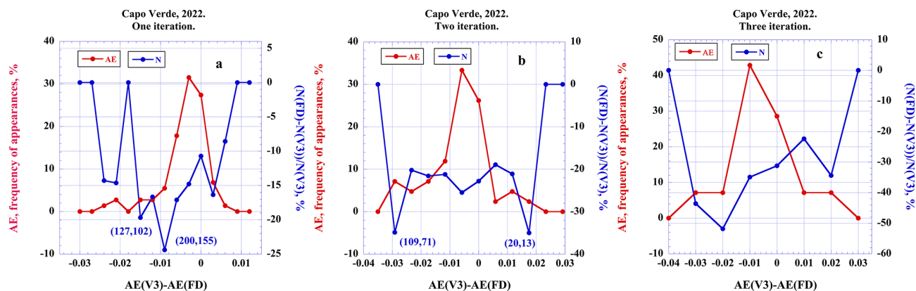
Figure 15. Histograms of the difference between AE corresponding to V3 L1.5 and AE after the first iteration of FD algorithm (red line) as well as relative difference in the number of AOD observations (blue line). Capo Verde AERONET site for the entire year of 2022: (a) after one iteration, (b) after two iterations, (c) after three iterations. The first number in the ordered pair in parentheses is the number of AOD measurements before the iteration and the second number is the one after.
