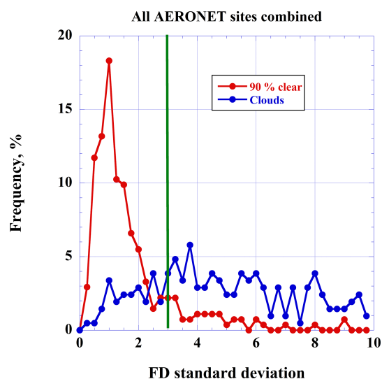
Figure 22. Distribution of FD standard deviation for 90 % clear (red line) and cloudy (blue line) conditions. Vertical line shows selected value for the threshold.
