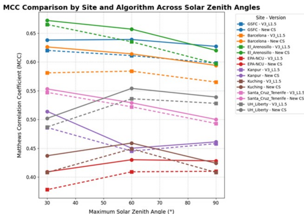
Figure 23. Dependence of Matthews correlation coefficient (MCC) on the maximum solar zenith angle for V3 Level 1.5 cloud screened data and data additionally screened FD algorithm abbreviated here as New CS.
