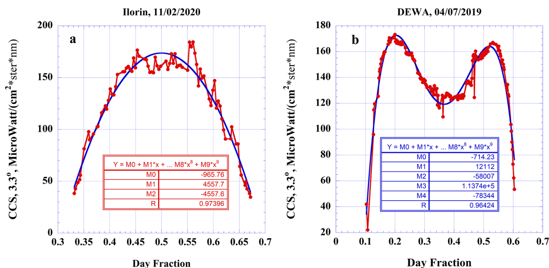
Figure 4. Temporal dependence of CCS (3.3) measured at (a) Ilorin AERONET site on 11 February 2020, (b) DEWA AERONET site on 4 July 2019.
