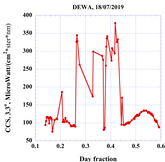
Figure 5. Temporal dependence of CCS (3.3) measured at DEWA AERONET site on 18 July 2019.
