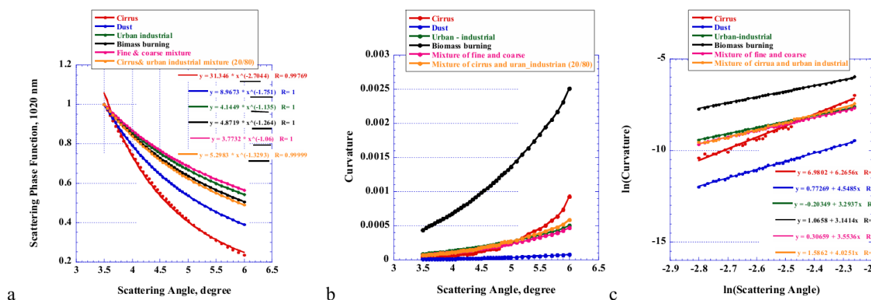
Figure 1. Scattering phase function calculated for different atmospheric particulates. Solid lines represent power law fit (a), Dependence of the curvature on the scattering angle in aureole calculated for three typical fine and coarse mode dominated aerosols, fine-coarse aerosols and aerosol-cirrus mixtures (b), Slope of the curvature in aureole estimated for three typical fine and coarse mode dominated aerosols, fine-coarse aerosols and aerosol-cirrus clouds mixtures (c).
