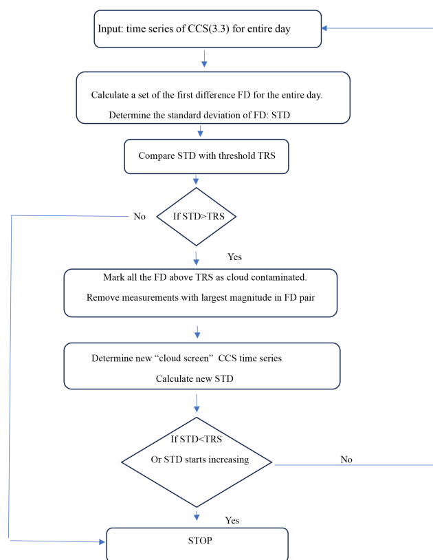
Figure 6. Flow chart of FD algorithm.
