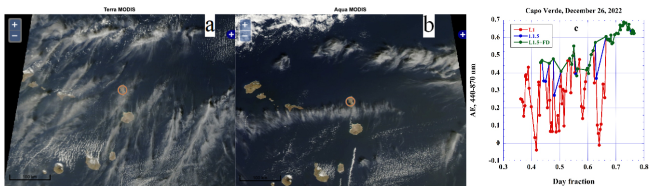
Figure 20. Terra MODIS image of the area in vicinity of the Capo Verde AERONET site on 26 December 2022: Terra (a), Aqua (b), time series of AE, red, blue and green lines depict L1, L1.5 and L1.5 after application of the FD algorithm respectively.
