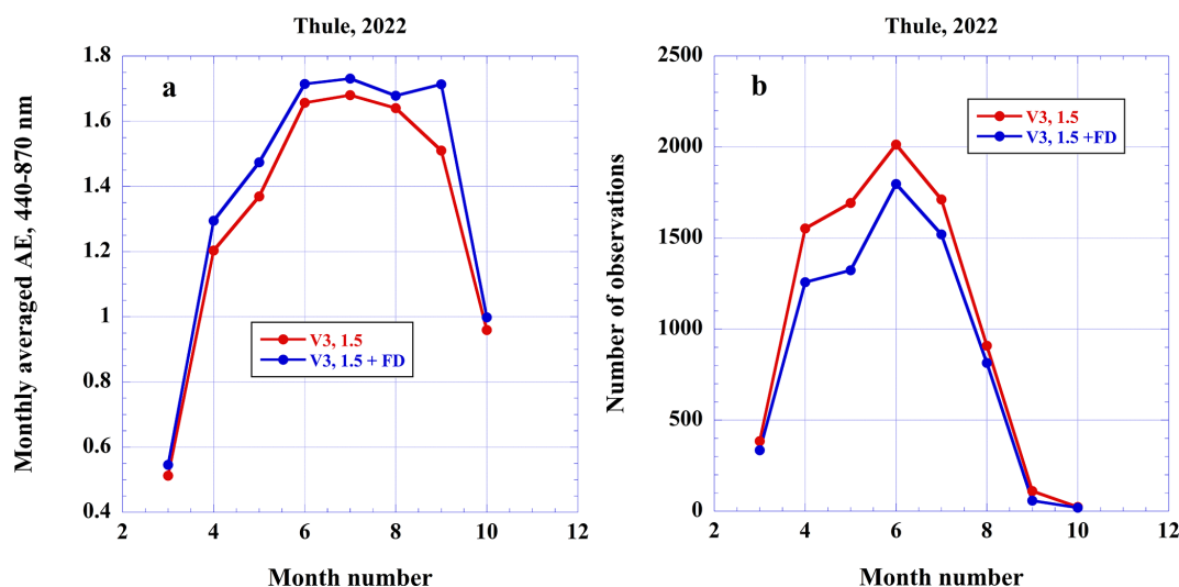
Figure 10. Monthly averaged AE as function of month for Thule AERONET site. Red line corresponds to V3 level 1.5 and blue line after FD algorithm was applied; (a) monthly averaged AE, (b) number of observations.
