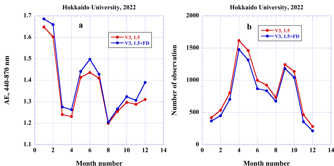
Figure 12. Monthly averaged AE as function of month for Hokkaido University AERONET site. Red line corresponds to V3 level 1.5 and blue line after FD algorithm was applied: (a) monthly averaged AE (440–870), (b) number of observations.
