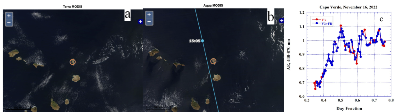
Figure 21. MODIS images of the area in vicinity of the Capo Verde AERONET site on 16 November 2022: Terra (a), Aqua (b), time series of AE, red and blue lines depict V3 and V3 after application of the FD algorithm respectively. On the Aqua image, blue line shows the Aqua MODIS satellite track.
