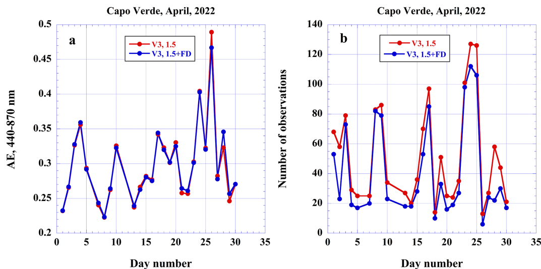
Figure 14. Daily averaged AE as function of day number for Capo Verde AERONET site in April 2022. Red line corresponds to V3 level 1.5 and blue line after FD algorithm was applied: (a) daily AE (440–870), (b) number of observations.
