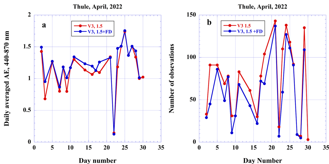
Figure 11. Daily averaged AE as function of day number for Thule AERONET site in April 2022. Red line corresponds to V3 level 1.5 and blue line after FD algorithm was applied; (a) daily averaged AE, (b) number of observations.
