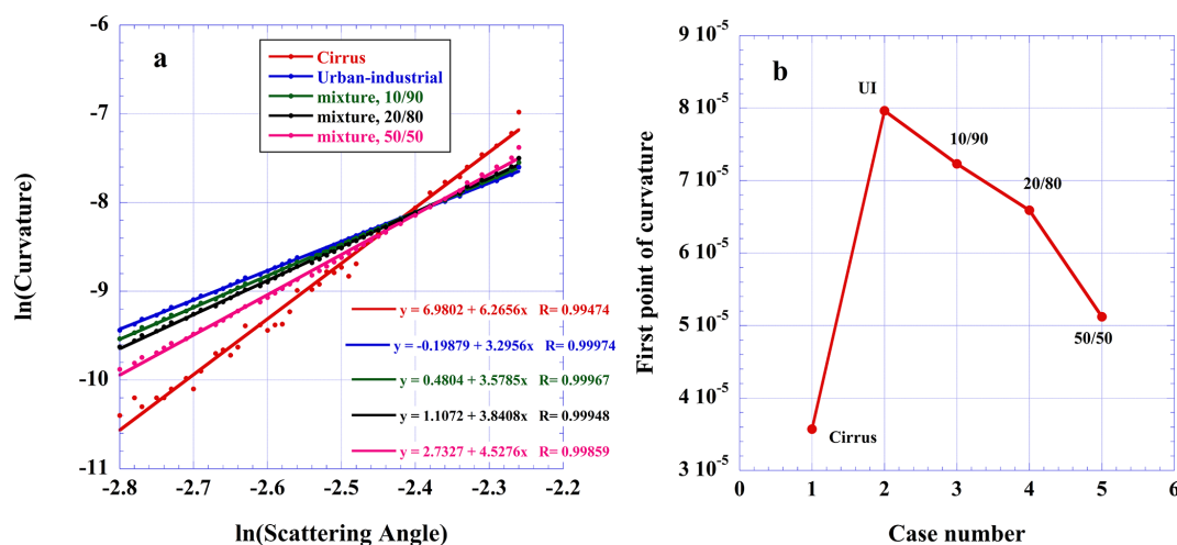
Figure 2. Dependence of the curvature slope on the cloud fraction for the three mixtures of urban industrial aerosol with cirrus clouds, (cirrus clouds/aerosols): 10/90, 20/80, and 50/50 (a), dependence of the first point of the curvature on case number, each case corresponding to the different cloud fraction for the mixture of urban-industrial aerosols with cirrus clouds (b).
