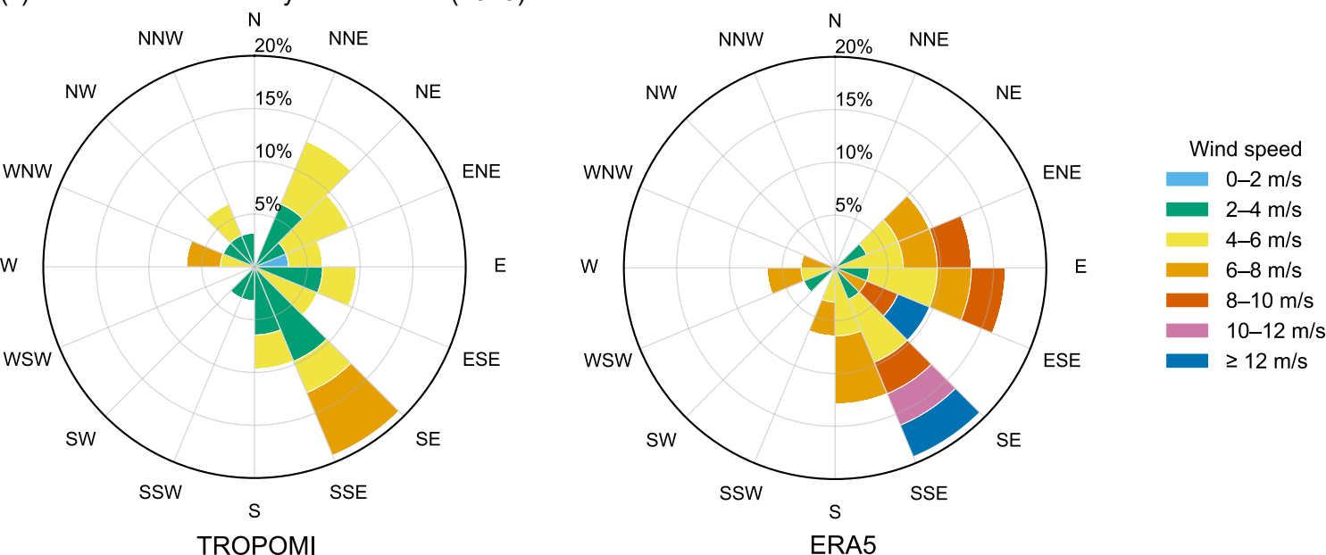
(c) Wind roses for the city of New York (2023)
