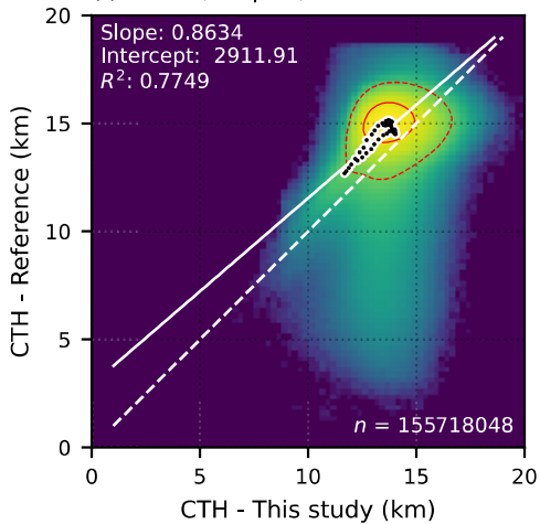
(f) SEVIRI, Tropics, 2004-2024
