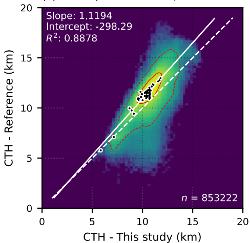
(e) SEVIRI, Tropics, 2007
