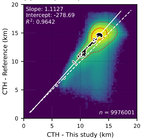
(c) SEVIRI, Mid-latitudes, 2007
