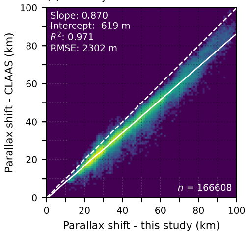
(c) Bias-adjusted to CALIPSO
