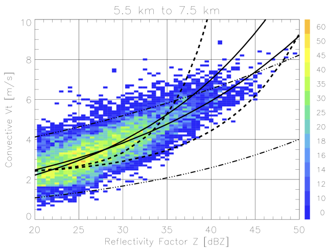
Figure 4. Cumulative histograms for profiler fall speed V_t (adjusted to sea level) versus radar reflectivity factor Z for “convective” media for heights between 5.5 km and 7.5 km a.g.l. Solid lines are the matched profiler behaviors for fits having a coefficients = [1.0, 0.71] and b coefficients = [0.19, 0.25]. Dashed lines are “graupel” fall speed curves from Giangrande et al. (2013, 2016a). Dashed-dotted lines follow previous fall speed relationships for rain and snow.
