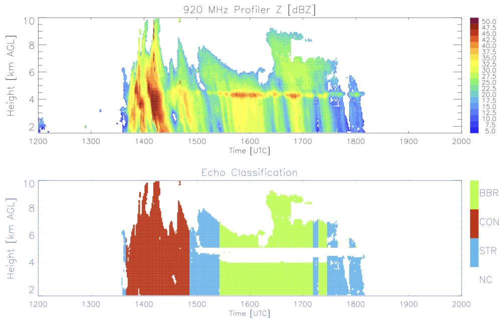
Figure 1. An example of Darwin 920 MHz Profiler radar reflectivity factor Z (top) and an associated convective rain (“CON”), stratiform rain (“STR”) and “bright band” stratiform rain (“BBR”) echo classifications for an event on 17 November 2005.
