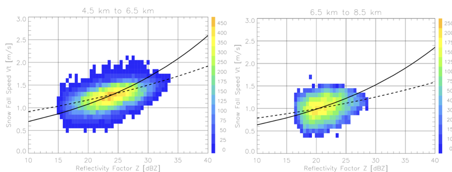
Figure 3. Cumulative histograms for Darwin profiler fall speed V_t (adjusted to sea level) versus radar reflectivity factor Z for snow above bright band signatures, for heights between 4.5 km and 6.5 km a.g.l. (left panel), and 6.5 km and 8.5 km a.g.l. (right panel). The solid line represents the fall speed relationship coefficient a = 0.45 (left panel) and 0.41 (right panel) for a fixed b coefficient of 0.19 . The dashed lines represent our dataset best-fit a = 0.72 (left panel) and 0.62 (right panel) for a fixed b = 0.1 .
