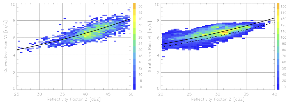
Figure 2. Cumulative histograms for fall speed V_t (adjusted to sea level) versus radar reflectivity factor Z for “convective” rain (left) and “stratiform” rain (right) collected by the Darwin profiler at altitudes below 2.5 km. Solid lines represent the best-fit fall speed relationship having an “ a ” coefficient of 2.59 (convective, left) and 3.3 (stratiform, right) for a fixed b coefficient of 0.1. The dashed line on the stratiform plot represents a disdrometer-based fall speed relationship having an a coefficient of 3.1.
