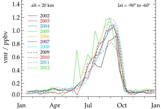
(b) ClO, V8H+V8R, day
