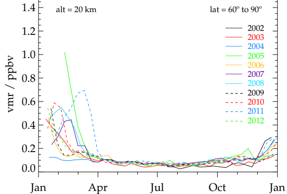
(a) ClO, V8H+V8R, day
