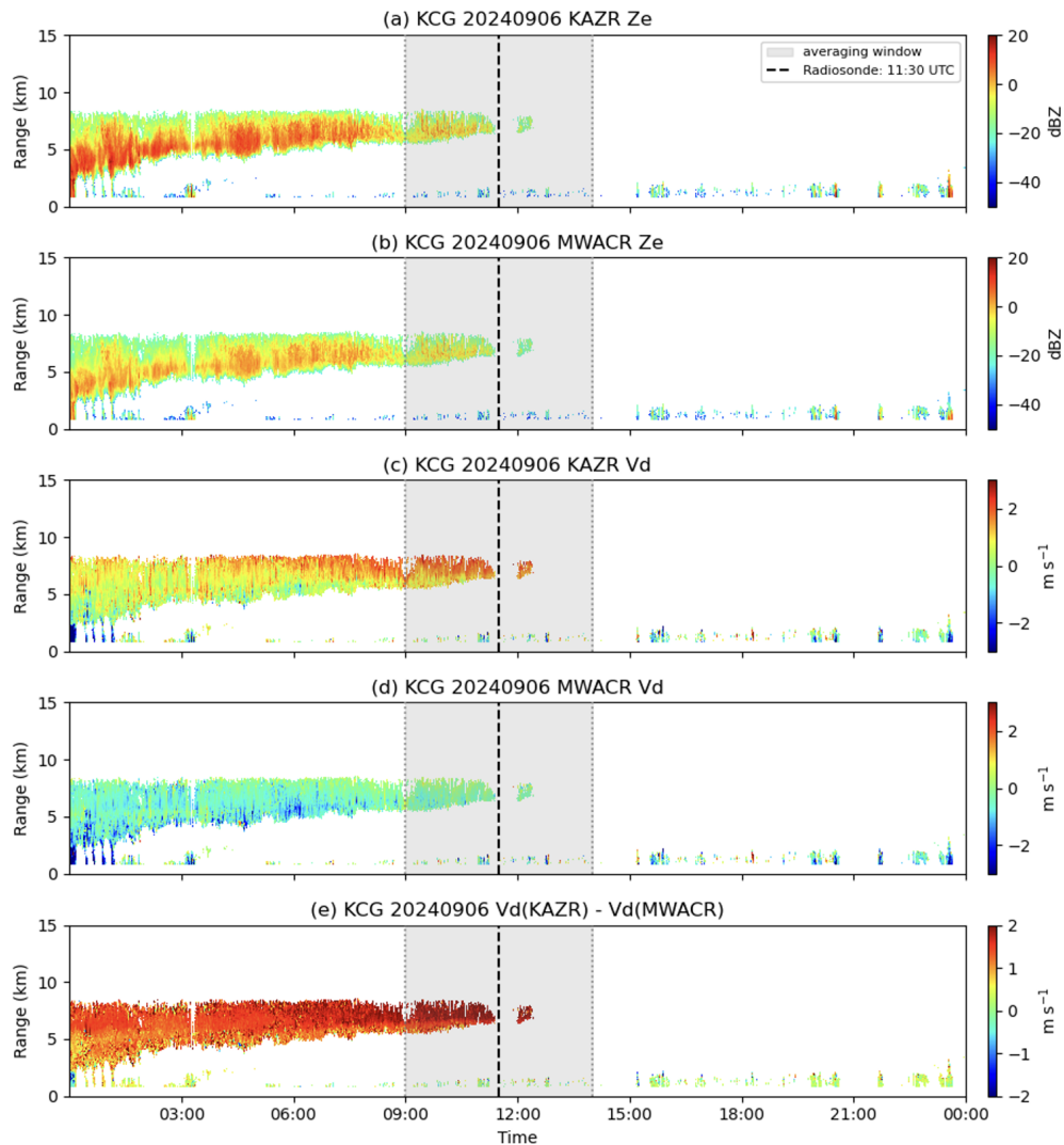
Figure 1. Time–height cross sections of radar reflectivity ( Z_e ) and Doppler velocity ( V_d ) observed by KAZR and MWACR at the CAPE-k site (KCG) on 6 September 2024. Panels show (a) KAZR reflectivity, (b) MWACR reflectivity, (c) KAZR Doppler velocity, (d) MWACR Doppler velocity, and (e) Doppler velocity difference V_d(\text{KAZR}) - V_d(\text{MWACR}) . The collocated radiosonde launch at 11:30 UTC is denoted by a dashed line, and the shaded regions indicate the 150 min radar-averaging window.
