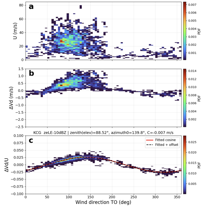
Figure 8. Same as Figs. 6 and 7, but for the difference in Doppler velocity ( \Delta V_d ) between KAZR and MWACR.
