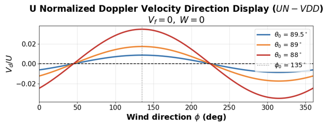
Figure 4. U -normalized velocity–direction displays (UN-VDDs) derived from the simulations in Fig. 3 for \theta_0 = 89.5 , 89, and 88^\circ .
