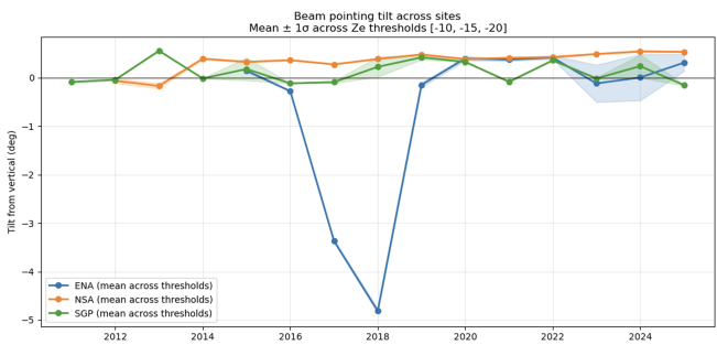
Figure 10. Time series of the mean KAZR beam-pointing tilt from vertical at the ENA, NSA, and SGP sites during 2011–2025. Tilt estimates are derived using multiple radar reflectivity ( Z_e ) thresholds (−10, −15, and −20 dBZ) to filter the observations used in the pointing estimation. Shaded regions represent the standard deviation of the tilt estimates obtained using the different Z_e thresholds, indicating the sensitivity of the retrieval to reflectivity-based data selection. The results show generally stable pointing within approximately 0.5° at NSA and SGP over the analysis period, while a larger deviation is evident at ENA during 2017–2018.
