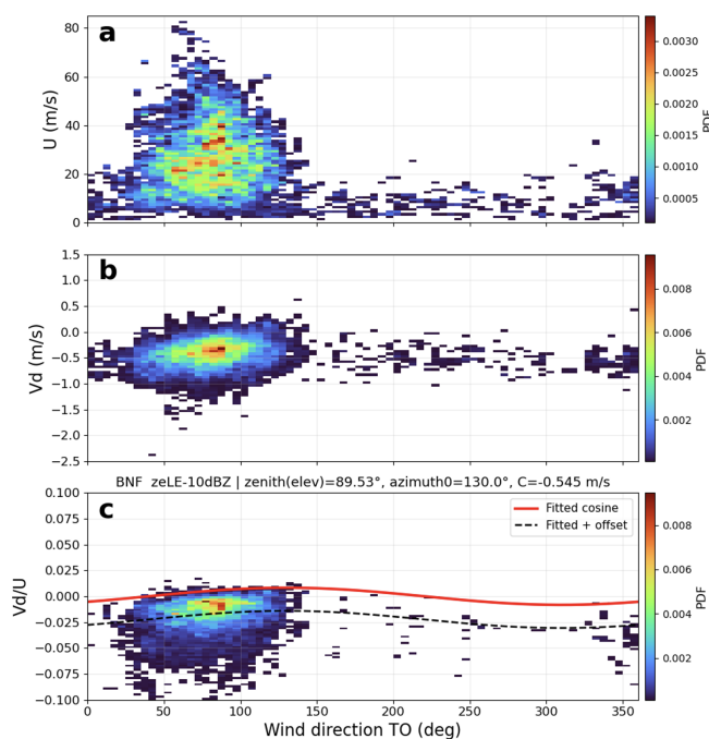
Figure 9. Same as Fig. 6, but for KAZR at BNF.
