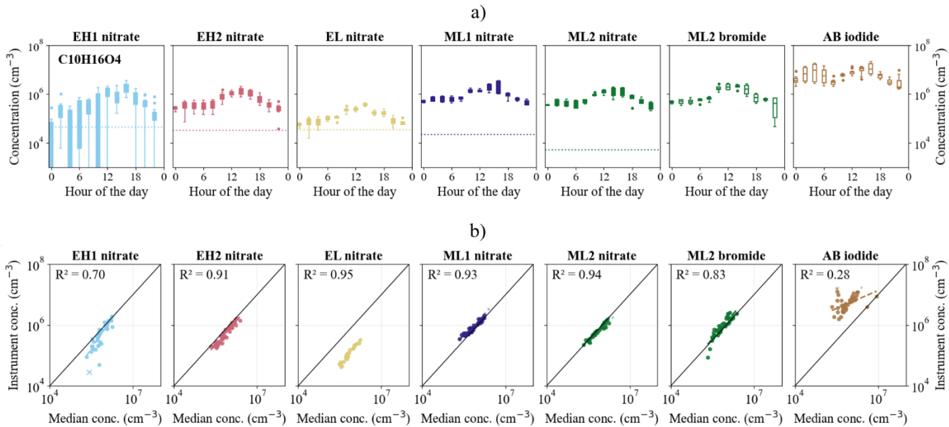
230 Figure S7 (a) Box plots showing the diurnal variation of C_{10}H_{16}O_4 based on measurements conducted on 1-2 August 2024. Data are from five instruments operating in nitrate mode (EH1, EH2, EL, ML1, ML2), one instrument operating in bromide mode (ML2), and one instrument operating in iodide mode (AB). Boxes indicate the interquartile range, whiskers represent the non-outlier range, and full circles denote outliers. For the instruments operating in nitrate mode, instrument-specific LOD_{CIMS} values are indicated by dotted horizontal lines. 235 (b) Scatter plots of hourly median concentrations showing, for each instrument and ionization mode combination, the concentrations measured by the individual instrument-mode against the median concentration measured across all instruments-mode combinations over the same period. Dashed lines indicate linear regressions for each instrument, with the corresponding coefficient of determination ( R^2 ) reported in the figure.
