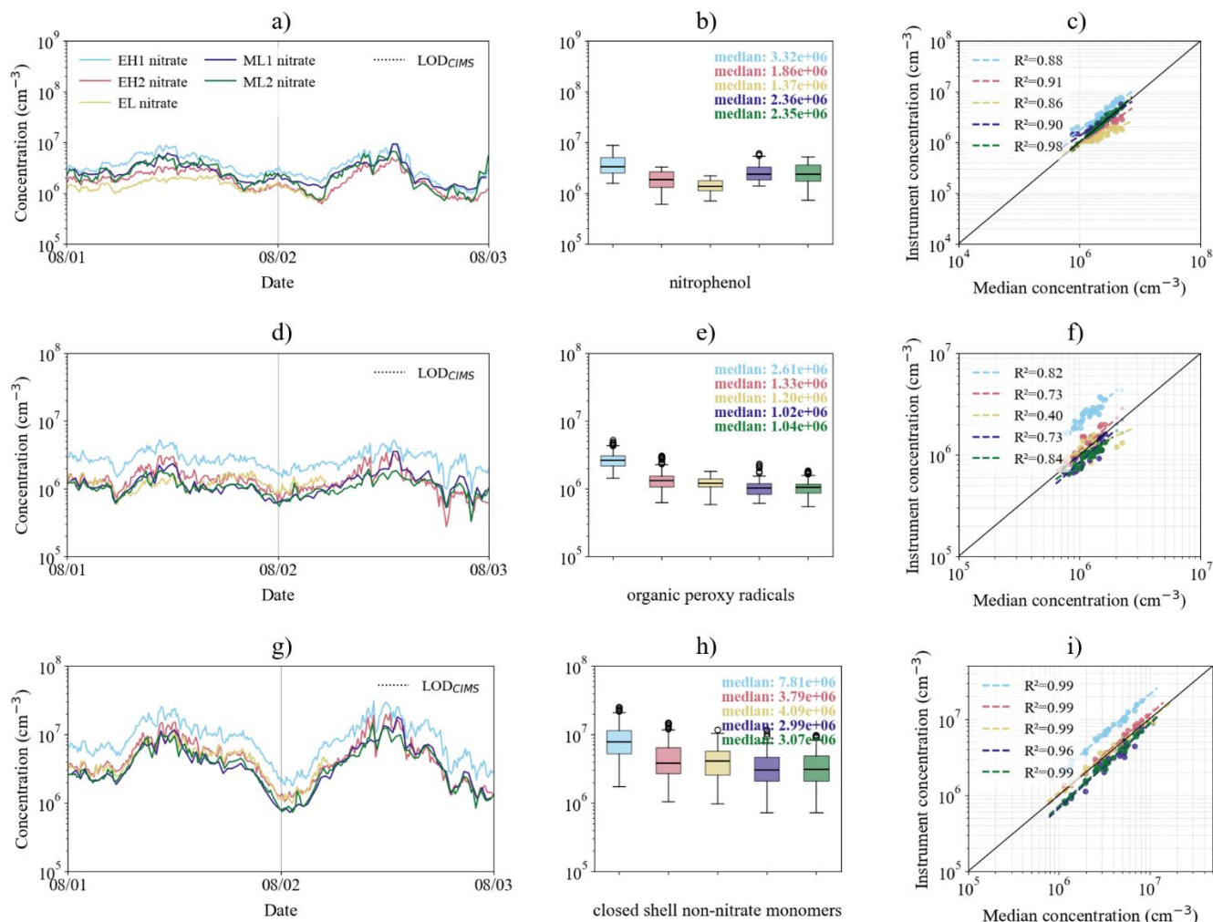
170 Figure S5 Concentrations of (top panel) nitrophenol, (central panel) organic peroxy radicals, and (bottom panel) closed-shell non-nitrate monomers measured in nitrate mode by five CI-API-ToFs during 1-2 August 2024. For each panel, the left figure ((a), (d), and (g)) shows concentration time series, with instrument-specific LOD_{CIMS} values indicated by dotted horizontal lines. The central figure ((b), (e), and (h)) shows a box plot summarizing the distributions over the same period; boxes indicate the interquartile range, horizontal lines indicate the 175 median, whiskers represent the non-outlier range, and empty circles denote outliers. Data points below LOD_{CIMS} are excluded from the box plot. The right figure ((c), (f), and (i)) shows the hourly median concentration measured by each instrument against the median of the hourly median concentrations across all five instruments. Dashed lines indicate log-log linear regressions for each instrument, with the corresponding coefficient of determination ( R^2 ) reported in the legend. Points below the corresponding LOD_{CIMS} are shown as crosses (X), while outliers are plotted as smaller semi-transparent points; both are excluded from the linear fits.
