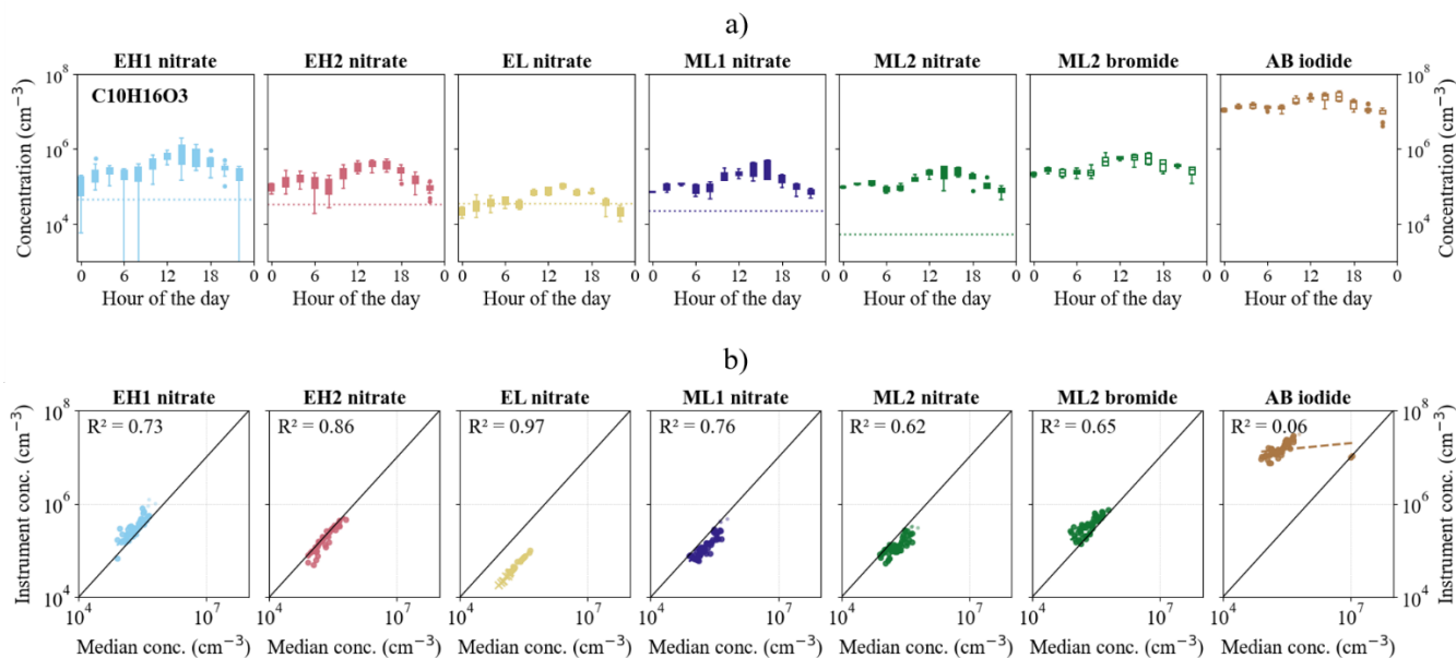
240 Figure S8 (a) Box plots showing the diurnal variation of C_{10}H_{16}O_3 based on measurements conducted on 1-2 August 2024. Data are from five instruments operating in nitrate mode (EH1, EH2, EL, ML1, ML2), one instrument operating in bromide mode (ML2), and one instrument operating in iodide mode (AB). Boxes indicate the interquartile range, whiskers represent the non-outlier range, and full circles denote outliers. For the instruments operating in nitrate mode, instrument-specific LOD_{CIMS} values are indicated by dotted horizontal lines. 245 (b) Scatter plots of hourly median concentrations showing, for each instrument and ionization mode combination, the concentrations measured by the individual instrument-mode against the median concentration measured across all instruments-mode combinations over the same period. Dashed lines indicate linear regressions for each instrument, with the corresponding coefficient of determination ( R^2 ) reported in the figure.
