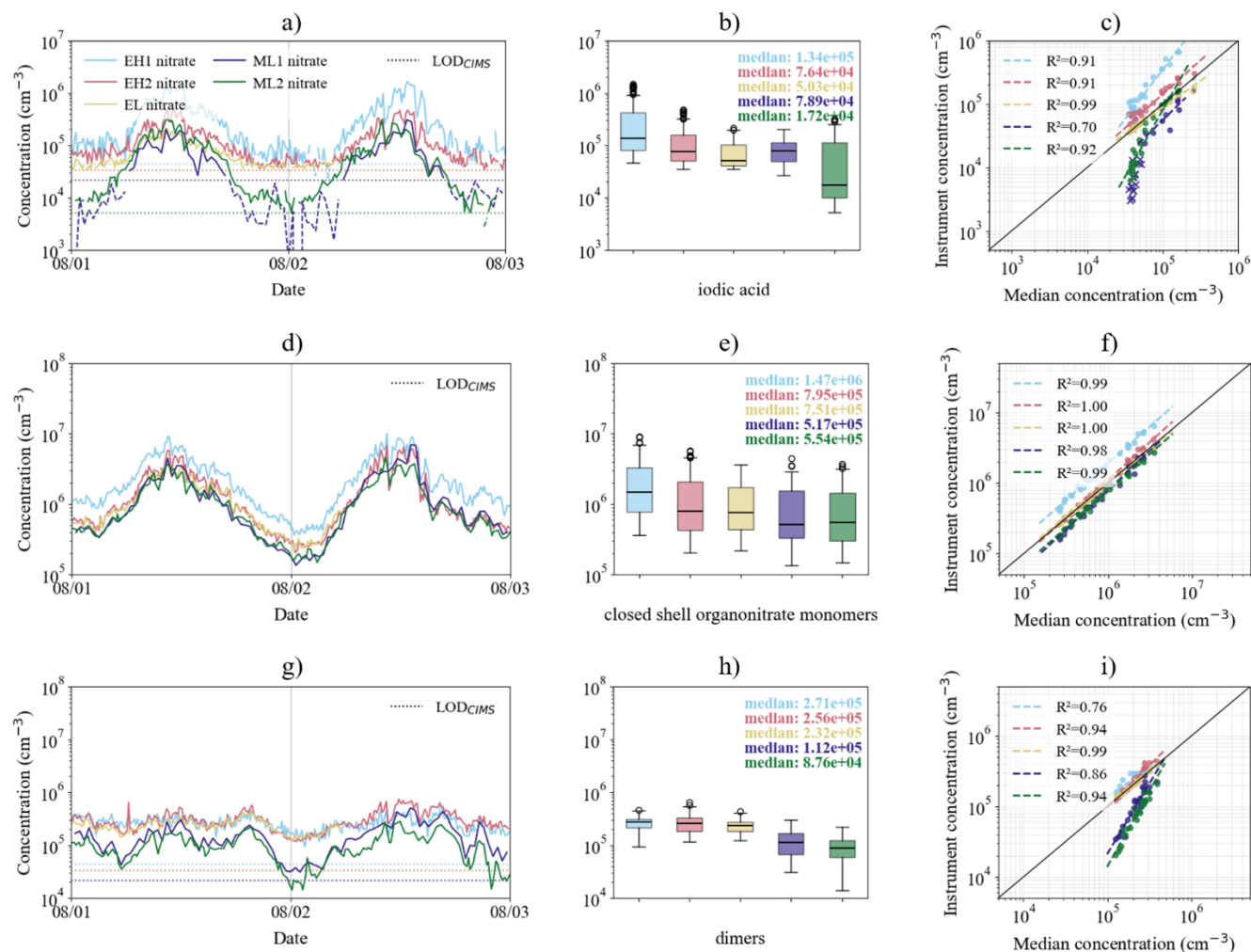
Figure 5. Concentrations of (a–c) iodic acid, (d–f) closed shell organonitrate monomers, and (g–i) dimers measured in nitrate mode by five CI-API-ToFs during 1–2 August 2024. For each panel, the left panels (a, d, g) show concentration time series, with instrument-specific \text{LOD}_{\text{CIMS}} values indicated by dotted horizontal lines. The central panels (b, e, h) show a box plot summarizing the distributions over the same period; boxes indicate the interquartile range, horizontal lines indicate the median, whiskers represent the non-outlier range, and empty circles denote outliers. Data points below \text{LOD}_{\text{CIMS}} are excluded from the box plot. The right panels (c, f, i) show the hourly median concentration measured by each instrument against the median of the hourly median concentrations across all five instruments. Dashed lines indicate log–log linear regressions for each instrument, with the corresponding coefficient of determination ( R^2 ) reported in the legend. Points below the corresponding \text{LOD}_{\text{CIMS}} are shown as crosses (X), while outliers are plotted as smaller semi-transparent points; both are excluded from the linear fits.
