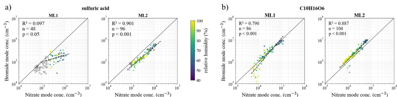
Figure 7. Scatter plots of hourly median concentrations measured in bromide mode versus nitrate mode for (a) sulfuric acid and (b) C_{10}H_{16}O_6 obtained with ML1 and ML2 during 27–30 July 2024. Dashed lines indicate linear regressions for each plot, with the corresponding coefficient of determination ( R^2 ), number of data points considered ( n ), and probability value ( p ) reported. The color of the points represents the relative humidity, as indicated by the color bar in the center. Points falling below the corresponding LOD_{CIMS} are shown as crosses (X), while outliers are plotted as smaller semi-transparent points; both are excluded from the linear fits.
