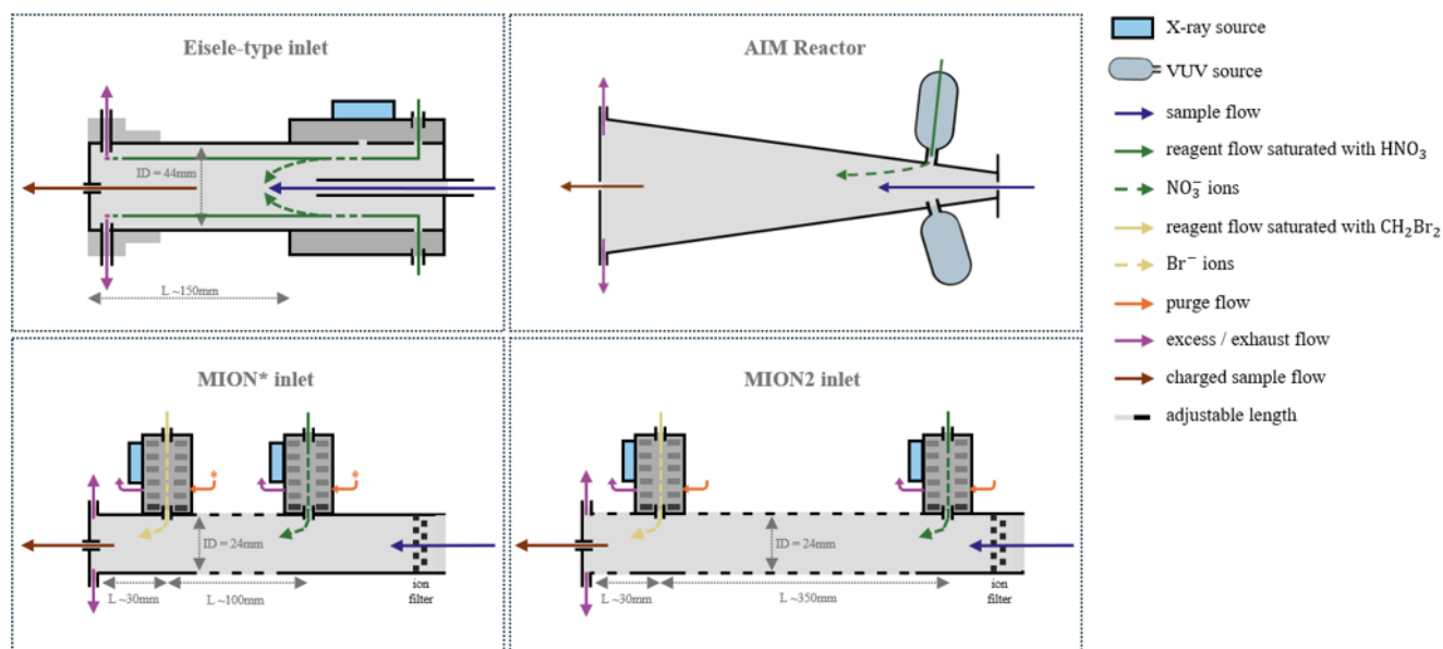
Figure 1. Schematic representation of the chemical ionization inlets employed during the ACTRIS CI-FII campaign: Eisele-type inlet, AIM Reactor, MION* inlet, and MION2 inlet. The MION* inlet incorporates an added purge flow compared to the original MION design described by Rissanen et al. (2019), and is therefore denoted with an asterisk.
