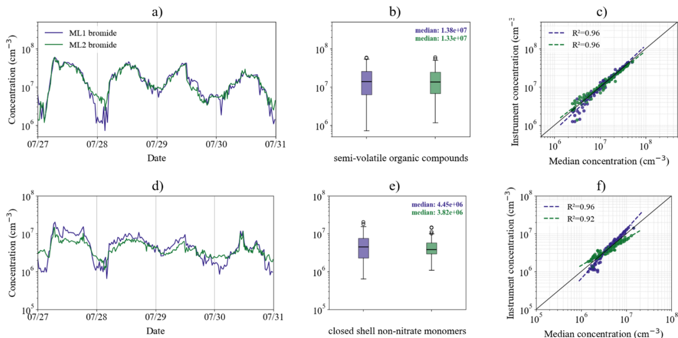
Figure 6. Concentrations of (a–c) semi-volatile organic compounds, and (d–f) closed shell non-nitrate monomers measured in bromide mode by ML1 and ML2 during 27–30 July 2024. For each panel, the left panels (a, d) show concentration time series, while the central panels (b, e) show a box plot summarizing the distributions over the same period. Boxes indicate the interquartile range, horizontal lines indicate the median, whiskers represent the non-outlier range, and empty circles denote outliers. The right panels (c, f) show the hourly median concentration measured by each instrument against the mean of the corresponding hourly median concentrations from the two instruments. Dashed lines indicate log–log linear regressions for each instrument, with the corresponding coefficient of determination ( R^2 ) reported in the legend. Outliers are plotted as smaller semi-transparent points and are excluded from the linear fits.
