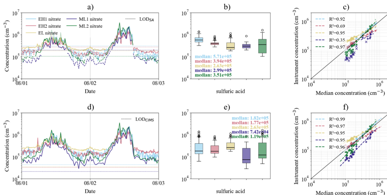
Figure 4. Sulfuric acid concentrations measured in nitrate mode by five CI-API-ToFs during 1–2 August 2024. Upper and lower panels show the same comparison using two different limits of detection: \text{LOD}_{\text{SA}} in the upper panels (a–c) and \text{LOD}_{\text{CIMS}} in the lower panels (d–f). For each panel, the left panels (a, d) show the time series of sulfuric acid concentrations, with instrument-specific LOD values indicated by dotted horizontal lines. The central panels (b, e) show a box plot summarizing the distributions over the same period; boxes indicate the interquartile range, horizontal lines indicate the median, whiskers represent the non-outlier range, and empty circles denote outliers. Data points below LOD are excluded from the box plot. The right panels (c, f) show the hourly median sulfuric acid concentration measured by each instrument against the median of the hourly median concentrations across all five instruments. Dashed lines indicate log–log linear regressions for each instrument, with the corresponding coefficient of determination ( R^2 ) reported in the legend. Points below the corresponding LOD are shown as crosses (X), while outliers are plotted as smaller semi-transparent points; both are excluded from the linear fits.
