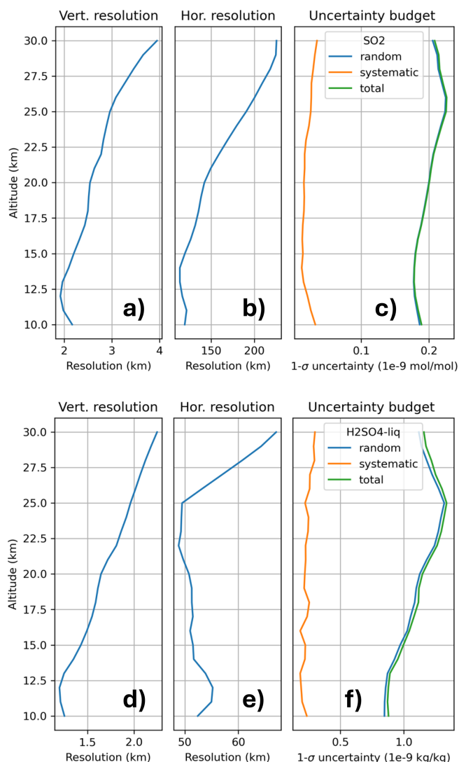
Figure 3. Vertical profile of the vertical (a, d) and horizontal resolutions (b, e) and of the uncertainty budget (c, f) for SO 2 (a–c) and SA CAIRT PO retrievals (d–f). In panels (c) and (f), the blue, orange and green curves represent the random, systematic and total uncertainties, respectively. The vertical and horizontal resolution and the uncertainty budget, for both SO 2 and SA, are representative of individual retrievals with 100 km across-track binning.
