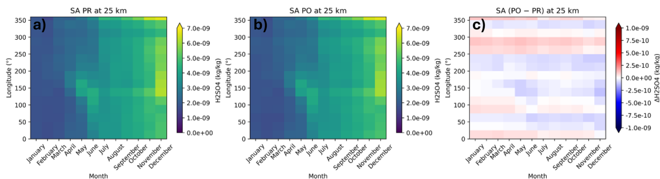
Figure 6. Time series of monthly average meridional mean total SA mass concentration at 25 km altitude, for the Geo SSP5-34-OS 2.0 PR scenario (a) and corresponding CAIRT PO (b), for year 2034. The absolute difference of PO and PR monthly average meridional means are shown in panel (c).
