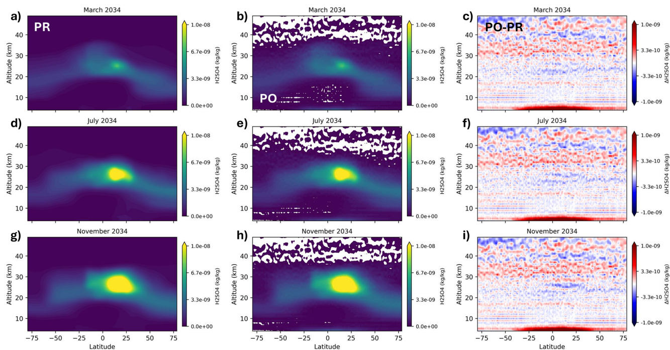
Figure 7. Zonal average vertical profiles of the total SA mass concentration, for the Geo SSP5-34-OS 2.0 PR scenario, for selected months of the year 2034 – monthly averages (a, d, g) and corresponding CAIRT PO averages (b, e, h). The absolute difference of PO and PR average profiles are shown in the third column (c, f, i).
