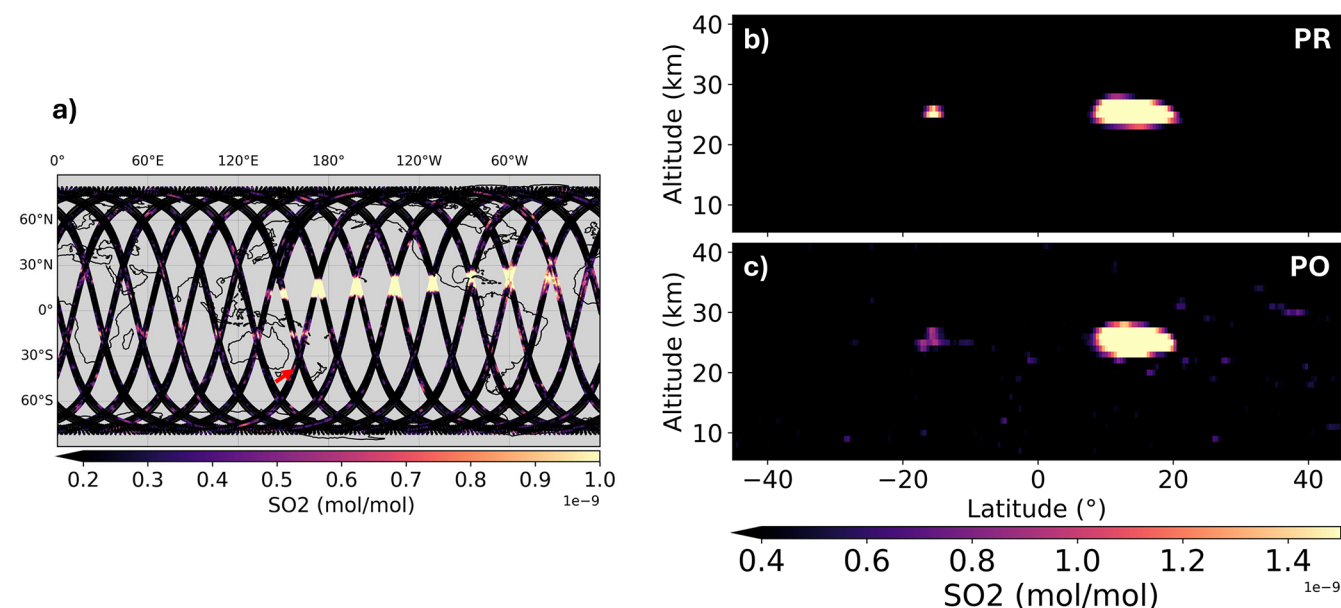
Figure 4. (a) CAIRT POs of the SO 2 mixing ratio for February 2034, at 25 km altitude. (b–c) Across-track average PR (b) and CAIRT PO (c) of the SO 2 vertical profiles, for the orbit segment individuated with a red arrow in panel (a).
