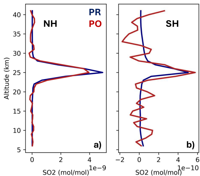
Figure 5. Average vertical SO 2 profiles, PR (blue lines) and CAIRT PO (red lines), for the two SO 2 injection points visible in Fig. 4b–c (a: injection point in the NH, at 15°N; b: injection point in the SH, at 15°S). The total SO 2 mass intercepted by the CAIRT POs, for the two injection points, is (a) 3.1 t (PR: 3.4 t) and (b) 0.4 t (PR: 0.5 t).
