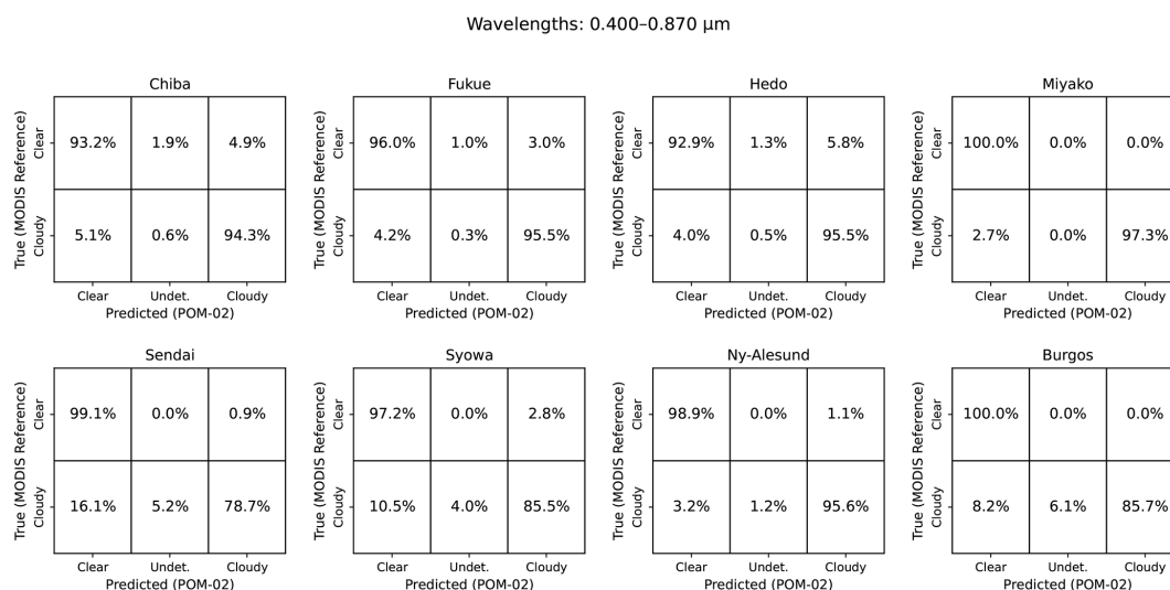
Figure 8. Same as Fig. 6, but for the spectral slope between 0.400 and 0.870 \mu\text{m} .
