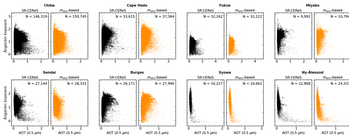
Figure 11. Scatter plots of Ångström exponent (AE) versus aerosol optical thickness (AOT) at 0.5\ \mu\text{m} for eight SKYNET sites after cloud screening using two systems: the SR-CEReS package (left panels) and the slope-based method derived from the atmospheric slope of zenith radiance between 0.500 and 0.675\ \mu\text{m} with \epsilon value of 0.05 (right panels). Numbers indicate the total observations retained by each method.
