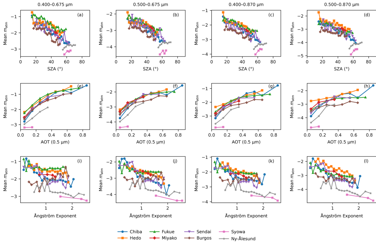
Figure 4. Dependence of mean spectral atmospheric slope ( m_{\text{atm}} ) values on solar zenith angle (SZ), aerosol optical thickness (AOT), and Ångström exponent (AE) under clear-sky conditions identified using the reference MODIS cloud mask data. Mean values were calculated at each site using bin intervals of 2^\circ for SZ, 0.1 for AOT, and 0.1 for the AE.
