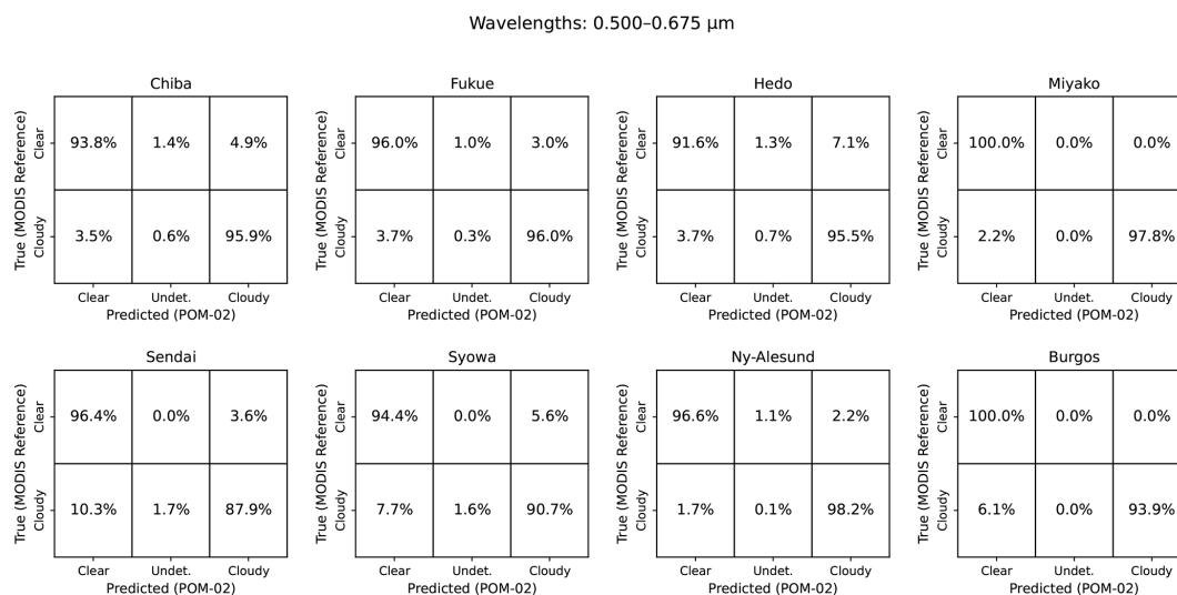
Figure 7. Same as Fig. 6, but for the spectral slope between 0.500 and 0.675 \mu\text{m} .
