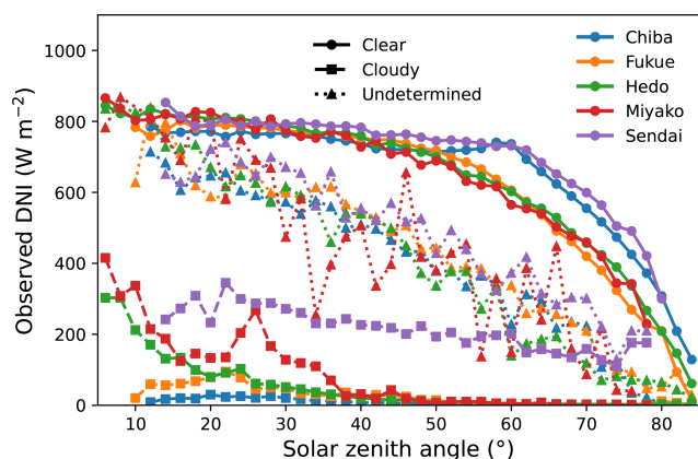
Figure 10. Relationship between median values of observed direct normal irradiance (DNI) within a 2^\circ solar zenith angle (SZA) bin and SZA for clear, cloudy, and undetermined conditions predicted using wavelength pair of 0.500 and 0.675 with \epsilon = 0.05 at (a) Chiba, (b) Hedo, (c) Fukue, (d) Miyako, and (e) Sendai.
