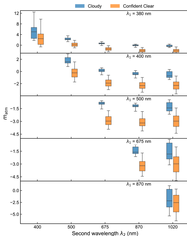
Figure 3. Box-and-whisker distributions of spectral slope values of atmospheric slope ( m_{\text{atm}} ) for cloudy and confidently clear sky conditions for Chiba. Each row corresponds to a fixed first wavelength ( \lambda_1 ), while the x -axis represents the second wavelength ( \lambda_2 ). In the figure, the boxes represent the 25th and 75th percentiles, and the whiskers represent the 5th and 95th percentiles.
