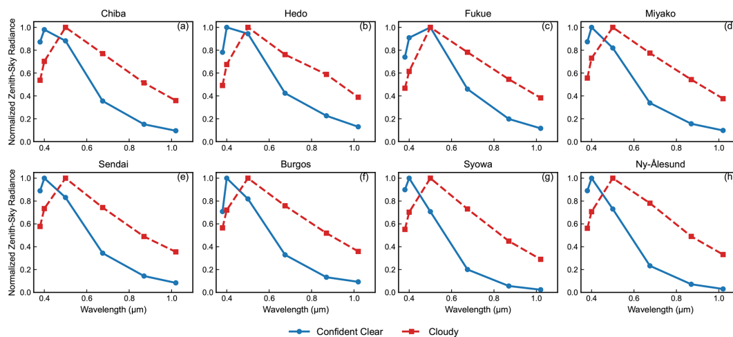
Figure 2. Median normalized spectral zenith sky radiance under cloud and confidently clear sky conditions at (a) Chiba, (b) Hedo, (c) Fukue, (d) Miyako, (e) Sendai, (f) Burgos, (g) Syowa, and (h) Ny-Ålesund. Zenith sky radiances were normalized by the maximum value within each observation and averaged separately for MODIS-identified cloudy and confidently clear cases.
