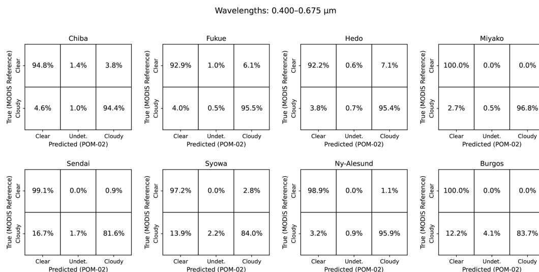
Figure 6. Confusion matrices for clear, undetermined, and cloudy sky discrimination using atmospheric slope ( m_{\text{atm}} ) values determined using 0.400 and 0.675 \mu\text{m} wavelength pair. MODIS cloud-mask classifications are used as the reference, while POM-02 slope-based classifications are treated as predictions. Each matrix is normalized by the MODIS reference class, so that each row sums to 100 %.
