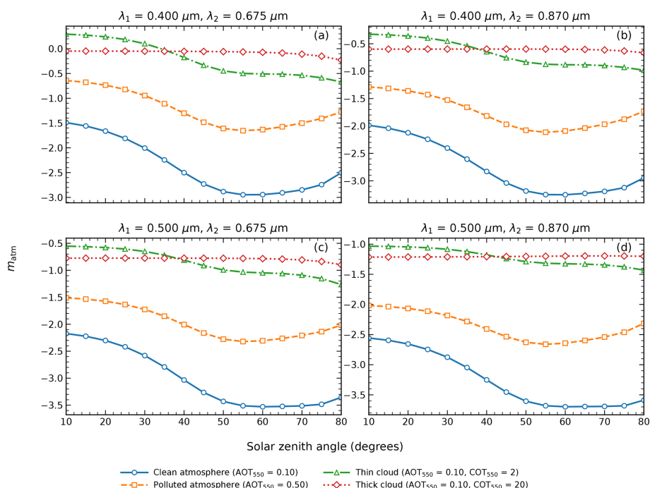
Figure 1. Atmospheric spectral slope ( m_{\text{atm}} ) as a function of solar zenith angle (SZA) simulated for four selected wavelength pairs: (a) 0.400–0.675 \mu\text{m} , (b) 0.400–0.870 \mu\text{m} , (c) 0.500–0.675 \mu\text{m} , and (d) 0.500–0.870 \mu\text{m} . Simulations were performed with mid-latitude summer atmospheric model, precipitable water vapor of 1.0 cm, total column ozone of 0.30 cm-atm, Lambertian surface albedo of 0.10, and clouds represented as plane-parallel layers.
