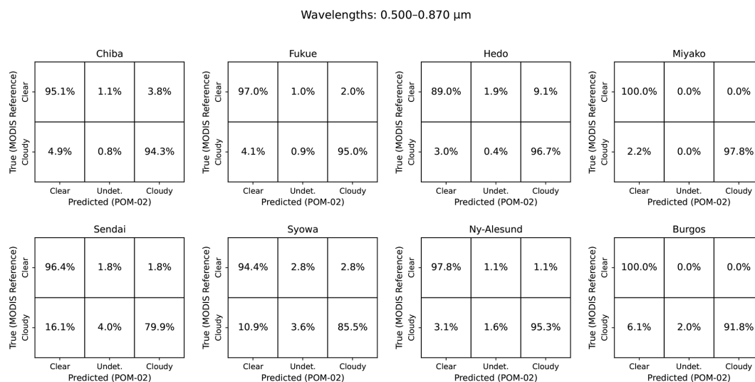
Figure 9. Same as Fig. 6, but for the spectral slope between 0.500 and 0.870 \mu\text{m} .
