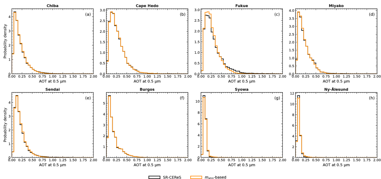
Figure 12. Probability density distributions of aerosol optical thickness (AOT) at 0.5\ \mu\text{m} obtained after clear-sky screening using the SR-CEReS procedure and the proposed atmospheric-slope-based method at the eight SKYNET sites. A fixed AOT bin width of 0.05 was used for the probability density calculation. For clarity, the displayed AOT range is limited to 0 – 2.0 , although the probability density analysis was performed using all valid observations over the full analysis range.
