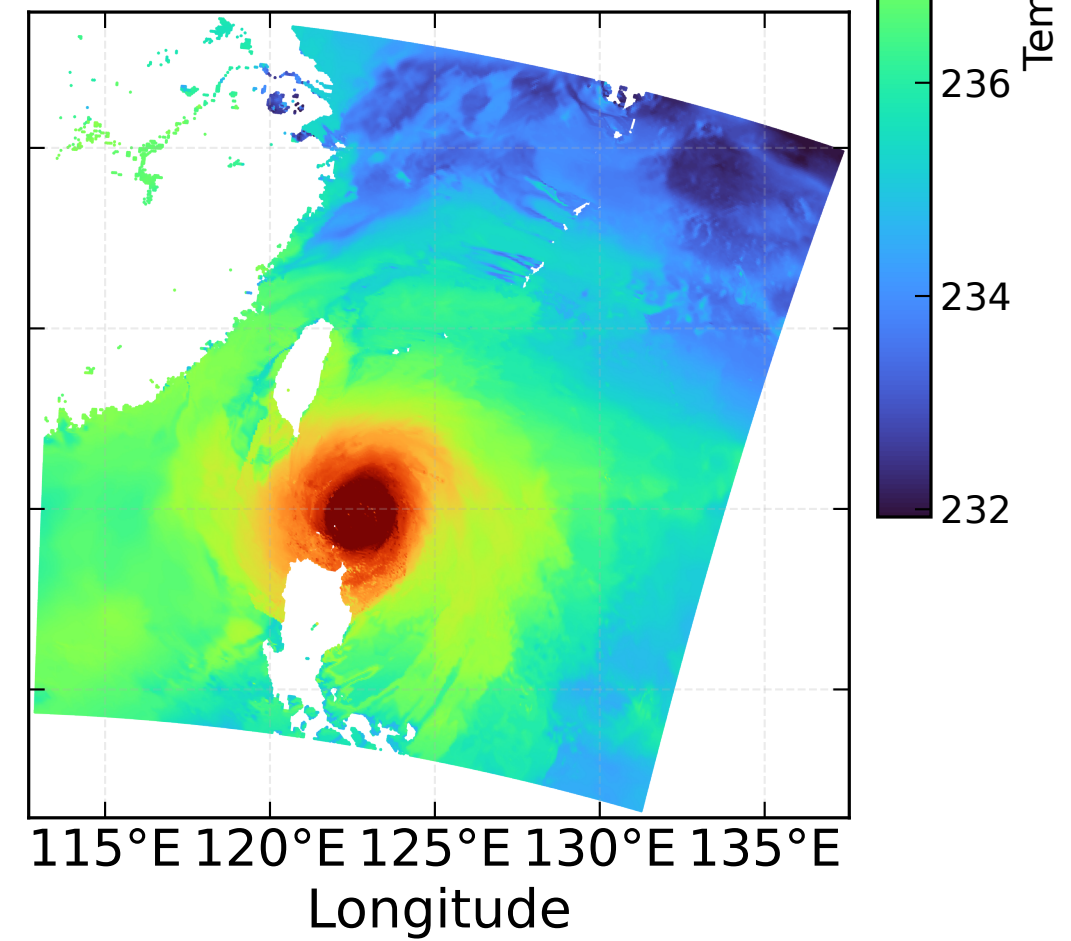
(f) Retrieval-250 hPa
