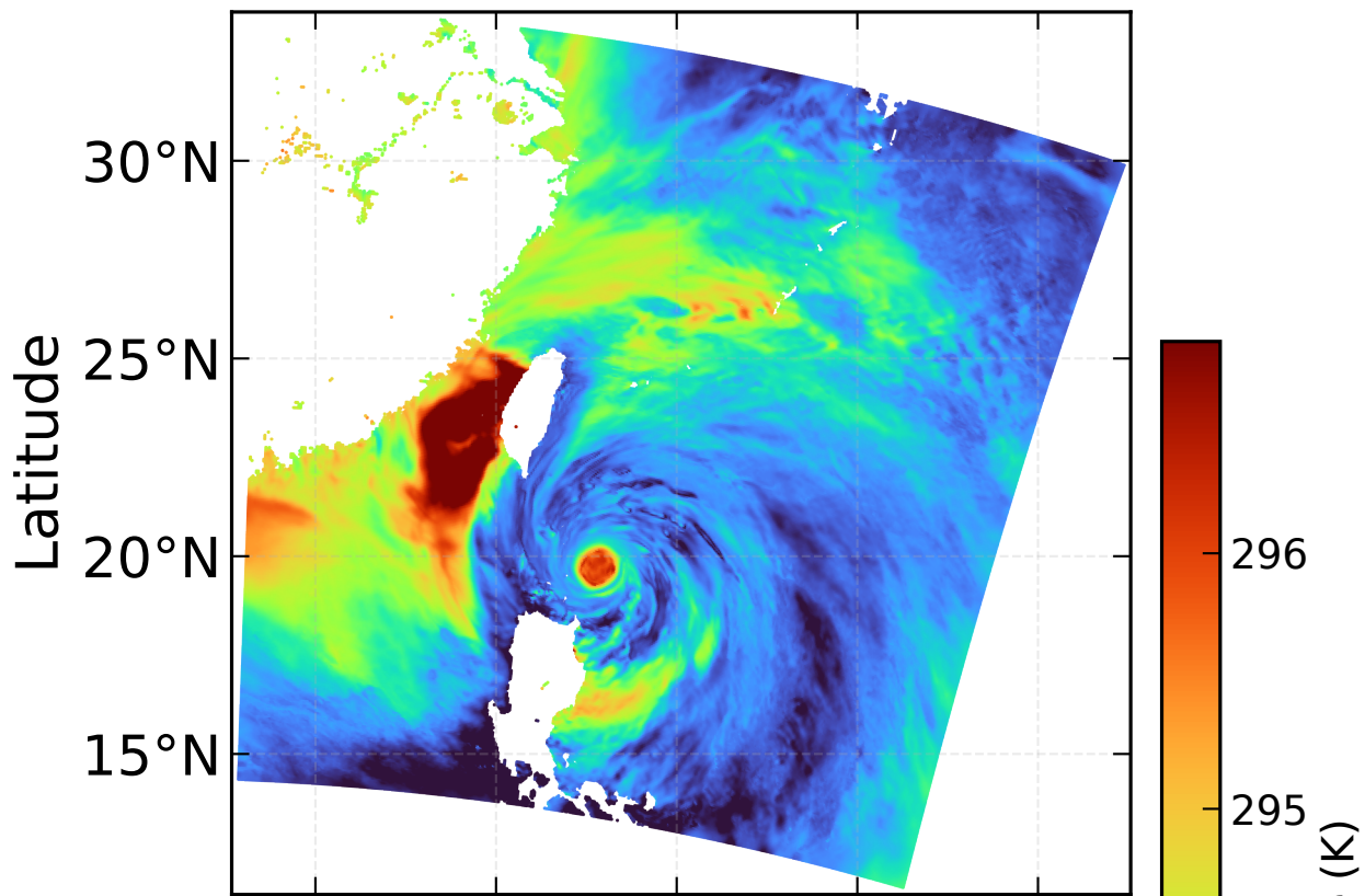
(a) Reference-850 hPa
