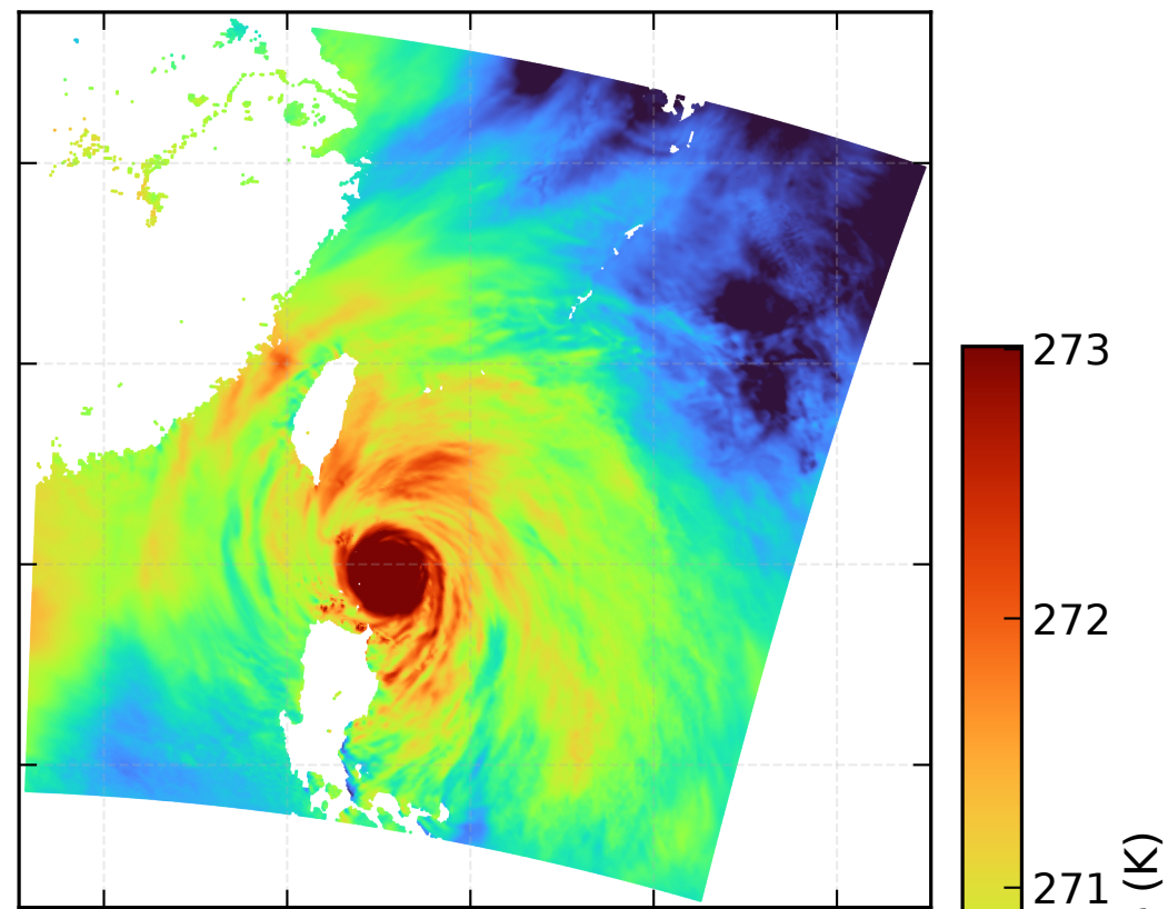
(b) Reference-500 hPa
