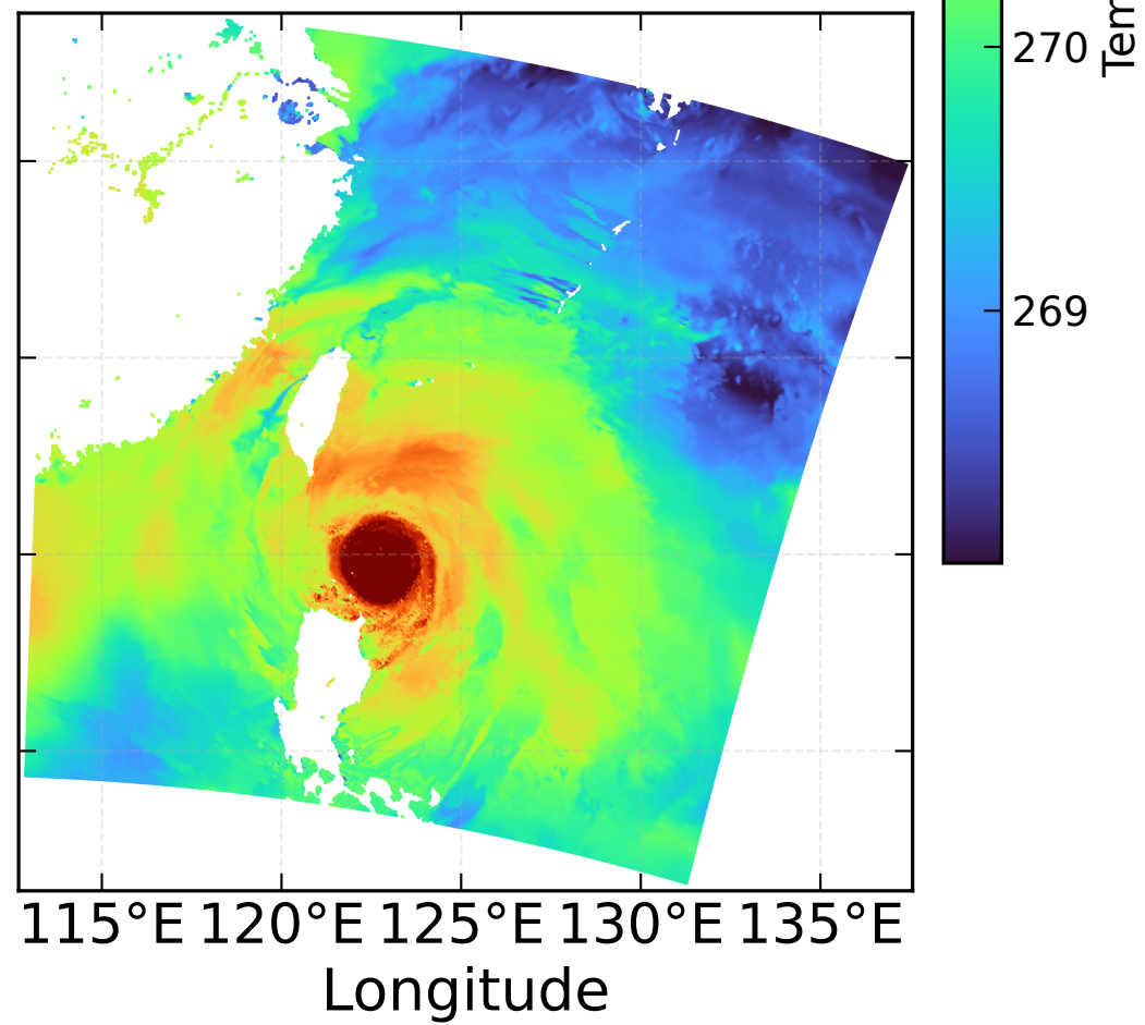
(e) Retrieval-500 hPa
