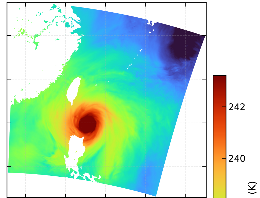
(c) Reference-250 hPa
