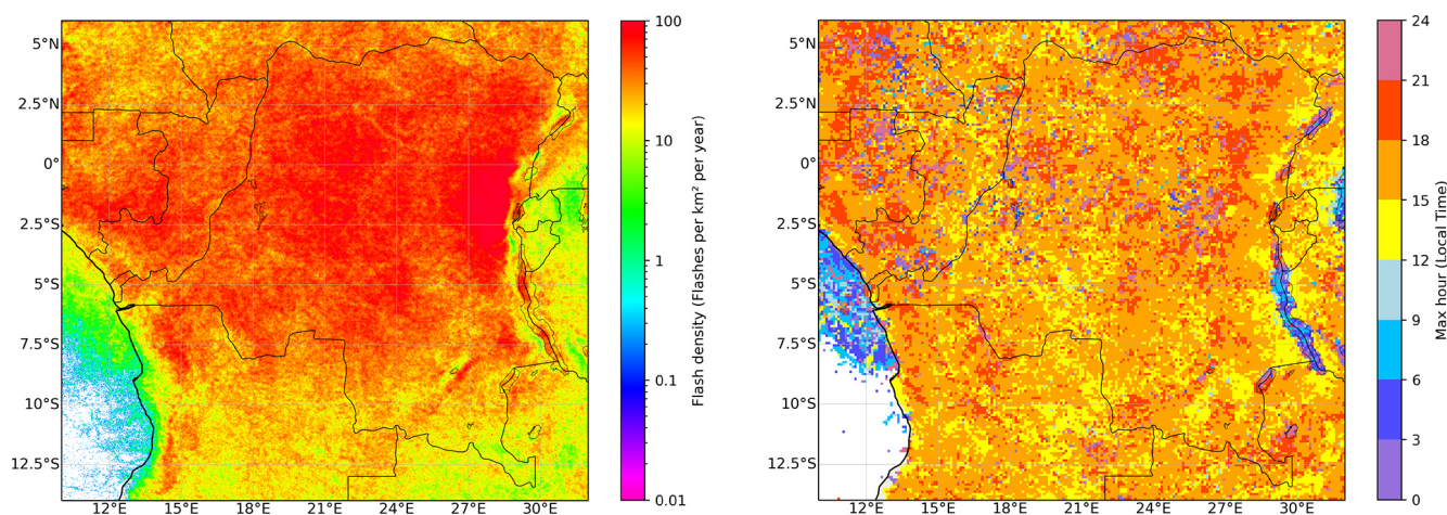
Figure 8. High-resolution 0.02^\circ \times 0.02^\circ MTG-LI flash density (flashes \text{km}^{-2} \text{yr}^{-1} ; left) and 0.1^\circ \times 0.1^\circ resolution peak hour of lightning activity (right) in the Congo Basin from July 2024 to June 2025.
