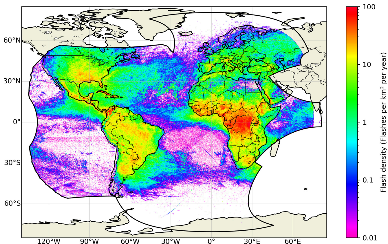
Figure 11. Spatial distribution of GOES-GLM and MTG-LI merged flash density (flashes \text{km}^{-2} \text{yr}^{-1} ) from July 2024 to June 2025 on a 0.1^\circ \times 0.1^\circ spatial grid. The black polygon represents the union between the FOV of GLM on GOES-East and FOV of MTG-LI.
