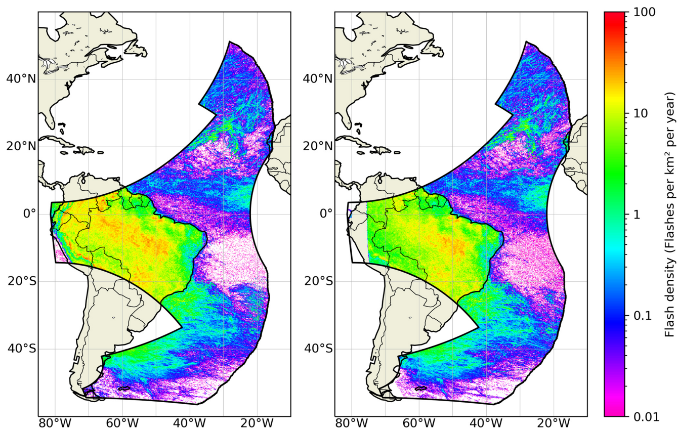
Figure 10. Spatial distribution of GOES-GLM (left) and MTG-LI (right) flash density (flashes \text{km}^{-2} \text{yr}^{-1} ) from July 2024 to June 2025 on a 0.1^\circ \times 0.1^\circ spatial grid. The black polygon represents the overlap between the FOV of GLM on GOES-East and FOV of MTG-LI.
