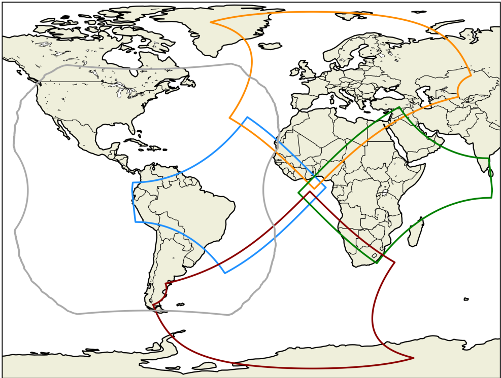
Figure 1. Field of view of GLM on GOES-East (GOES-16 and GOES-19) (gray), and of the four Sectors covered by MTG-LI cameras without considering the parallax correction effects described in the text (West in blue, North in orange, East in green, and South in red, respectively).
