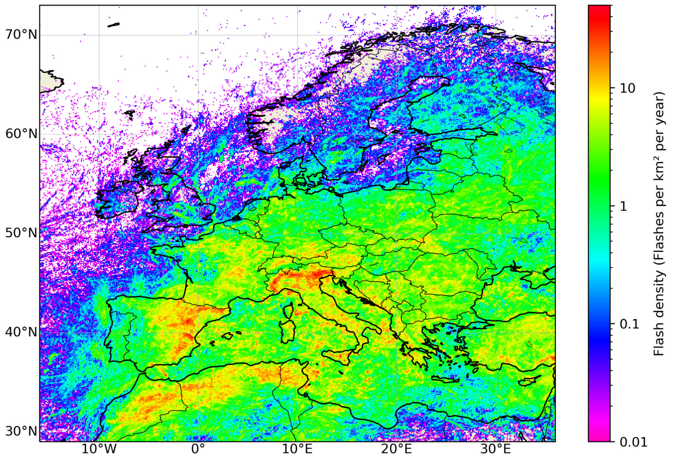
Figure 3. Spatial distribution of MTG-LI flash density (flashes \text{km}^{-2} \text{yr}^{-1} ) over Europe from July 2024 to June 2025 on a 0.1^\circ \times 0.1^\circ spatial grid. Note, the scaling of the colour palette is different from Fig. 2.
