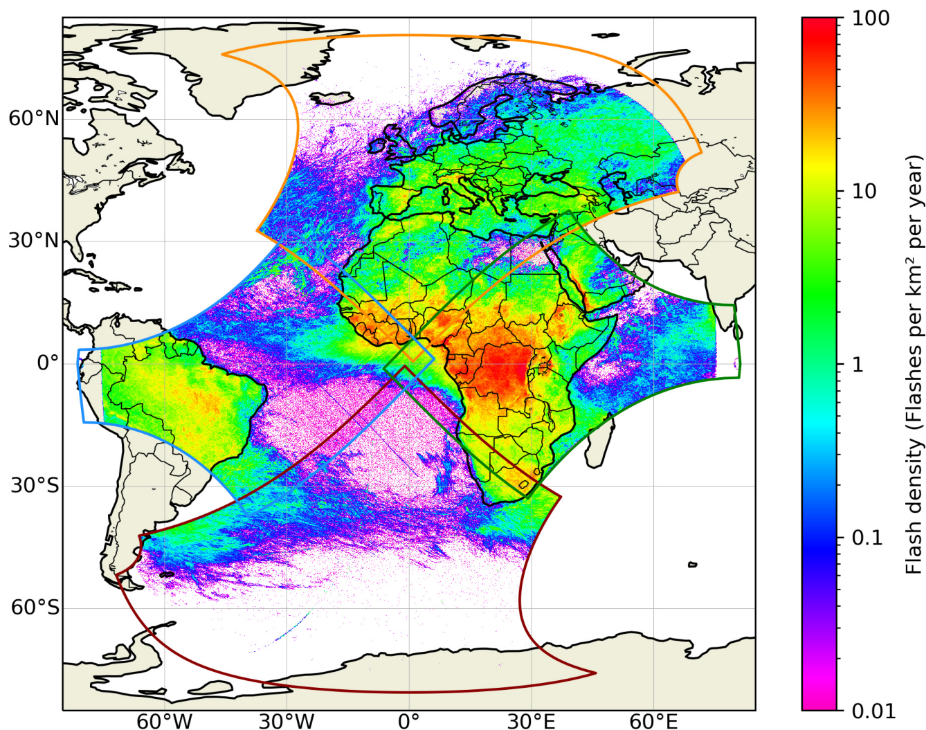
Figure 2. Spatial distribution of MTG-LI flash density (flashes \text{km}^{-2} \text{yr}^{-1} ) over the full MTG-LI FOV from July 2024 to June 2025 on a 0.1^\circ \times 0.1^\circ spatial grid.
