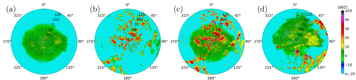
Figure 5. Comparison of Cartesian representations of different DBZH images: (a) cluttered summer radar image, (b) winter radar image, (c) their corresponding synthetic radar image with weighting factors \lambda_w = 6.5 , and \lambda_s = 1 and (d) mixed summer radar image. The radar images shown were measured (a) on 18 June 2022, at 10:00 UTC in Neuheilenbach, (b) on 9 January 2025, at 17:00 UTC in Borkum and (d) on 16 June 2022, at 09:55 UTC in Memmingen.
