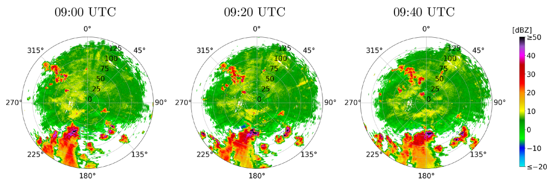
Figure 13. Time series of mixed summer radar images collected at the same radar station at 20 min intervals. The radar images shown were measured on 16 June 2022 in Isen.
