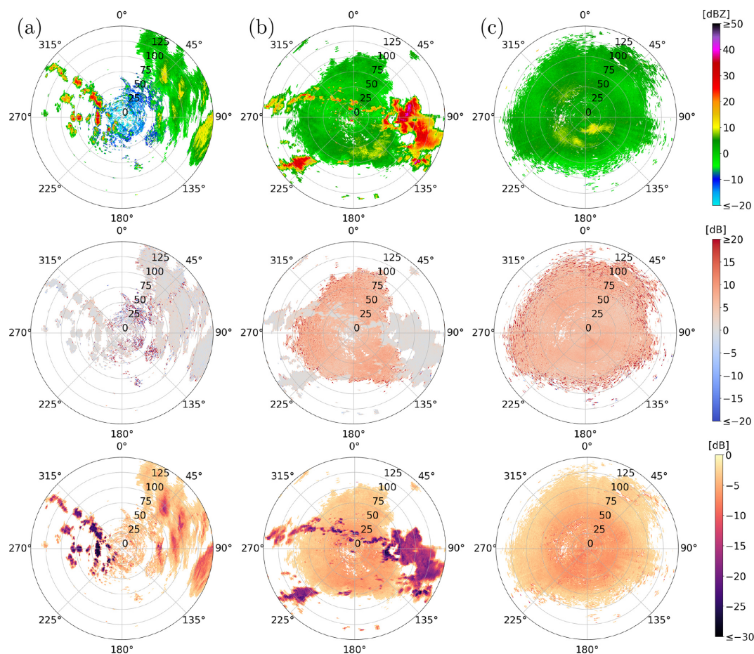
Figure 1. Horizontal reflectivity (first row), differential reflectivity (second row), and depolarization ratio (third row) for examples of (a) a winter sweep, (b) a mixed summer sweep, and (c) a cluttered summer sweep. White pixels are filtered by the initial preprocessing done by DWD. The sweeps shown were measured (a) on 9 January 2025, at 17:55 UTC in Flechtdorf, (b) on 16 June 2022, at 09:00 UTC in Dresden and (c) on 18 June 2022, at 10:00 UTC in Isen.
