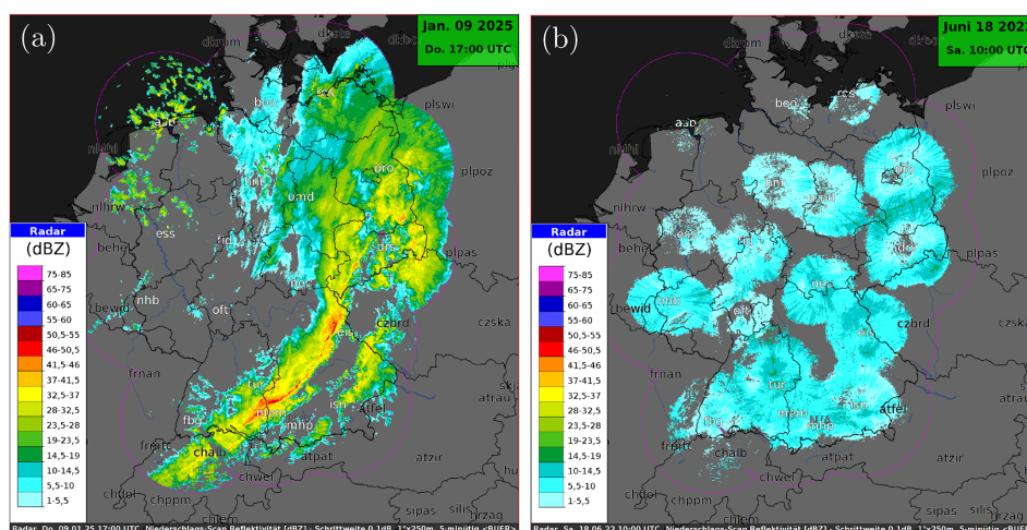
Figure 2. Composite radar images of the horizontal reflectivity over Germany: (a) the precipitation during the winter period, on 9 January 2025, at 17:00 UTC, and (b) the non-meteorological echoes during the cluttered summer period, on 18 June 2022, at 10:00 UTC.
