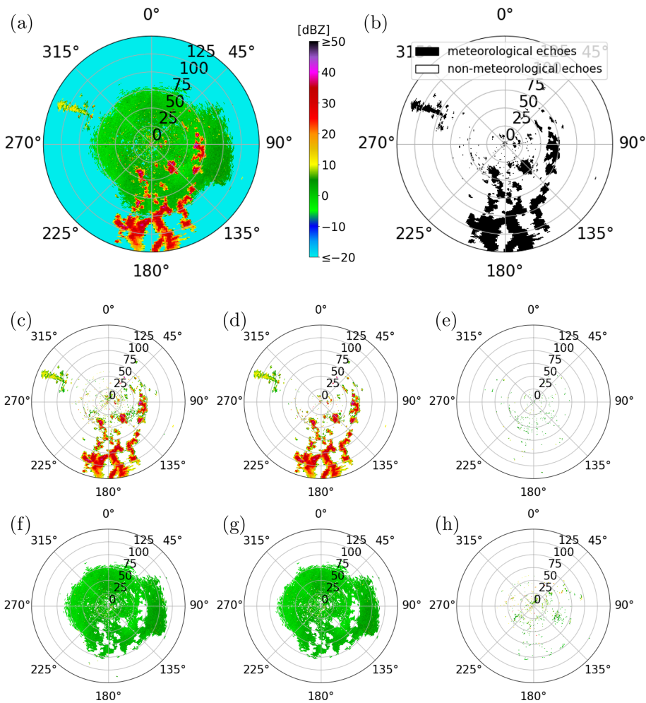
Figure 10. Evaluation of the network on a synthetic validation image: (a) input image and (b) corresponding ground truth, (c) pixels classified as meteorological echoes by the network, (d) correctly classified meteorological echoes, and (e) meteorological echoes misclassified as non-meteorological echoes. The bottom row shows (f) pixels classified as non-meteorological echoes, (g) correctly classified non-meteorological echoes, and (h) non-meteorological echoes misclassified as meteorological echoes. The radar image shown was generated using two radar images measured on 9 January 2025, at 17:05 UTC and on 18 June 2022, at 10:55 UTC in Essen.
