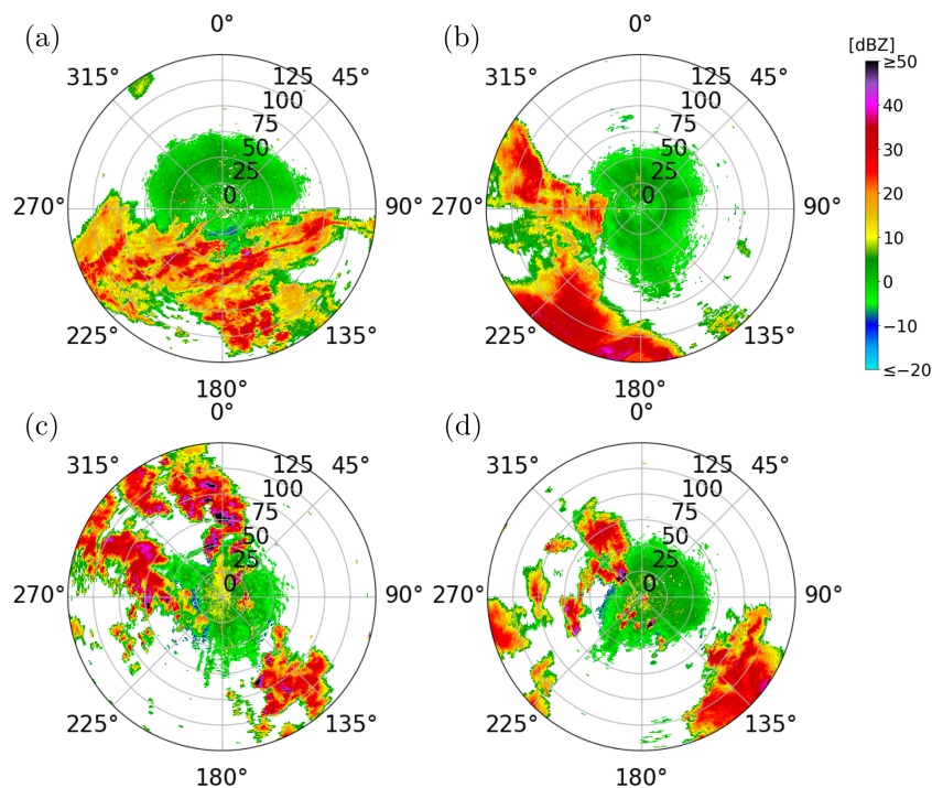
Figure 9. Overview of four of the five DBZH radar images in the test dataset \mathcal{D}_{\text{exp}}^{\text{m}} . The radar images shown were measured (a) on 5 June 2022, at 09:00 UTC in Essen, (b) on 5 June 2022, at 09:00 UTC in Neuhaus, (c) on 30 June 2022, at 16:00 UTC in Neuheilenbach and (d) on 30 June 2022, at 16:00 UTC in Türkheim. The remaining radar image from \mathcal{D}_{\text{exp}}^{\text{m}} , which was measured on 16 June 2022, at 09:00 UTC in Dresden, is shown in Fig. 1b.
