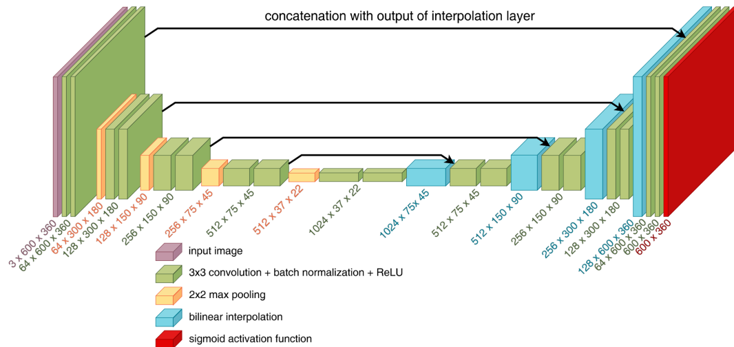
Figure 4. Schematic representation of the network architecture with n_f = 64 feature channels in the first downsampling step. Below each layer, the respective output dimensions are given.
