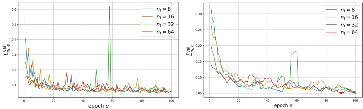
Figure 8. Validation loss L_{n_f,e}^{\text{val}} (left) and its moving average \bar{L}_{n_f,e}^{\text{val}} (right) over the epochs e for each number of feature channels n_f \in \{8, 16, 32, 64\} .
