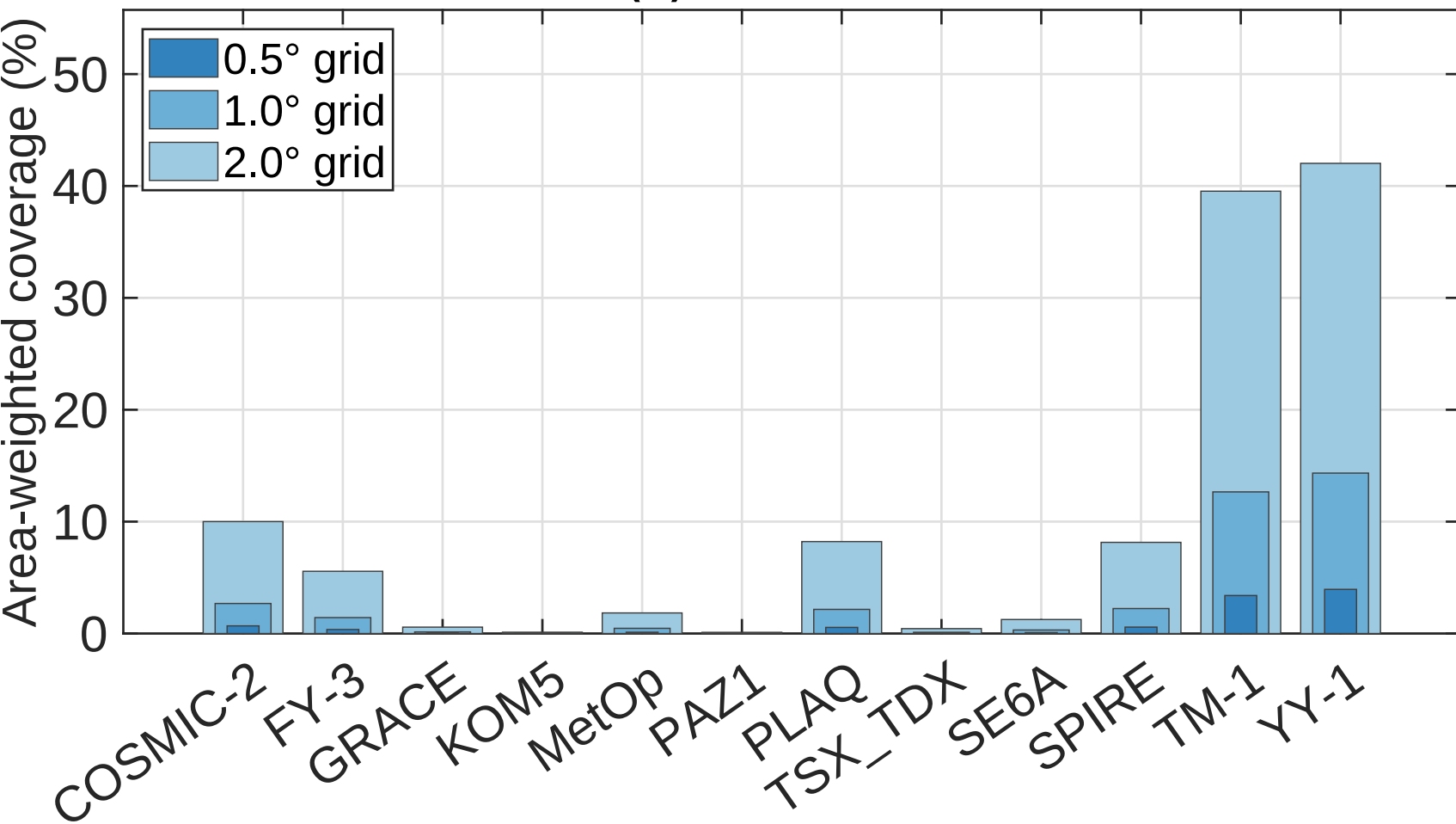
(c) 12–18 UTC
