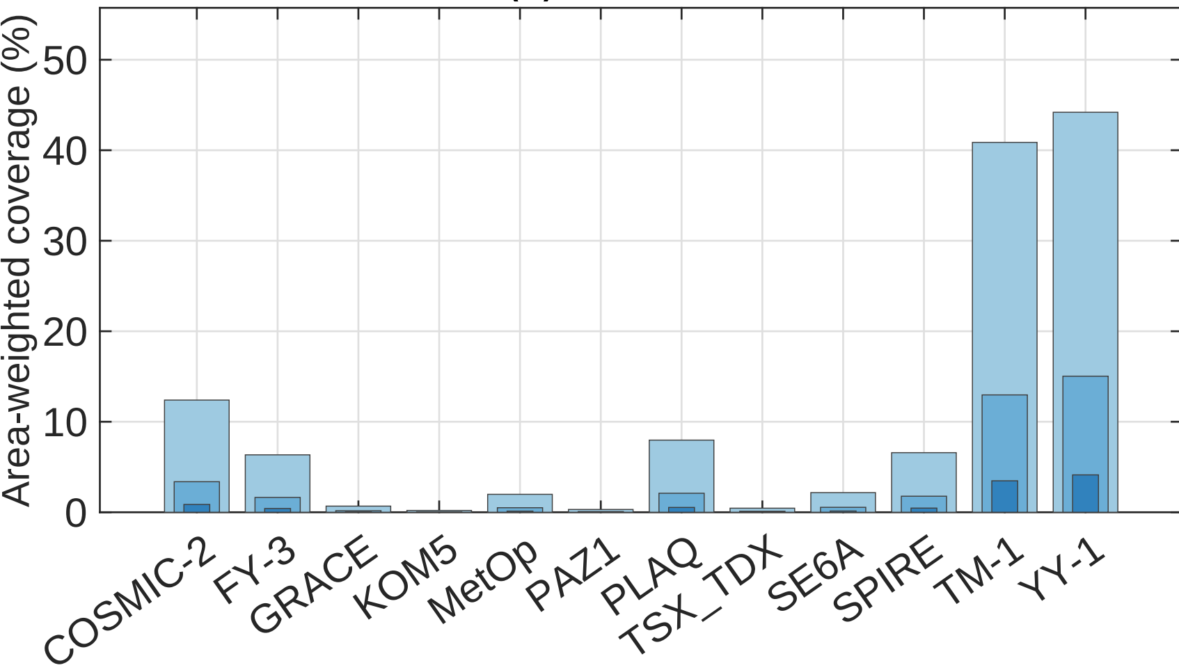
(c) 12–18 UTC
