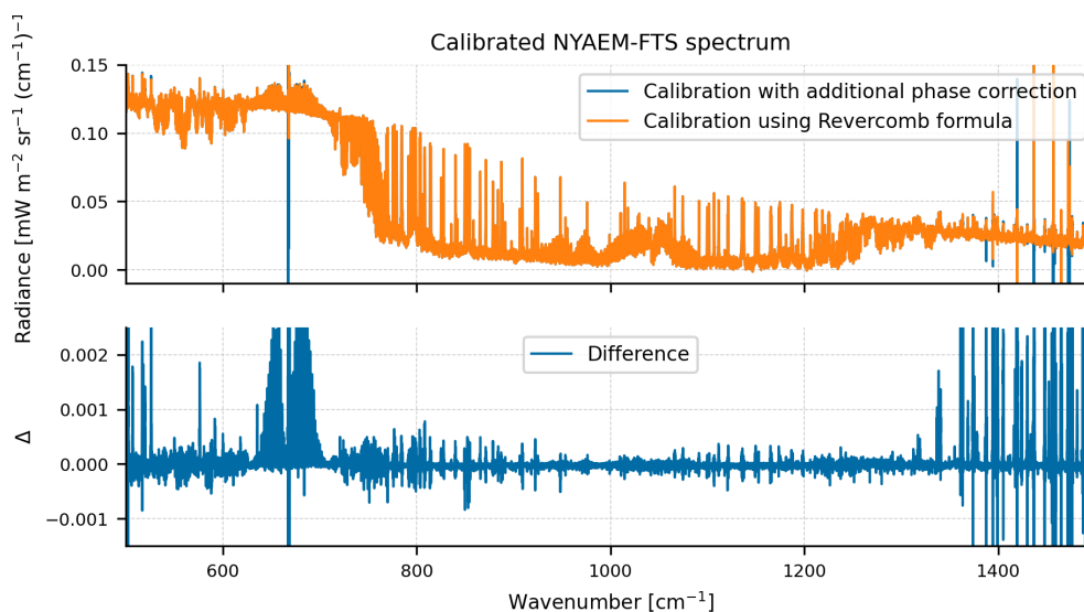
Figure 8. Representative calibrated spectrum measured with the NYAEM-FTS under clear sky conditions. Comparison between Revercomb and the modified calibration method shows influence where strong water vapor and CO 2 lines are present.
