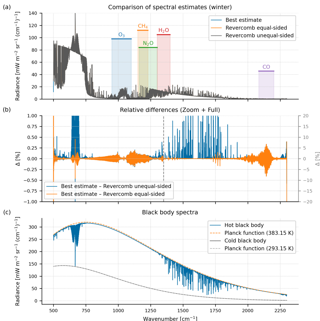
Figure 4. As in Fig. 3, panel (a) shows the best estimate in blue, the Revercomb calibration for equal-sided interferograms (modified method for unequal-sided interferograms) in orange and the application of the original Revercomb method to unequal-sided interferograms in gray, but for the entire measured mid-infrared spectral range. Panel (b) shows the relative differences. In the left part, where absorption lines are small in the blackbody spectrum, the differences are minor and become larger the stronger the absorption lines in the blackbody spectrum as can be seen on the right hand side (note the different axis scalings). The blackbody spectra are shown in panel (c). All are synthetic spectra from a realistic Arctic atmospheric winter profile (see Fig. 2).
