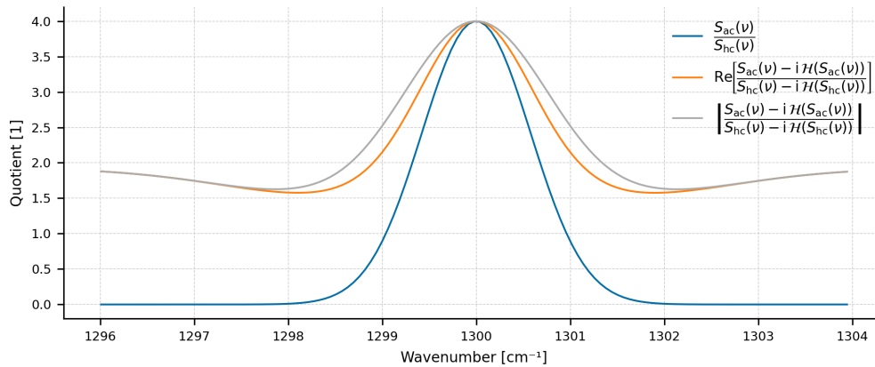
Figure A1. The quotient of two Gaussian lines is shown in blue. The orange graph shows the real part of the quotient of the complex spectra that are obtained if the interferograms corresponding to the Gaussian lines are subject to one-sided truncation. The magnitude instead of the real part is shown in gray.
