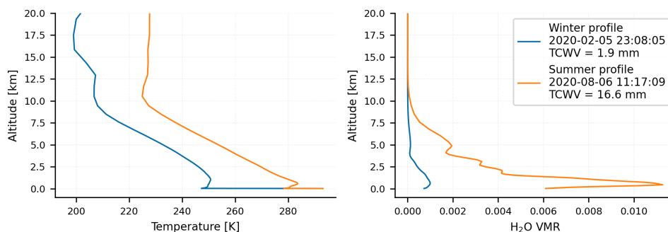
Figure 2. Representative temperature and humidity profiles for summer and winter in Ny-Ålesund, Svalbard. The abrupt peak at the bottom of the temperature profile corresponds to the column of warm lab air between the spectrometer and the hatch in the roof. The total column of water vapor (TCWV) varies largely between summer and winter.
