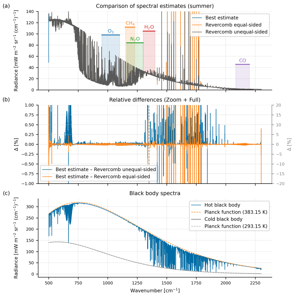
Figure 5. Same as Fig. 4 but for summer.
