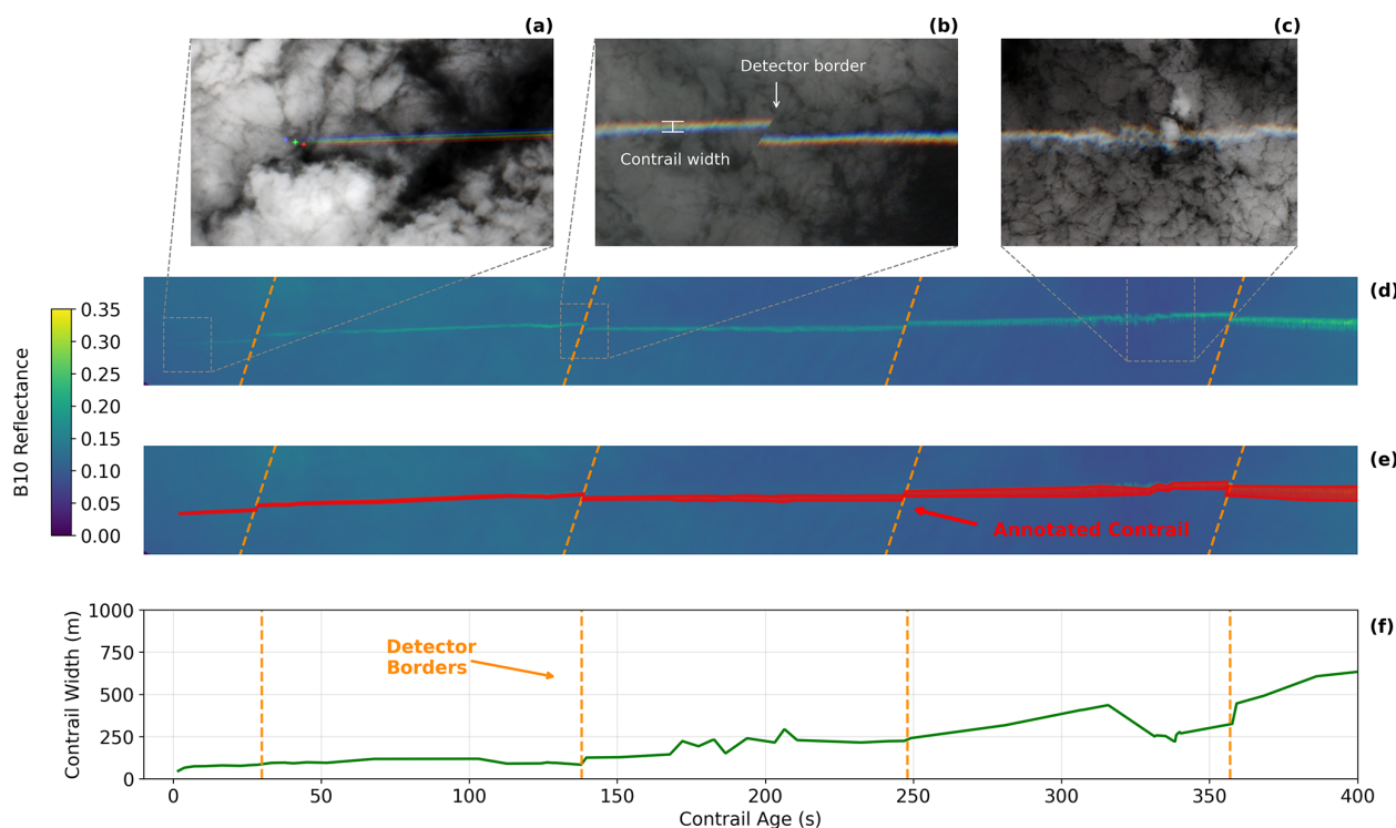
Figure 3. (a) Sentinel-2 true colour image showing the aircraft and the contrail in the first 10 s. (b) Sentinel-2 true colour image of the contrail after 140 s showing discontinuity caused by the detector border. (c) Sentinel-2 true colour image showing how the contrail loses its linearity after the wake vortex pair has broken down. (d) Sentinel-2 B10 top-of-atmosphere reflectance of the contrail. The vertical dimension of the image has been increased by a factor of 2 as compared to the horizontal dimension to improve the visibility of the contrail. (e) Same as panel (d), with manually annotated contrail polygon. (f) Contrail width as a function of contrail age. Dashed lines indicate the locations of the detector borders. Panels (a)–(e) contain modified Copernicus Sentinel data 2021.
