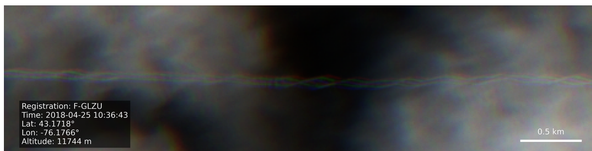
Figure D3. Contrail observed in Sentinel-2 imagery illustrating the occurrence of the Crow instability (Crow, 1970). Contains modified Copernicus Sentinel data 2018.
