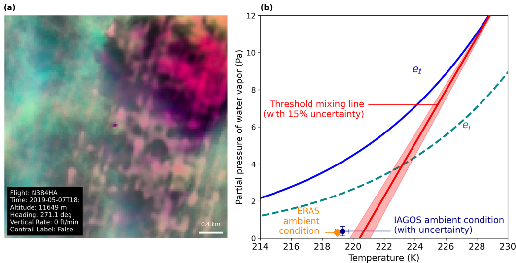
Figure A3. Same as Fig. A1, but for a Landsat false colour composite. Landsat-8 image courtesy of the U.S. Geological Survey.
