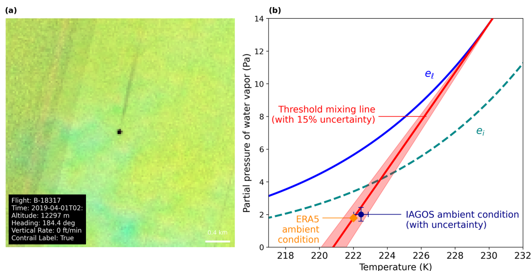
Figure A2. Same as Fig. A1, but for a Landsat false colour composite. Landsat-8 image courtesy of the U.S. Geological Survey.
