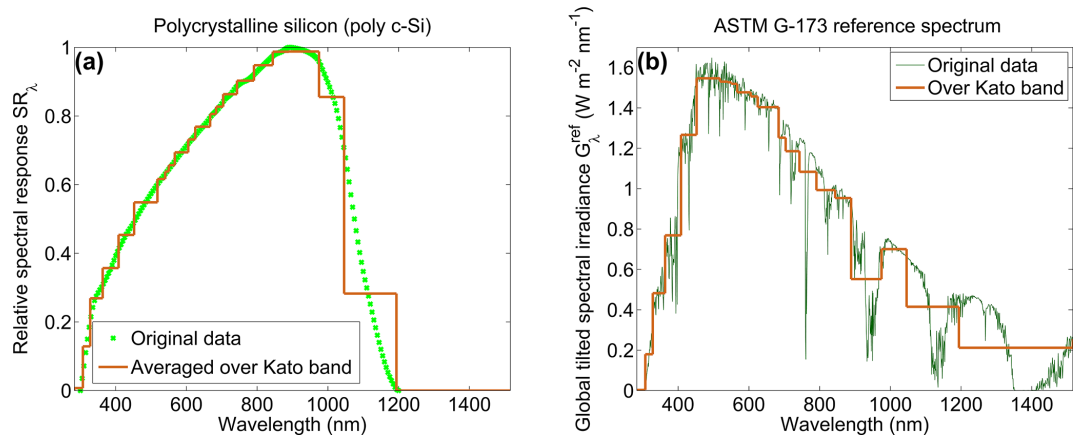
Figure 1. (a) Relative spectral response (on vertical axis) of polycrystalline silicon cell as function of wavelength (on horizontal axis). (b) ASTM G173-03 reference spectrum (on vertical axis) as function of wavelength (on horizontal axis). Original data in green and over Kato bands in orange. The spectral response is defined over the wavelength range from 300 to 1200 nm. Out of this wavelength range, the spectral response is 0.
