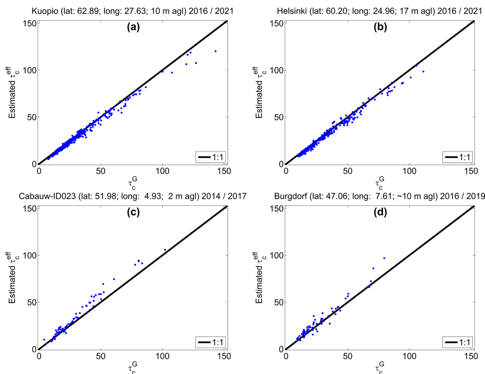
Figure 8. Scatterplots of 15 min averages between \tau_c^G retrievals (horizontal axis) and \tau_c^{\text{eff}} estimates (vertical axis) for water clouds at (a) Kuopio, (b) Helsinki, (c) Cabauw-ID023 and (d) Burgdorf when using CF MODIS for selecting overcast sky conditions.
