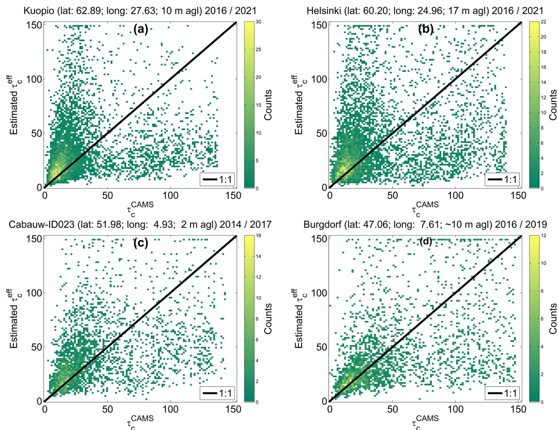
Figure 11. 2D histograms of between instantaneous \tau_c^{\text{CAMS}} retrievals (horizontal axis) and 15 min averages of \tau_c^{\text{eff}} estimates (vertical axis) for water clouds at (a) Kuopio, (b) Helsinki, (c) Cabauw–ID023 and (d) Burgdorf when using \text{CF}^{\text{CAMS}} for selecting overcast sky conditions. The color indicates the number of pairs in the area within the interval 1.5 \times 1.5 .
