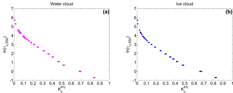
Figure 3. Scatterplot between K_c^{PV} on horizontal axis and \ln(\tau_{c,550}) on vertical axis by varying all parameters except AOD_{550} = 0.074 , \rho_g = 0.2 and w_s = 5 \text{ m s}^{-1} . (a) For water cloud and (b) for ice cloud.
