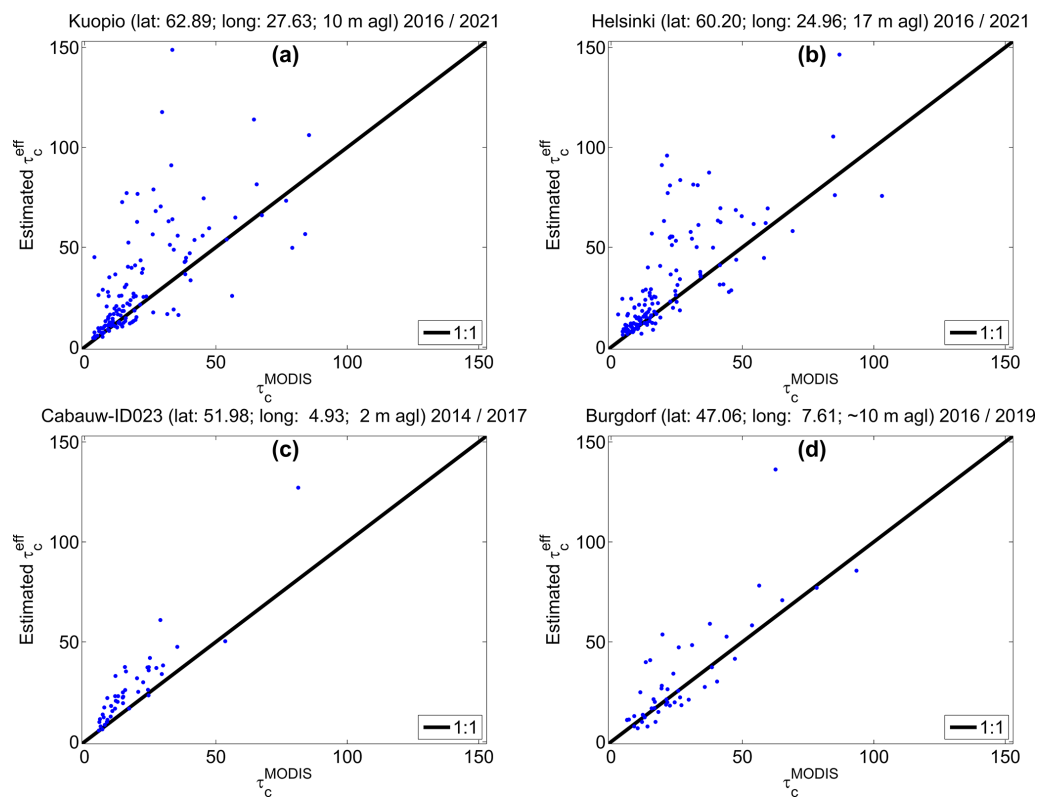
Figure 10. Scatterplots between instantaneous \tau_c^{\text{MODIS}} retrievals (horizontal axis) and 15 min averages of \tau_c^{\text{eff}} estimates (vertical axis) for ice clouds at (a) Kuopio, (b) Helsinki, (c) Cabauw–ID023 and (d) Burgdorf when using \text{CF}^{\text{MODIS}} for selecting overcast sky conditions.
