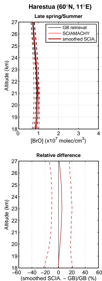
Fig. 10. Comparison between mean SCIAMACHY limb (thin red and thick dark red solid lines) and ground-based UV-visible BrO profiles (solid black line) at Harestua ( 60^{\circ} N, 11^{\circ} E) for evening conditions for the 2002–2006 period (49 coincidences). The mean relative differences appear in the lower plot. They have been plotted for the smoothed SCIAMACHY profile. In both plots, the dashed lines represent the one-sigma standard deviation. The standard deviation of the unsmoothed SCIAMACHY profile is similar to the one calculated for the smoothed profile.
