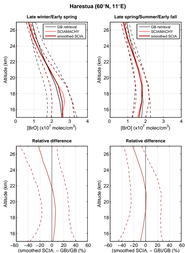
Fig. 9. Comparison between mean SCIAMACHY limb (thin red and thick dark red solid lines) and ground-based UV-visible BrO profiles (solid black line) at Harestua ( 60^{\circ} N, 11^{\circ} E) for the 2002–2006 period (morning coincidences). Profiles have been plotted separately for late winter/early spring (left plot) and late spring/summer/early fall (right plot) conditions. The number of coincident events is 154 and 358, respectively. The mean relative differences appear in the lower plots. They have been plotted for the smoothed SCIAMACHY profiles. In the four plots, the dashed lines represent the one-sigma standard deviation. The standard deviation of the unsmoothed SCIAMACHY profiles is similar to the one calculated for the smoothed profiles.
