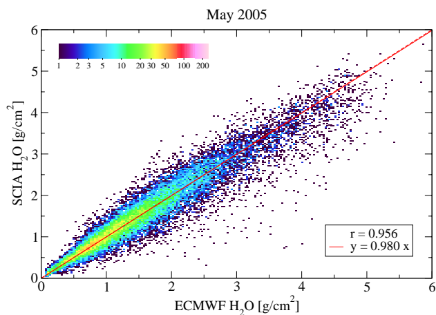
Fig. 11. As Fig. 10, but excluding observations over the Sahara and Australia.
