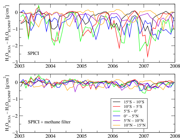
Fig. 9. Monthly averaged differences between total water vapour columns from SCIAMACHY and values derived from ECMWF data averaged over six tropical latitude zones. Upper panel: using cloud filter following Krijger et al. (2005) (SPICI). Lower panel: additionally rejecting observations with \text{CH}_4 total column below 90% of expected value.
