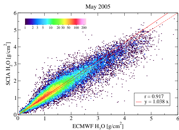
Fig. 10. Density plot of correlation between individual SCIAMACHY total water vapour results and values derived from ECMWF data for all cloud-free observations of May 2005. Results of regression analysis are indicated. The dashed line corresponds to y=x .
