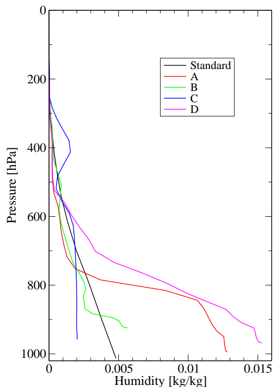
Fig. 15. Standard atmospheric water vapour profile used in test retrievals and typical profiles for locations A–D indicated in Fig. 14.
