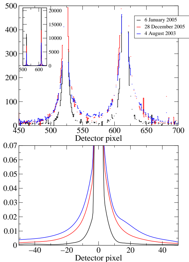
Fig. 2. Upper panel: measurements of two spectral line source (SLS) lines at 2326.66 and 2337.94 nm, respectively. Black: one day after decontamination; red: during the stable phase after mid-2005; blue: during a period of strong scattering. Bad and dead detector pixels have been blanked out. In the inset the same at full scale. Note that the peaks of the red and blue curves are at 62% and 40% of the value measured just after decontamination. Lower panel: modelled slit functions for the three cases in the upper panel for the range \pm 50 detector pixels, corresponding to about \pm 6 nm. The functions are normalised such that their maximum is equal to 1.
