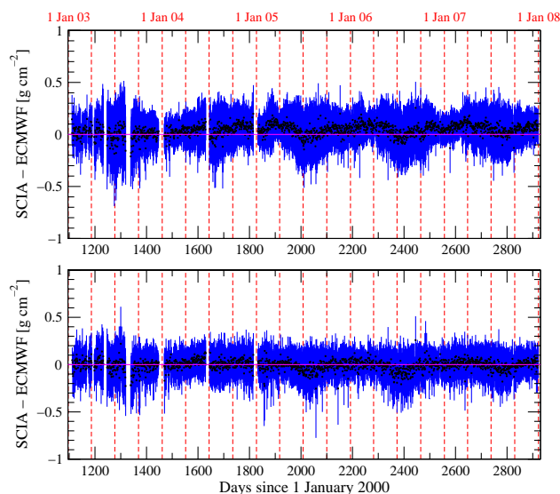
Fig. 13. Daily mean (black) and standard deviation (blue) of difference between SCIAMACHY retrieved water vapour columns and values derived from collocated ECMWF humidity data. Upper panel: all observations. Lower panel: observations over Sahara and Australia excluded. Red dashed lines separate three-month intervals.
