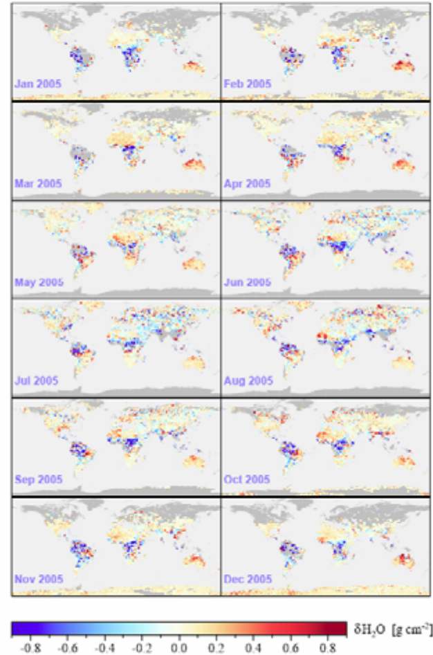
Fig. 7. Monthly averaged differences between SCIAMACHY total water vapour columns and values derived from spatially and temporally collocated ECMWF data for 2005 on a 1^\circ \times 1^\circ grid.
