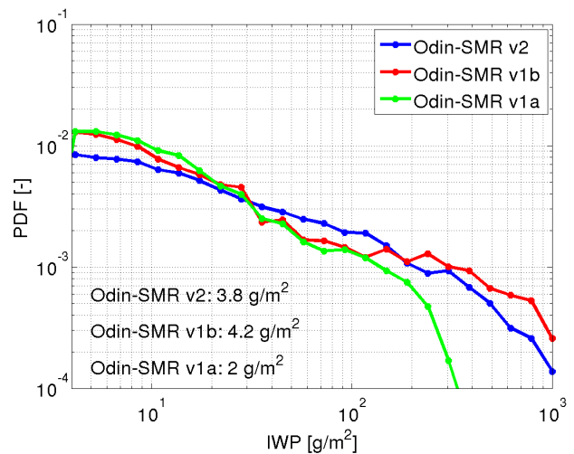
Fig. 12. New Odin-SMR (v2) and previous Odin-SMR (v1) retrieved pIWP. For v1 the PDF of both original data (v1a) and after a correction for cloud inhomogeneity effects (v1b).
