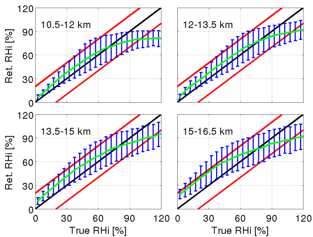
Fig. 7. Statistics for simulated relative humidity retrievals. The green line is the mean retrieved RH for each interval, the vertical bars show the range between the 14 and 86% percentiles (corresponds to \pm 1\sigma ), the black line the one to one line, and the red lines correspond to a 20% RH error.
