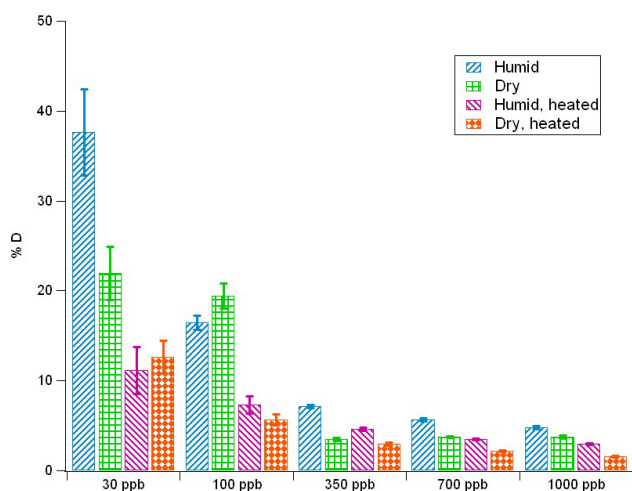
Fig. 5. D-factor illustrates the extent of \text{NH}_3 surface interaction at a range of \text{NH}_3 mixing ratios under conditions of dry and humidified air and using a heated line. The relative contribution of surface interactions is higher at lower mixing ratios, under humid conditions and without the use of a heated line. Error bars indicate one standard deviation.
