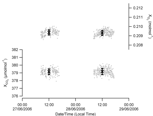
Fig. 3. X_{\text{CO}_2} (left axis) and X_{\text{O}_2} (right axis) filtered for solar intensity variation and retrieval error, and corrected for airmass dependence on the 27 and 28 June 2006. The crosses with error bars represent the mean \pm standard deviation of each day's measurements.
