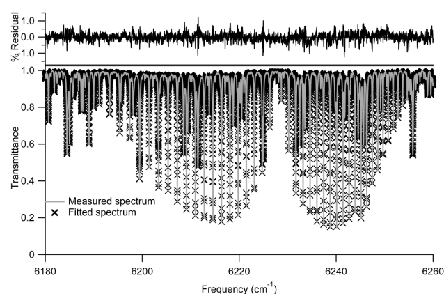
Fig. 2. An example measured (grey) and fitted (black crosses) spectrum in the CO 2 6228 cm -1 band, along with the percentage residual difference (black – upper panel) between the two spectra. This particular spectrum was measured on 20 December 2005 at a solar zenith angle of 12 deg.
