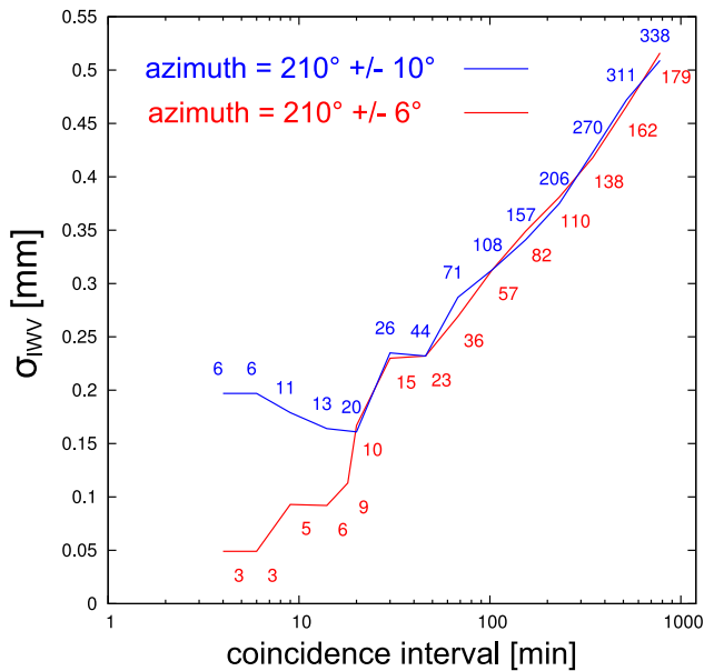
Fig. 3. The standard deviation of differences between DIAL and FTIR IWV values \sigma_{IWV} as a function of the length of the coincidence interval. Only FTIR measurements within an azimuth interval of 210^\circ \pm 6^\circ were taken into account for the lower curve, while the upper curve is for an increased azimuth interval ( 210^\circ \pm 10^\circ ). The numbers of coincident pairs are shown next to both curves.
