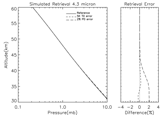
Fig. 8. Same as Fig. 7 but for pressure.
