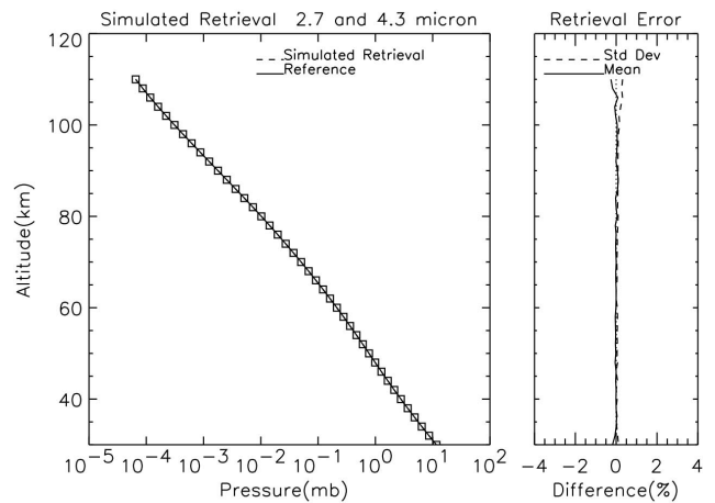
Fig. 20. Same as Fig. 19 but for pressure.
