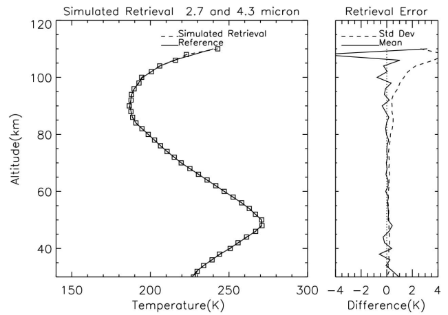
Fig. 19. Temperature results using a two-channel retrieval to overcome lower boundary error of 2% in pressure and 5 K in temperature. Right-hand panel shows the mean error and error standard deviation due to 10^{-5} random measurement error on broadband averaged transmittance.
