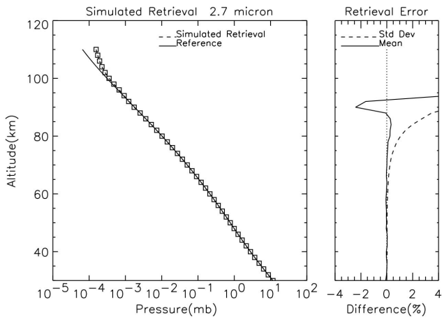
Fig. 14. Same as Fig. 13 but for pressure.
