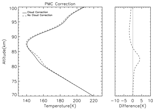
Fig. 28. Impact of PMC correction, right-hand panel shows the difference.
