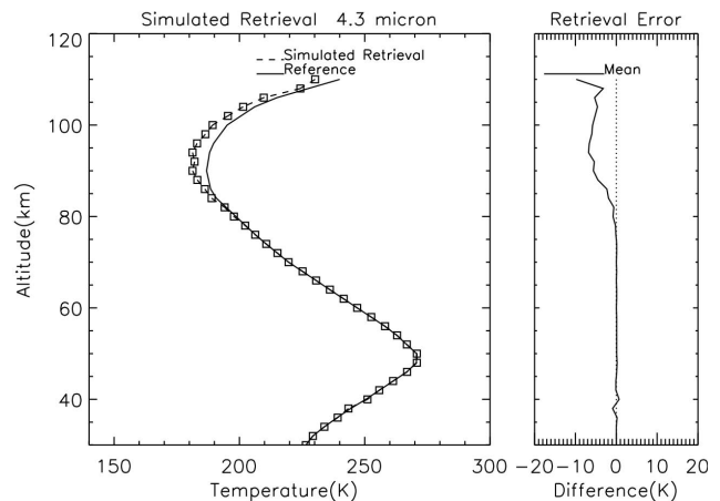
Fig. 17. Impact on the retrieved temperature profile of using the \text{CO}_2 mixing ratio error shown in Fig. 18. Right-hand panel shows the error in retrieved temperature.
