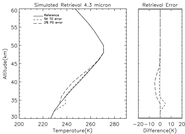
Fig. 7. Effect of lower boundary (34 km) temperature and pressure errors on temperature retrieved from 4.3 \mu\text{m} \text{CO}_2 . Solid lines are retrievals without boundary layer error, and dashed lines are retrievals with incorrect boundary layer conditions. Right-hand panel shows the errors.
