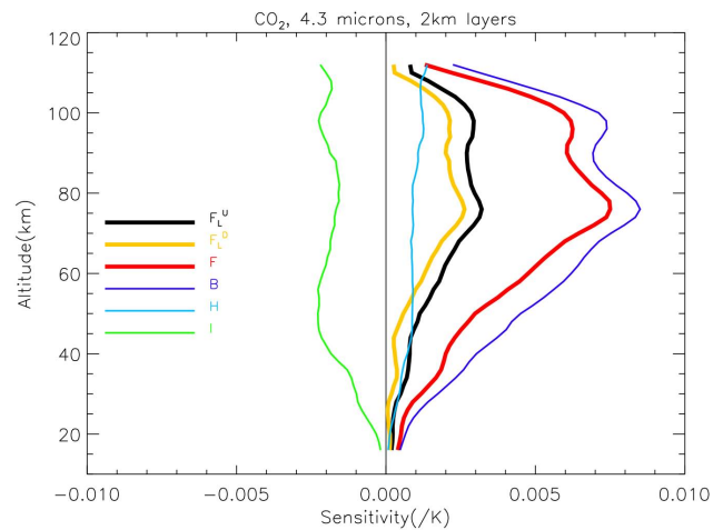
Fig. 3. F_L^U – Sensitivity of 4.3 \mu m CO_2 limb path extinction to 1 K change at the tangent altitude, keeping layers below fixed. F_L^D – Sensitivity to 1 K change at the tangent point, keeping layers above fixed. F – Sensitivity to 1 K change in all layers at or above the tangent altitude, keeping layers below fixed. B – Sensitivity due to temperature used for line strength and broadening. H – Sensitivity due to impact on hydrostatic pressure (hydrostatic equilibrium maintained at all altitudes). I – Sensitivity due to impact of the ideal gas law. Sensitivity is defined as the fractional change of broadband extinction through a perturbed atmosphere relative to unperturbed. In the case of F , the perturbation is a 1 K change to all layers from the tangent point upwards. For all others, the perturbation is a 1 K change to the tangent layer alone.
