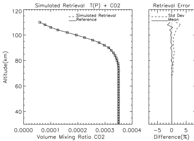
Fig. 24. Same as Fig. 23 but retrieved \text{CO}_2 mixing ratio profile.
