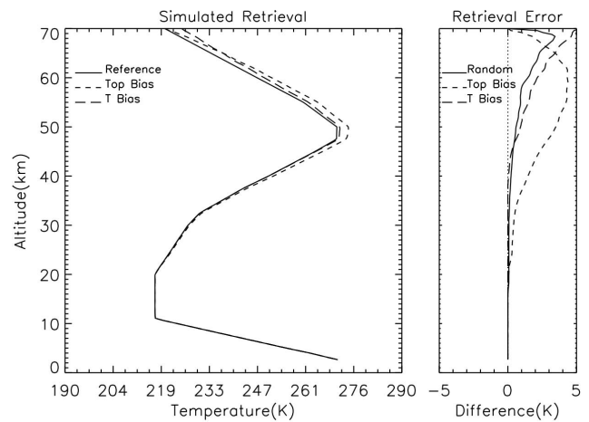
Fig. 25. Impact of random pointing errors and top boundary errors on retrieved temperature, long dashed line shows impact of 5 K upper boundary temperature error, short dashed lines shows impact of 5 % upper boundary error on refraction angle. Right-hand panel shows the errors, solid line in right-hand panel shows impact of random pointing error of 0.02 arc sec.
