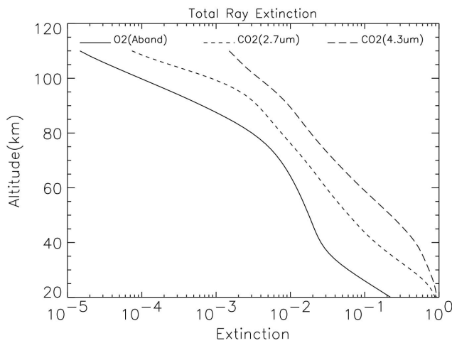
Fig. 2. Broadband limb-path extinction profiles for the 760 nm O_2 A-band and 2.7 and 4.3 \mu m CO_2 . Extinction is defined as (1 - \bar{\tau}_S) .
