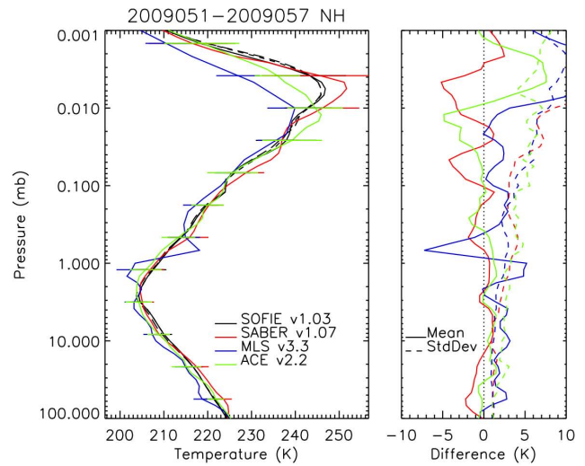
Fig. 31. Comparison between mean SOFIE (black), SABER (red), ACE (green), and MLS (blue) profiles for coincident Northern Hemisphere (NH) data for the period 20–26 February 2009, left-hand panel shows the mean profiles, right-hand panel shows the mean difference and difference standard deviation profiles (SOFIE – each of the others).
