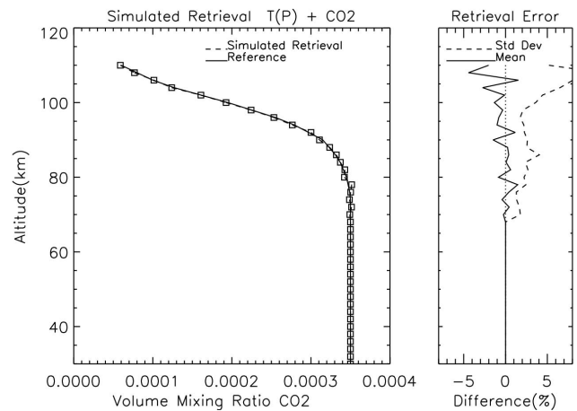
Fig. 22. Same as Fig. 21 but retrieved \text{CO}_2 mixing ratio profile.
