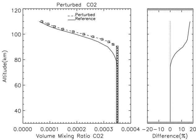
Fig. 18. CO 2 mixing ratio error. Right-hand panel shows the % error.
