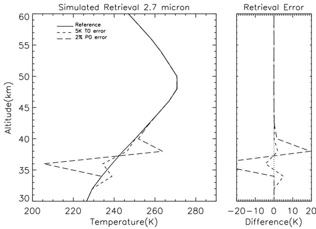
Fig. 9. Same as Fig. 7 but for the 2.7 \mu\text{m} \text{CO}_2 band.
