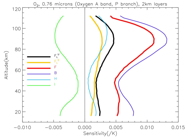
Fig. 6. Same as Fig. 5 but using only the weaker part of the P-branch of the \text{O}_2 A-band.
