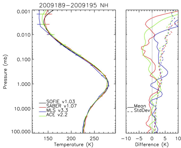
Fig. 30. Comparison between mean SOFIE (black), SABER (red), ACE (green), and MLS (blue) profiles for coincident Northern Hemisphere (NH) data for the period 8–14 July 2009, left-hand panel shows the mean profiles, right-hand panel shows the mean difference and difference standard deviation profiles (SOFIE – each of the others).
