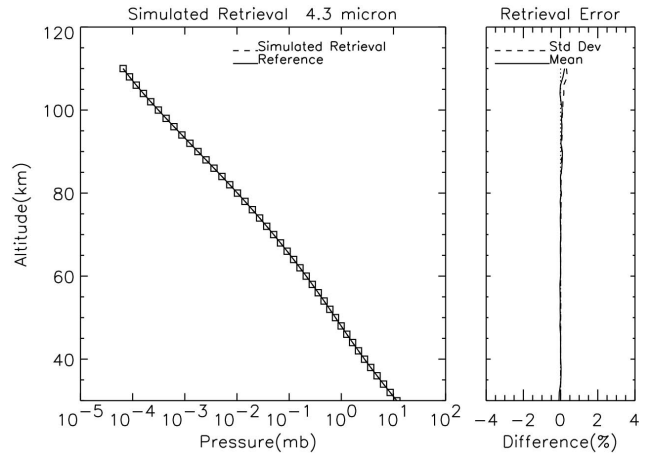
Fig. 12. Same as Fig. 11 but for pressure.
