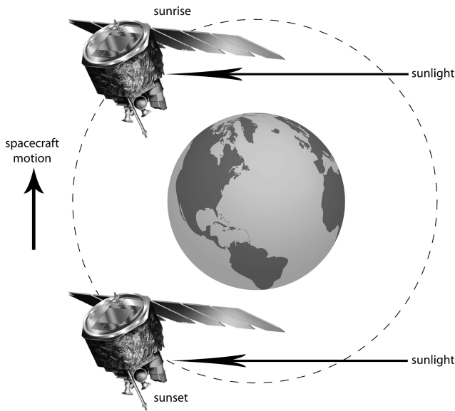
Fig. 1. Solar occultation geometry.
