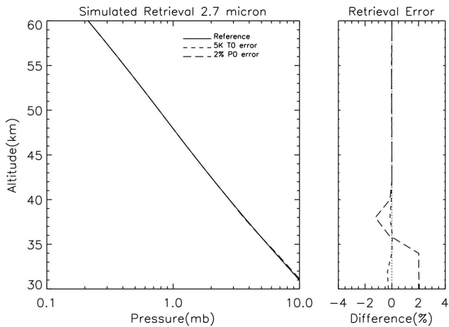
Fig. 10. Same as Fig. 9 but for pressure.
