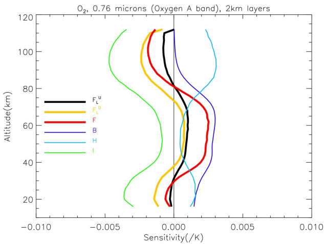
Fig. 5. Same as Fig. 3 but for \text{O}_2 A-band.
