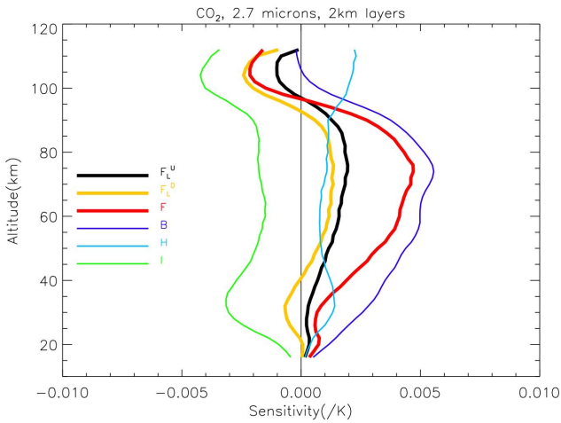
Fig. 4. Same as Fig. 3 but for the 2.7 \mu\text{m} \text{CO}_2 band.
