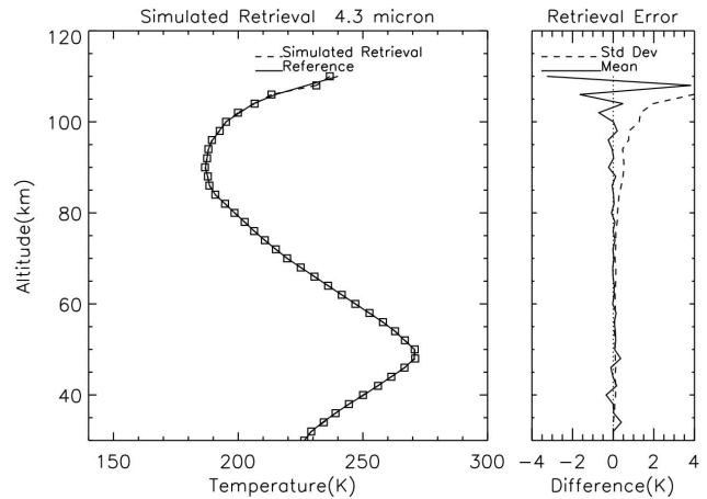
Fig. 11. Simulated temperature retrieval results for the 4.3 \mu\text{m} \text{CO}_2 band. Right-hand panel shows the mean error and error standard deviation due to 10^{-5} random measurement error on broadband averaged transmittance.
