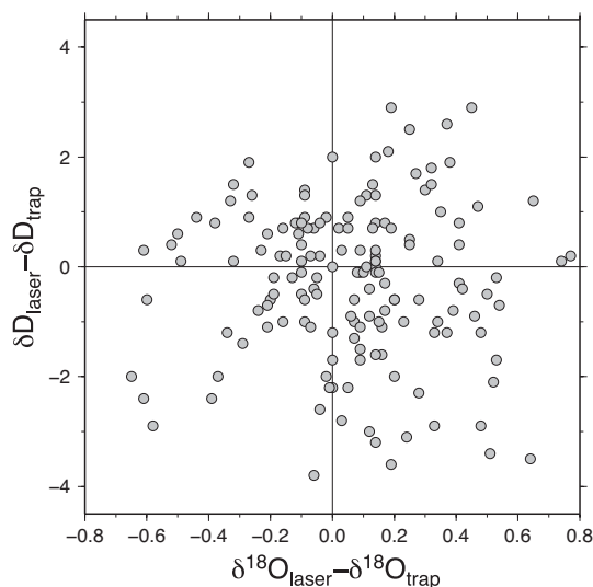
Fig. 10. Comparison of \delta D and \delta^{18}O of water vapor collected via the cold trap method and directly measured using the WVIA. For improved comparison, the time-averaged isotopic values of WVIA measurements during vapor trapping periods are plotted.
