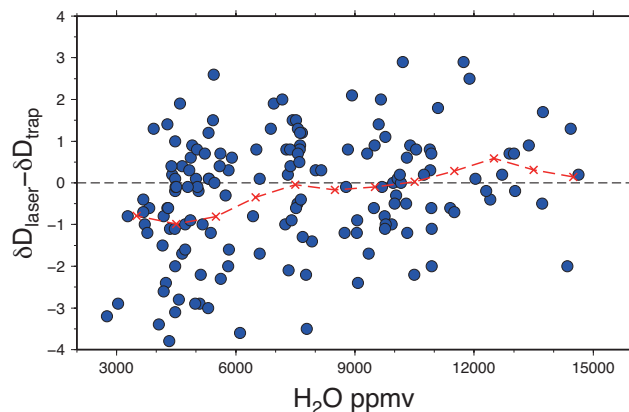
Fig. 9. The same as Fig. 8b, but for \delta\text{D} values.
