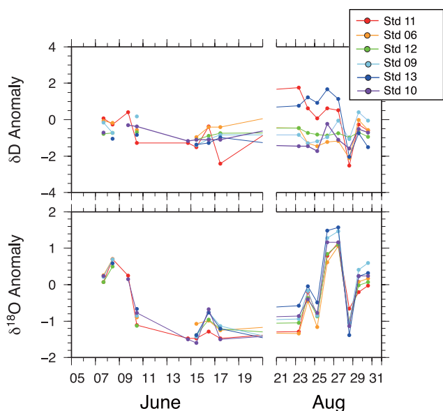
Fig. 5. Comparison of time-dependent \delta D and \delta^{18}O variations of six water standards with different isotopic compositions. Plotted values are expressed as a normalized anomaly, that is, a departure from the long-term mean for the analysis period, divided from the standard deviation during this period.
