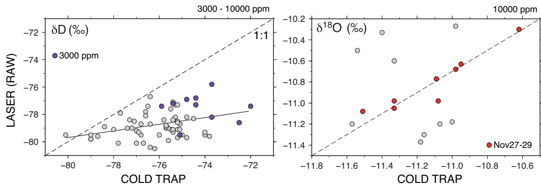
Fig. 3. A comparison of cold trap vapor analysis with direct vapor measurement using the WVIA: (a) \delta\text{D} in a concentration range of 3000–10 000 ppm; the purple points represent values at 3000 ppm; and (b) \delta^{18}\text{O} at 10 000 ppm only; the red plots represent data from 27–29 November 2011. Broken lines represent the 1 : 1 relationship. These WVIA measurements are the uncorrected and uncalibrated \delta\text{D} and \delta^{18}\text{O} values.
