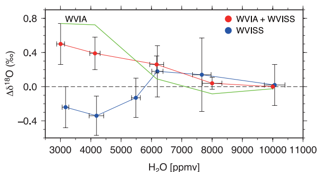
Fig. 7. \delta^{18}O anomaly with changing water vapor concentrations. Anomalies are calculated by subtracting the mean value at 10 000 ppm from measured values at a given water vapor concentration. Error bars show the standard deviation of repeated experiments. The WVISS was run with different water vapor concentrations and the resultant vapor was measured with the WVIA (red line). To escape from the influence of WVIA temporal drift, this experiment was completed within a 30 min time frame after starting calibration. Moisture from WVISS exhaust air was collected using the cold trap system and analyzed off line (blue). To collect a sufficient amount of water for isotope analysis, vapor trapping continued more than two hours. A large spread in the error bar at each vapor concentration may result from isotopic changes in WVISS-generated air and analytical error. Humidity bias stemming solely from the WVIA (green line) was calculated by subtracting the mean values of water vapor generated by the WVISS from WVIA-measured values at a given water vapor concentration.
