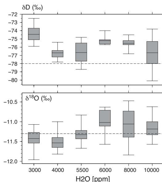
Fig. 2. Analytical variations in the \delta\text{D} and \delta^{18}\text{O} of cold trapped vapor sampled from a WVISS exhaust line with different \text{H}_2\text{O} concentrations. Repeated analysis of standard water ( \delta\text{D} = -78\text{‰} and \delta^{18}\text{O} = -11.3\text{‰} ) was run at 6 levels of vapor concentration from 3000 to 10 000 ppm. The broken line represents known isotopic values determined via IRMS measurement. The box and whisker plots of \delta^{18}\text{O} data represent the median (dark bar), 25–75% quantile range (inter-quantile range [IQR] shown as the box), and maximum and minimum values (whiskers) for repeated experiments.
