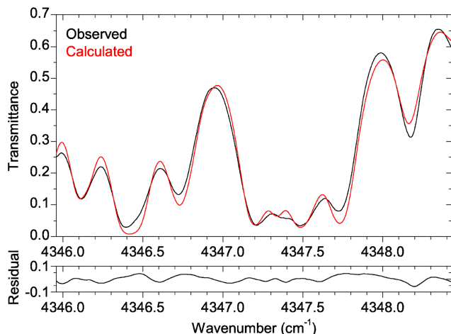
Fig. 1. Observed and calculated atmospheric transmittance spectra in the CH 4 region. All features arise from CH 4 .
