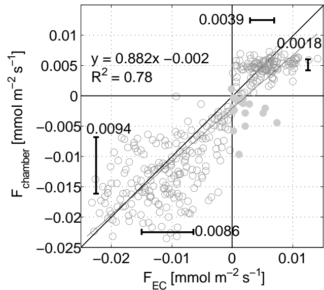
Fig. 1. Scatterplot of EC- and chamber-determined NEE: light grey filled circles represent CO 2 fluxes with opposite directions, and black bars show interquartile ranges of EC/chamber CO 2 source and sink fluxes, respectively (opposite CO 2 fluxes excluded).
