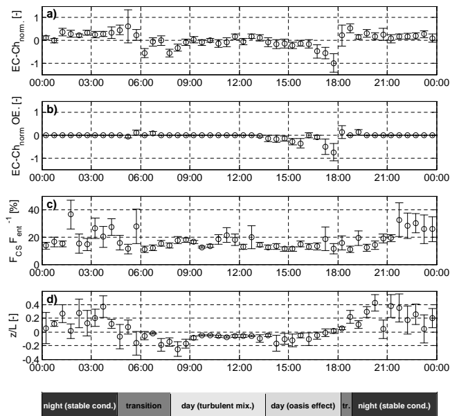
Fig. 2. Mean diurnal cycles of (a) normalized EC–chamber \text{CO}_2 flux differences, (b) normalized EC–chamber \text{CO}_2 flux differences during times with oasis effect (OE), (c) absolute proportion of fluxes by coherent structures and (d) the stratification defined by the stability parameter z/L ( z : height, L : Obukhov length); the bars below indicate different regimes of atmospheric mixing during the day; incoming shortwave radiation reaches 80 \text{ W m}^{-2} at 05:30 and finally at 19:00; time in CET = UTC + 1; error bars indicate variation within the 10-day period.
