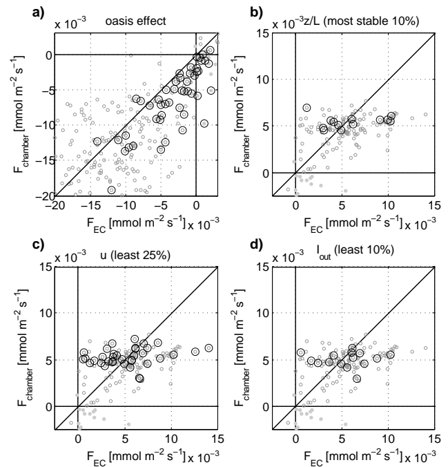
Fig. 3. Scatterplot sections of EC- and chamber-determined NEE under particular micrometeorological conditions: (a) oasis effect; (b) atmospheric stability z/L > 0.7 ; (c) wind velocity u < 0.9 \text{ m s}^{-1} ; (d) outgoing long-wave radiation I_{\text{out}} < 319 \text{ W m}^{-2} – labeled with large black circles in each case; light grey circles represent fluxes with different directions.
