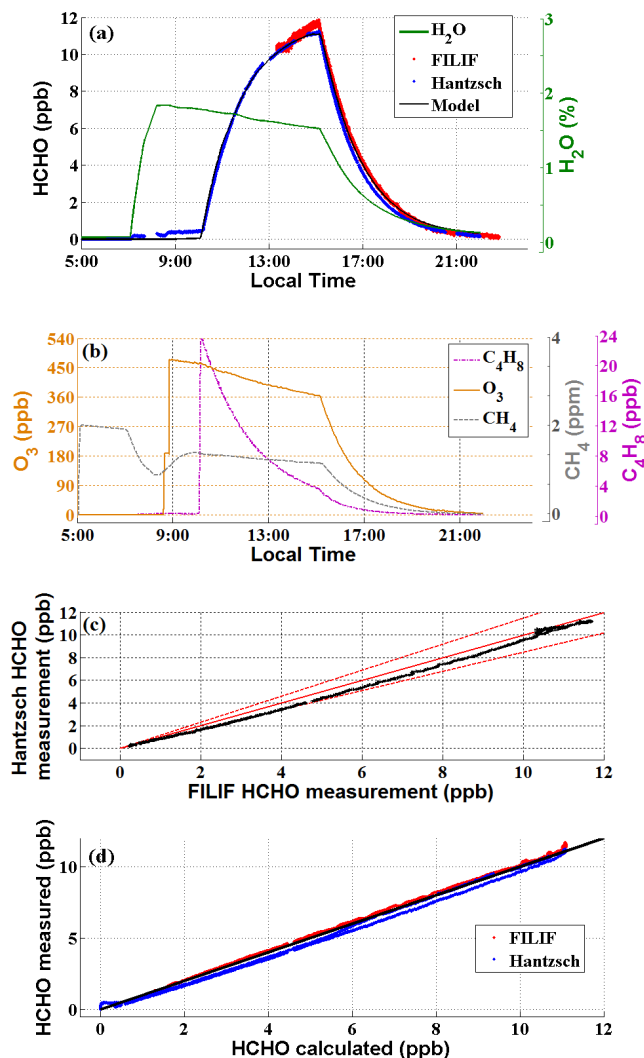
Figure 4. (a) Time series of measured and calculated HCHO mixing ratios and H_2O during day 4. (b) Time series of C_4H_8 , ozone, CH_4 . (c) Comparison between HCHO measurements. Error bars represent 3\sigma precision. Lines represent 1 : 1 agreement and \pm 15\% FILIF measurements. (d) Measurement/model comparison, with the line showing 1 : 1 agreement.
