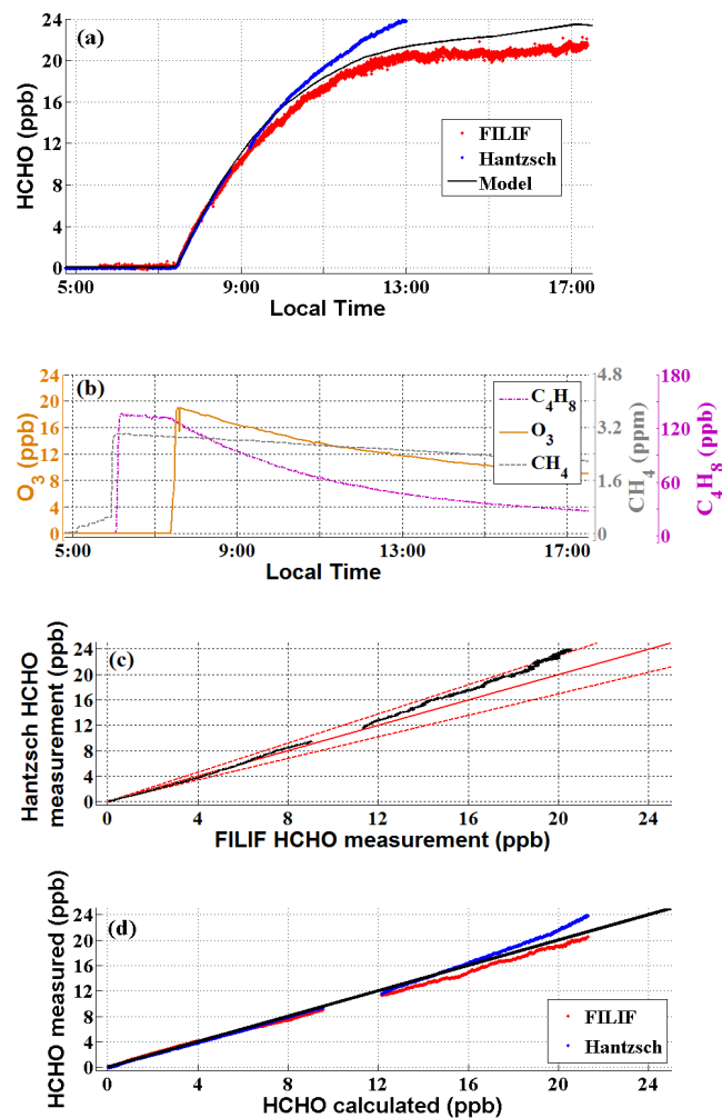
Figure 3. (a) Time series of measured and calculated HCHO mixing ratios during day 3. (b) Time series of C_4H_8 , ozone, and CH_4 . (c) Comparison between HCHO measurements. Error bars represent 3\sigma precision. Lines represent 1 : 1 agreement and \pm 15\% FILIF measurements. (d) Measurement/model comparison, with the line showing 1 : 1 agreement.
