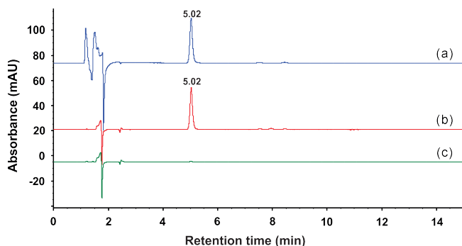
Figure 1. Chromatograms of an aqueous standard containing 0.1 mM guaiacol (a) and guaiacol reaction mixture aliquots quenched by addition of catalase (b) or by drying (c), both sampled at t = 0 min. Chromatographic conditions: isocratic elution, ACN/THF/water (30/4/66, v/v/v ) mixture containing 5 mM ammonium formate buffer pH 3, column: Atlantis T3 ( 3.0 \times 150 mm, 3 \mu\text{m} particle size), flow rate: 0.5 \text{ mL min}^{-1} , column temperature: 30^\circ\text{C} , injection volume: 10 \mu\text{L} , detection: UV (276 nm). The peak eluting at 5.02 min corresponds to guaiacol.
