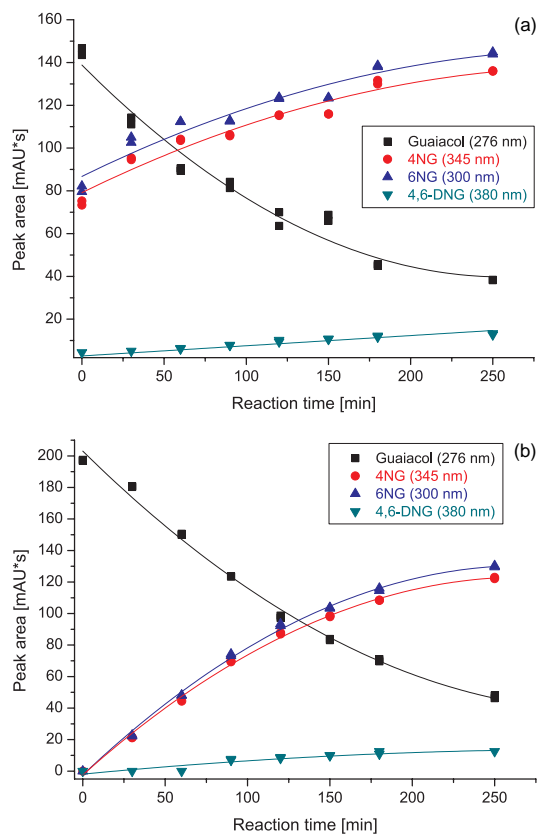
Figure 2. Time evolution of guaiacol, 4-nitroguaiacol (4NG), 6-nitroguaiacol (6NG) and 4,6-dinitroguaiacol (4,6DNG) in the presence of 0.1 mM guaiacol, 1.0 mM \text{H}_2\text{O}_2 and 1.0 mM \text{NaNO}_2 under UV/Vis irradiation. Reaction quenched with 0.01 % catalase (a) and 1 % ascorbic acid (b). Chromatographic parameters are the same as in Fig. 1. The used compound specific detection wavelengths are given in parenthesis after the compounds' names.
