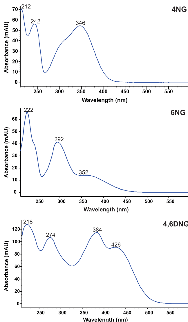
Figure 4. UV/Vis spectra of the main photonitration products of guaiacol. The spectra were collected during analytical HPLC-UV/Vis (DAD) analysis of the nitroguaiacols. Solvent: ACN/THF/water (30/4/66, v/v/v) mixture containing 5 mM ammonium formate buffer pH 3; and temperature: 30 °C.
