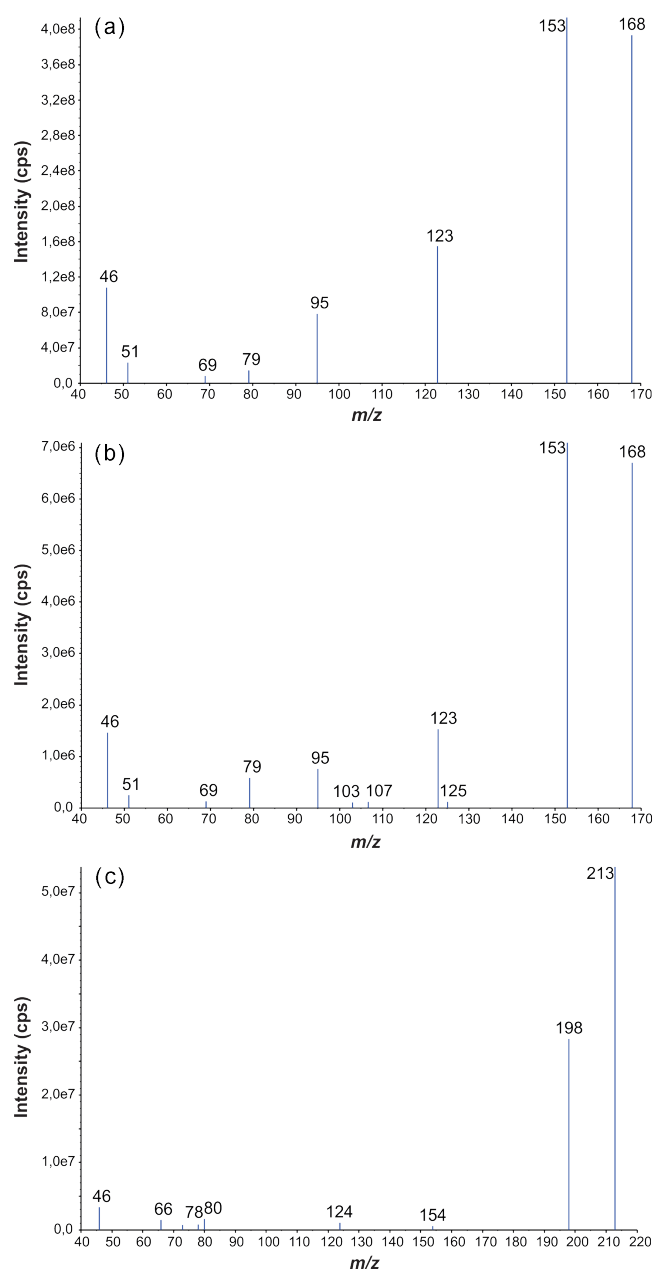
Figure 5. Direct infusion (–)ESI-MS 2 product ion spectra of [M - H]^- for 4-nitroguaiacol (a), 6-nitroguaiacol (b) and 4,6-dinitroguaiacol (c) standards obtained on the 4000 QTRAP instrument.
