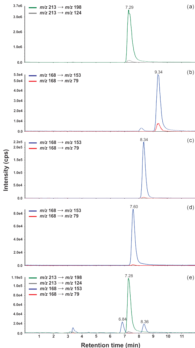
Figure 7. SRM chromatograms for the standards of 4,6DNG ( 270 \mu\text{g L}^{-1} ) (a), 6NG ( 1130 \mu\text{g L}^{-1} ) (b), 4NG ( 150 \mu\text{g L}^{-1} ) (c), 5NG ( 150 \mu\text{g L}^{-1} ) (d), and PM 10 sample (23/12/10) (e). Chromatographic conditions: Atlantis T3 column ( 2.1 \times 150 \text{ mm} , 3 \mu\text{m} particle size); ACN/THF/water = 30/4/66 (v/v/v) mixture containing 5 mM ammonium formate buffer pH 3; flow rate: 0.2 \text{ mL min}^{-1} ; column temperature: 30 \text{ }^\circ\text{C} ; injection volume: 10 \mu\text{L} ; and detection: MS/MS (SRM).
