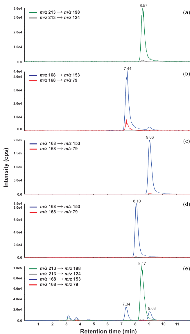
Figure 6. SRM chromatograms for the standards of 4,6DNG ( 270 \mu\text{g L}^{-1} , diluted 1 : 100) (a), 6NG ( 1130 \mu\text{g L}^{-1} ) (b), 4NG ( 150 \mu\text{g L}^{-1} ) (c), 5NG ( 150 \mu\text{g L}^{-1} ) (d), and PM 10 sample (23/12/10) (e). Chromatographic conditions: Atlantis T3 column ( 2.1 \times 150 \text{ mm} , 3 \mu\text{m} particle size); methanol/THF/water = 30/15/55 (v/v/v) mixture containing 5 mM ammonium formate buffer pH 3; flow rate: 0.2 \text{ mL min}^{-1} ; column temperature: 30 \text{ }^\circ\text{C} ; injection volume: 10 \mu\text{L} ; and detection: MS/MS (SRM).
