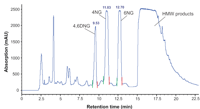
Figure 3. Semi-preparative chromatogram of the guaiacol reaction product extract. Chromatographic conditions: for mobile phase conditions, see Table S1 in the Supplement; column: Atlantis Prep T3 (10 × 250 mm, 5 μm particle size), flow rate: 5 mL min -1 , column temperature: 30 °C, injection volume: 100 μL, detection: UV (300 nm). Green and red lines intersecting the main peaks represent the times of peak collection start and end, respectively.
