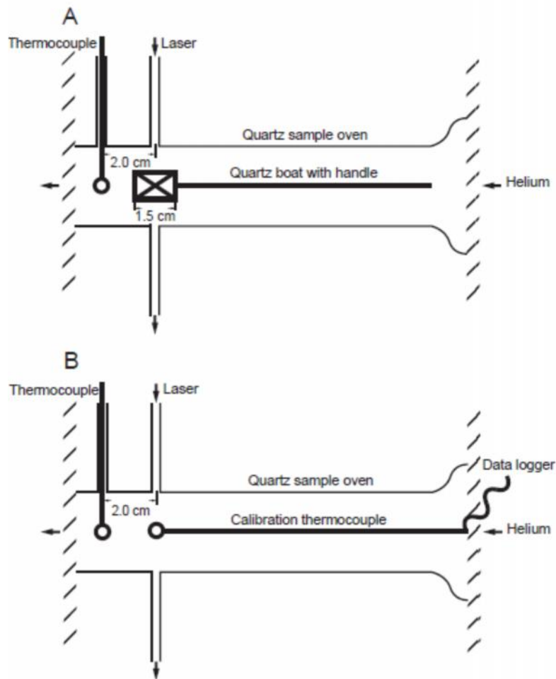
11 Figure S1. The sample analysis set (A) and calibration set (B) of the Sunset Laboratory Carbon Analyzer. 12 Note the position of the oven temperature sensor relative to the filter sample.
