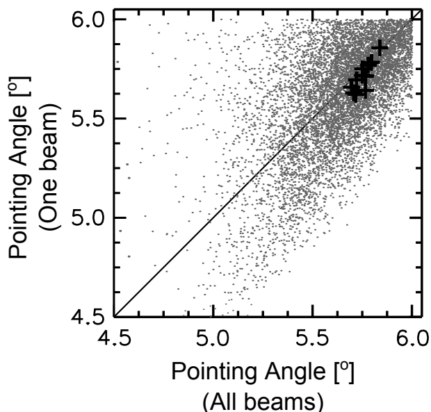
Figure 9. Effective pointing angles derived from 8 weeks of special radar operation, using all 4.2^\circ zenith beams (x axis), and the 252.5^\circ azimuth 4.2^\circ beam (y axis). The grey dots are pointing angles from hourly averages, and the pluses are averages over the whole 8 weeks of operation. The solid line traces the 1:1 points. Only results for every third height gate between 4 and 9 km are shown, to aid interpretation.
