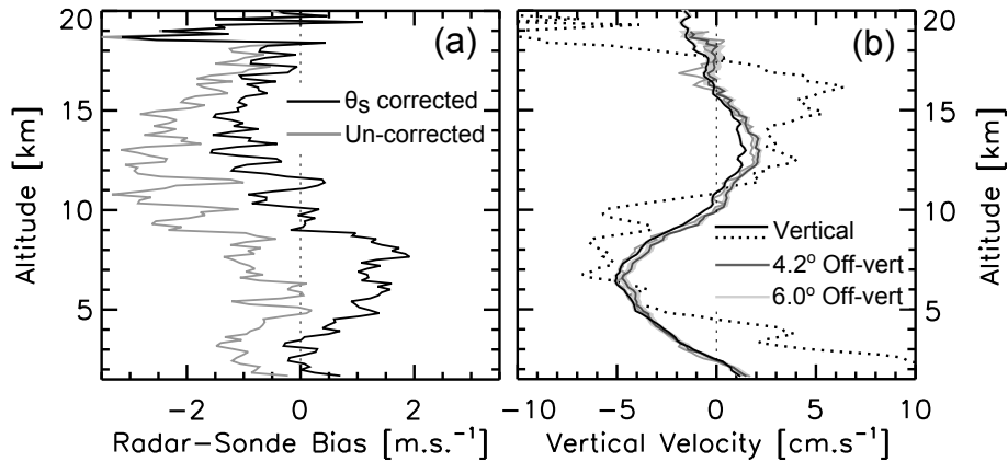
Figure 3. (a) As Fig. 1b but showing radar–radiosonde wind speed bias corrected for aspect sensitivity (black line) and un-corrected (grey line). Error shading has not been included to aid interpretation; the standard error for both curves is as Fig. 1b. (b) Dotted line: vertical velocities from the vertical beam averaged over the radar–radiosonde comparison period. The standard error (not shown) is the width of the solid lines. Solid lines: vertical velocities averaged over the 8 weeks of special operation, from vertical, and complementary off-vertical (4.2 and 6° degree zenith), beams. Shading shows the standard error for the vertical and 4.2° beams. To aid interpretation, the error for the 6° beam is omitted, but it is comparable to that of the 4.2° beam.
