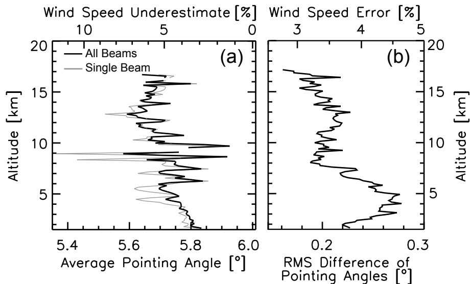
Figure 8. (a) Average effective pointing angles for 6^\circ beams, calculated across the 8 weeks of special operation. Effective pointing angles using one (grey curve), and all (black curve), 4.2^\circ beams are shown. The top axis gives the corresponding underestimate in wind speed. (b) RMS difference in effective pointing angles derived using one and four 4.2^\circ beam echo powers, calculated over the 8 weeks. The top axis gives the corresponding uncertainty in winds corrected with the one-beam method.
