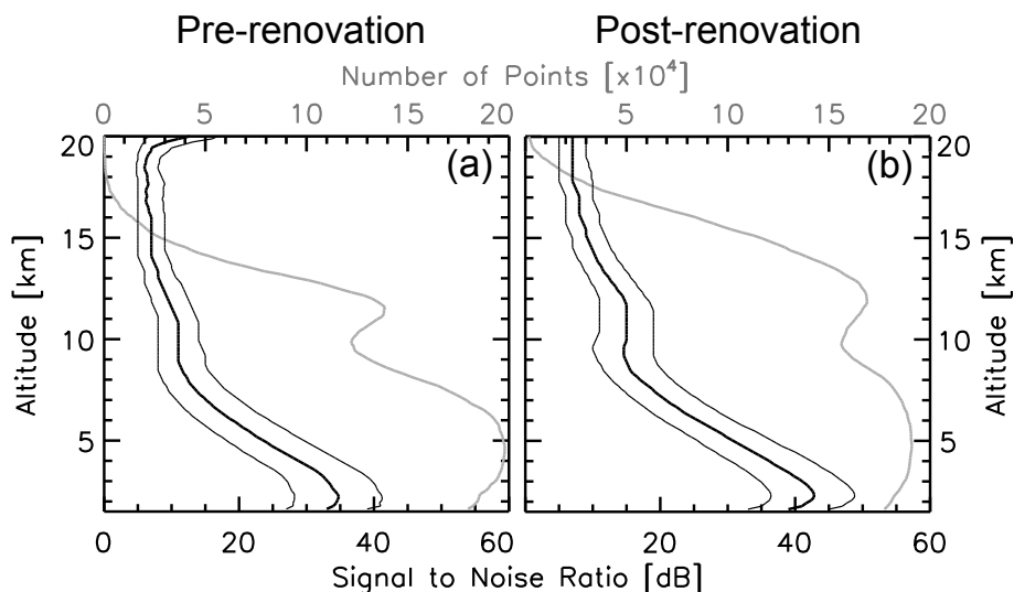
Figure 11. Average SNR (black curves) and the number of reliable ( 6^\circ zenith angle) complementary beam pairs of measurements (grey curves), before and after renovation (panels a and b, respectively). The thin black lines correspond to the upper and lower quartile of the SNR distribution. SNR values shown here are peak signal power spectral density to noise. A whole year of measurements has been used for each figure (2010 and 2012, respectively).
