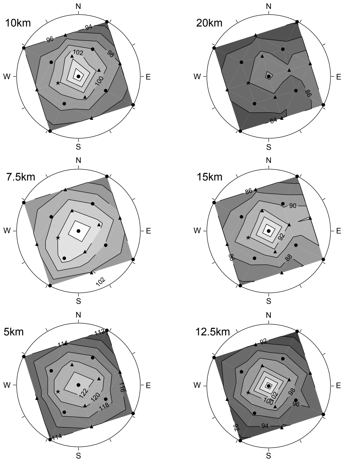
Figure 7. Average echo power maps derived from 8 weeks of special operation. The contours and labels give echo power in decibels. Symbols indicate the location of beams. Circles correspond to the 0, 6, and 12° zeniths; triangles give 4.2 and 8.5° zeniths. The star indicates the 4.2° zenith beam used to calculate aspect sensitivity for routine observations. The range is indicated in each panel.
