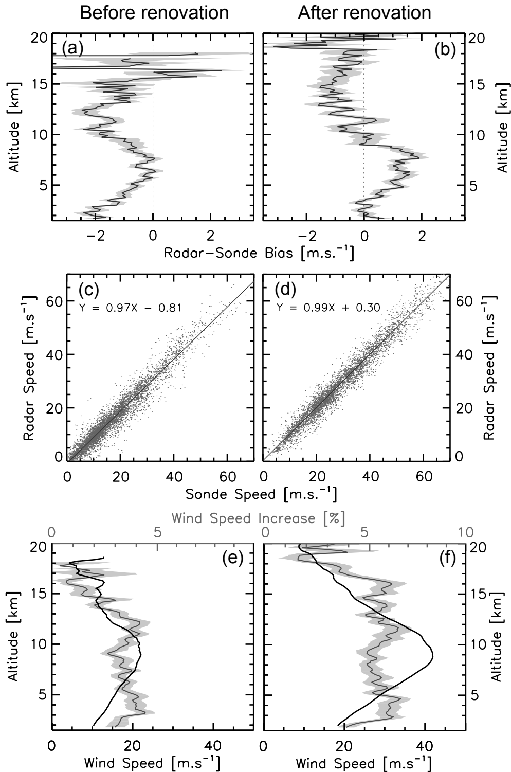
Figure 1. Comparison of wind speeds measured by the MST radar, and 75 and 52 radiosonde launched from the Aberystwyth radar site, pre- and post-renovation, respectively. (a) Average radar–radiosonde wind speed differences at different altitudes, before the renovation. Negative differences correspond to radar speeds smaller than radiosonde speeds. The grey shading shows the standard error. Radar winds have been corrected for aspect sensitivity. (b) As (a) but after the renovation. (c) MST against radiosonde wind speeds at all altitudes. The grey line is a best fit, quantified by the text at the top of the panel. (d) As (c) but after renovation. (e) Average MST radar wind speed (bottom axis and black line) and aspect sensitivity correction (top axis and grey line, with shading giving standard error) for the pre-renovation comparison. (f) As (e) but after renovation.
