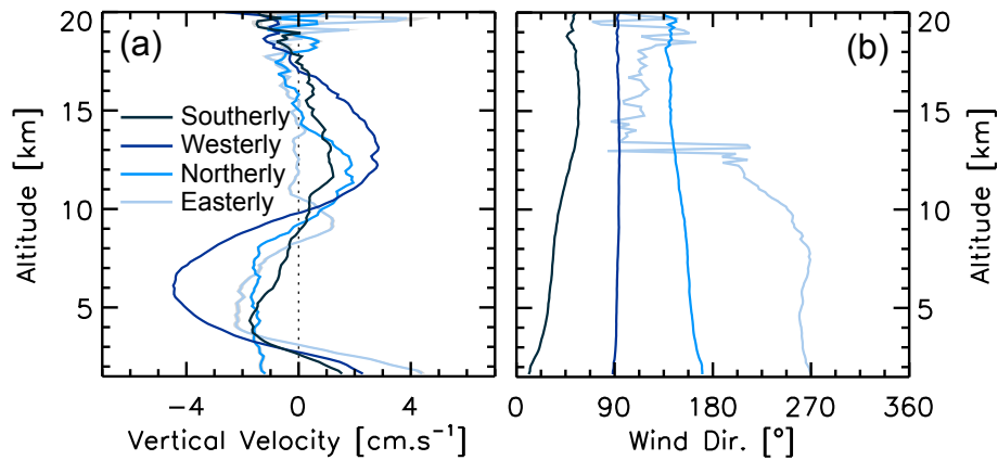
Figure 5. (a) Mean vertical velocities for different 2 km wind directions. 30 months of data from May 2011 have been used. The four curves comprise measurements whose 2 km wind vectors are within 45^\circ of north, south, east and west (indicated in the legend as southerlies, northerlies, westerlies, and easterlies, respectively). Shading gives the standard error, which is often smaller than the line thickness. (b) Mean wind direction in the profile when the direction at 2 km lies in one of the four quadrants.
