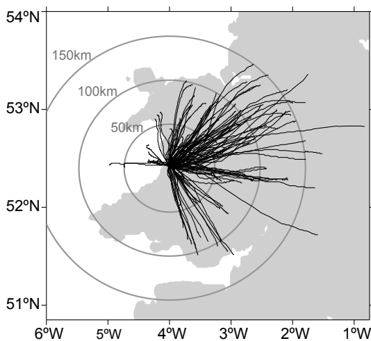
Figure 4. Flight tracks of 127 radiosondes launched from the Aberystwyth radar site. The grey shading indicates the land surface, and 50 km range intervals are shown by the concentric grey circles centred on the radar site. Only the first 21 km of sonde ascent are shown, corresponding to the upper altitude limit of the MST radar.
