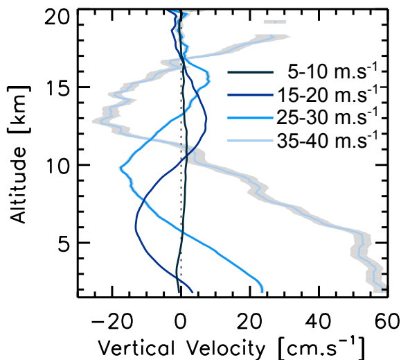
Figure 6. As Fig. 5a but showing the 2 km westerly winds, decomposed into different 2 km wind speeds (shown by the legend).
