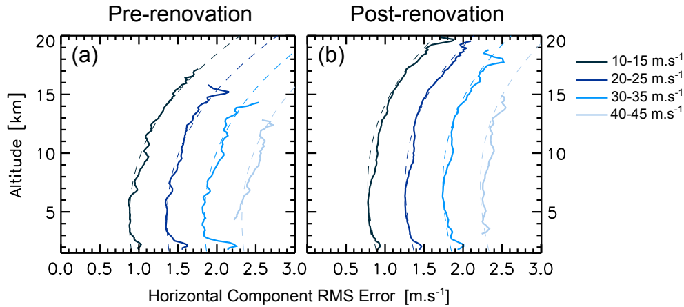
Figure 12. RMSE in horizontal wind components at different horizontal wind speeds. Curves show the combined error from beam separation (Fig. 10), and aspect sensitivity corrections (Fig. 8b) before and after the renovation (panels (a) and (b), respectively). Different shaded curves correspond to the different horizontal wind speeds described in the legend. Pre-renovation and post-renovation curves use all wind directions in 2009 and 2012, respectively. The dashed lines are approximations of the solid lines, calculated with Eq. (A1a) in the Appendix.
