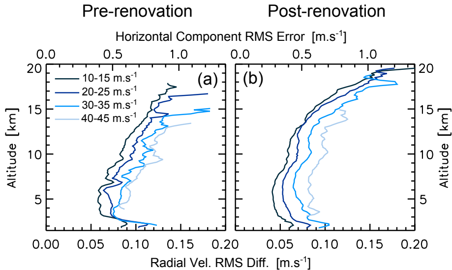
Figure 10. Radial velocity RMS differences at different horizontal wind speeds, before and after the renovation (panels (a) and (b), respectively). RMS values are from the difference of vertical beam and complementary beam vertical velocities, normalised to indicate the error associated with measurements made on a single beam (see text). Different shaded curves correspond to the different horizontal wind speeds described in the legend. The curves are averages of both 6^\circ zenith beam pairs. Pre-renovation and post-renovation curves use all wind directions in 2010 and 2012, respectively. The top axis gives the corresponding RMSE in horizontal wind components.
