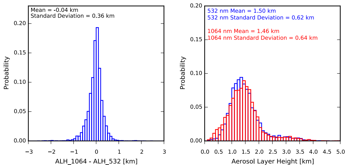
Figure S1. The probability distributions of the of the effective aerosol layer height derived from the 1064 nm and 532 nm CALIOP aerosol extinction vertical profile observations and their difference
