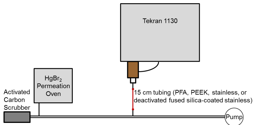
Figure S1. Diagram of manifold for testing transmission of \text{HgBr}_2 through tubing materials.
