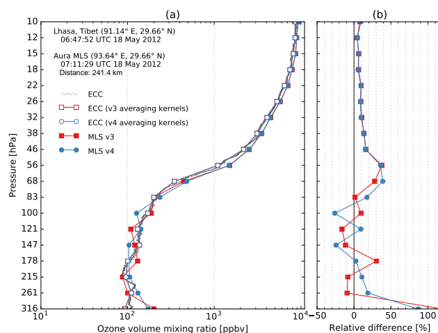
Figure 10. As in Fig. 3, but for ECC, MLS v3 and MLS v4 profiles of ozone volume mixing ratio.
