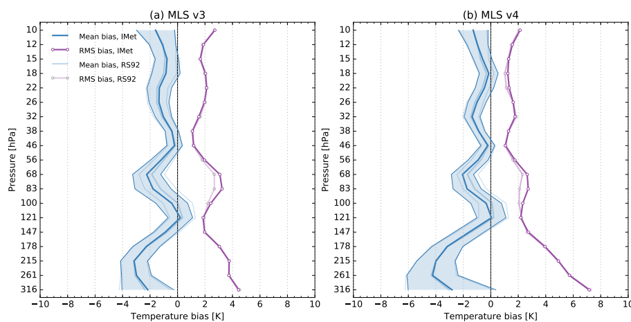
Figure 6. Mean and root mean square biases for (a) MLS v3 and (b) MLS v4 temperature retrievals relative to 17 temperature profiles at Lhasa and Linzhi measured using both InterMet (IMet) and RS92 radiosondes. Uncertainty bounds on the mean bias represent twice the standard error of the mean.
