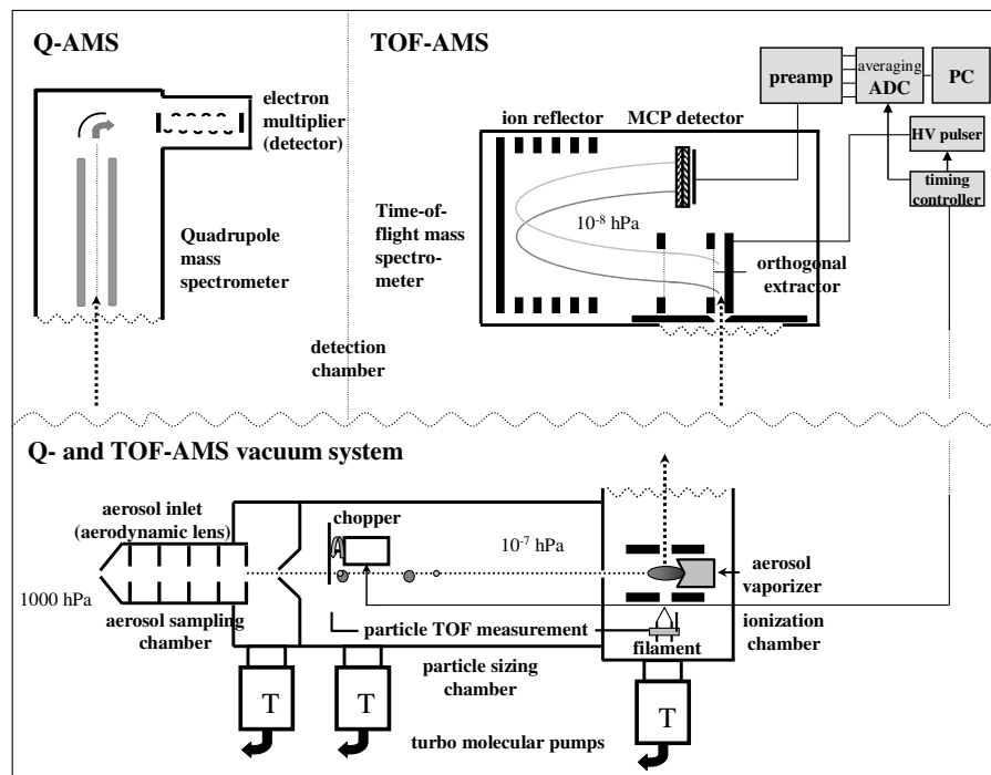
Fig. 1. Schematic diagrams of Q-AMS and ToF-AMS.
