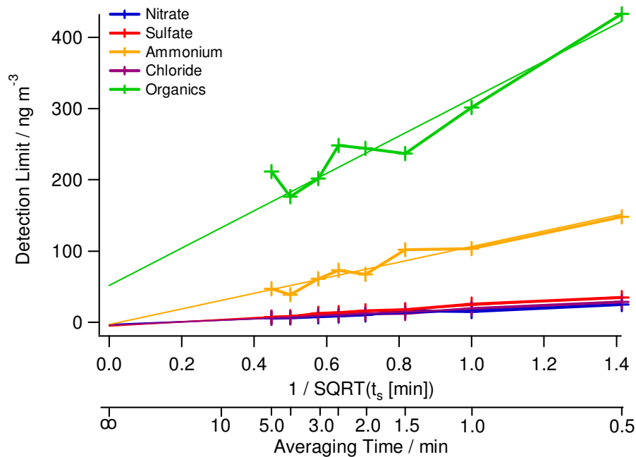
Fig. 5. Q-AMS detection limits for various averaging times plotted versus the inverse square root of the averaging time.
