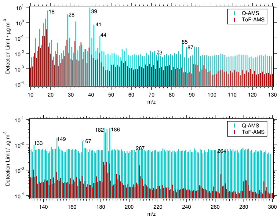
Fig. 2. Detection limits of individual m/z , experimentally determined from 30 seconds blank measurements for Q-AMS (blue) and ToF-AMS (red). The m/z with the highest detection limits are labeled. Note, that the detection limits for the different species (as given in Table 1) are calculated from the noise of that species and are not simply the sum of the DL of the corresponding m/z .
