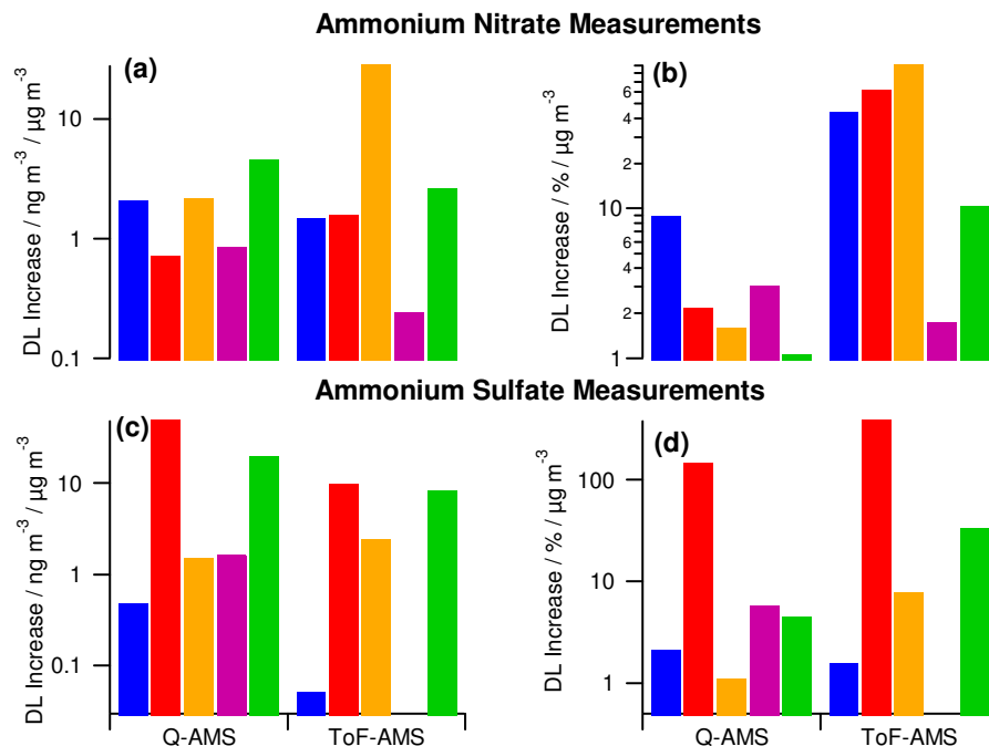
Fig. 3. Influence of increased aerosol mass concentrations on detection limits of the individual species. Upper panels: measurement of ammonium nitrate aerosol; lower panels: measurement of ammonium sulfate aerosol. Left panels: absolute increase in DL levels; right panels: relative increase of DL. Increases are based on \mu\text{g m}^{-3} of nitrate or sulfate for all species besides ammonium. For ammonium they are based on \mu\text{g m}^{-3} of ammonium measured.
