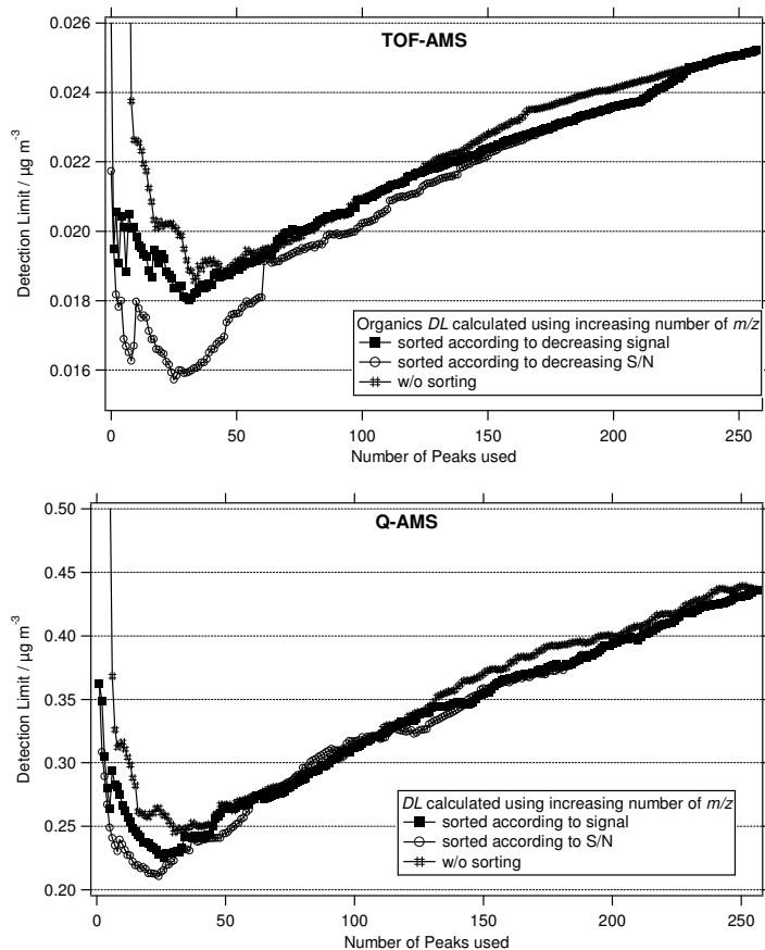
Fig. 6. (a) ToF-AMS and (b) Q-AMS DL from filter measurements, calculated using an increased number of selected m/z after different ways of sorting the signals. The lowest DL is achieved for the first 24–25 peaks with the largest S/N ratio.
