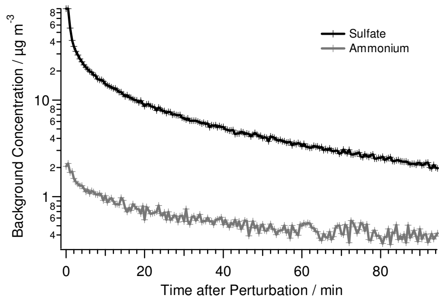
Fig. 4. Decay of Q-AMS sulfate and ammonium signal background after perturbation with 140 \mu\text{g m}^{-3} ammonium sulfate aerosol.
