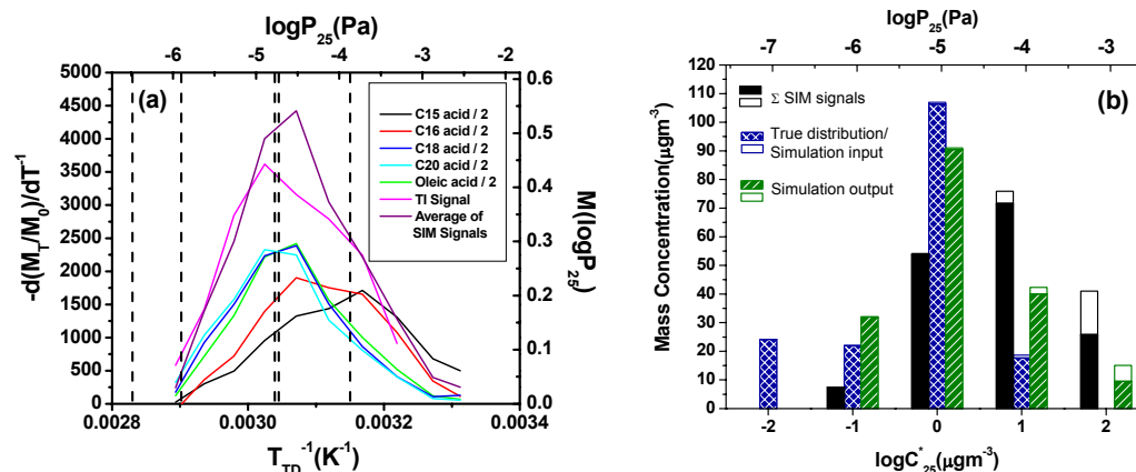
Fig. 9. (a) \log P_{25} distribution for a mixture of C_{15} , C_{16} , C_{18} , and C_{20} monoacids and oleic acid in mole ratios of 1:1:1:4. The fragments monitored in SIM mode for the individual components in the mixture were: pentadecanoic acid, m/z 242; hexadecanoic acid, m/z 256; octadecanoic acid, m/z 284; eicosanoic acid, m/z 312; oleic acid, m/z 264. For clarity, the curves for the individual SIM profiles were scaled by a factor of 1/2. The vertical lines are the averaged literature P_{25} values shown in Table 2 for each compound. (b) Volatility distribution for the mixture of C_{15} , C_{16} , C_{18} , and C_{20} monoacids and oleic acid showing calculated gas-particle partitioning. Filled and empty areas of the bars indicate particle phase and gas phase material, respectively. The experimental distribution was calculated from the mass fraction weighted average of the SIM profiles. The true distribution was calculated from the mass fractions of the components in the mixture and the literature values of P_{25} shown in (a).
