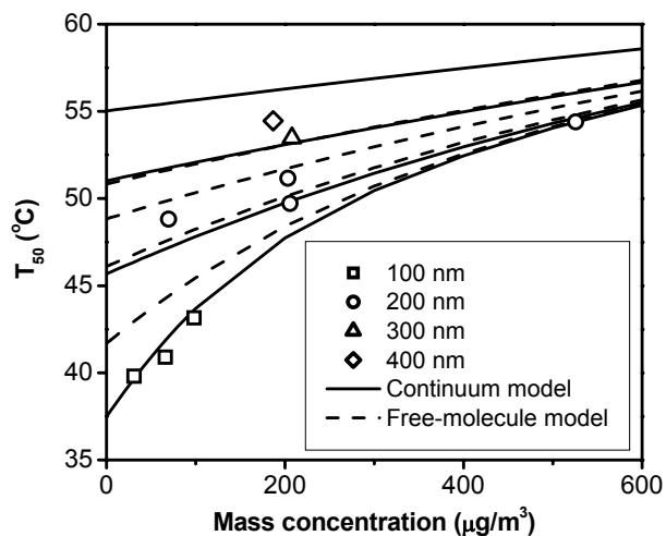
Fig. 7. Measured and simulated values of T_{50} vs. particle mass concentration for 100, 200, 300, and 400 nm diameter oleic acid particles.
