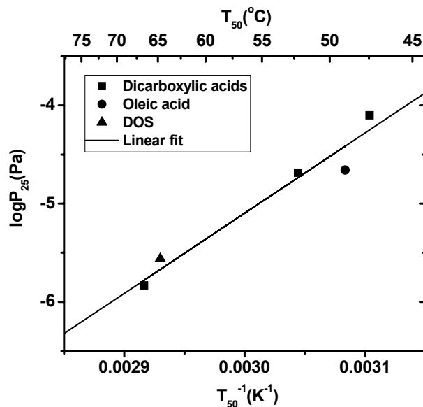
Fig. 5. \log P_{25} vs. T_{50} calibration plot. The T_{50} values were calculated as described in the text using 200 nm diameter particles and mass concentrations of 100–200 \mu\text{g m}^{-3} .
