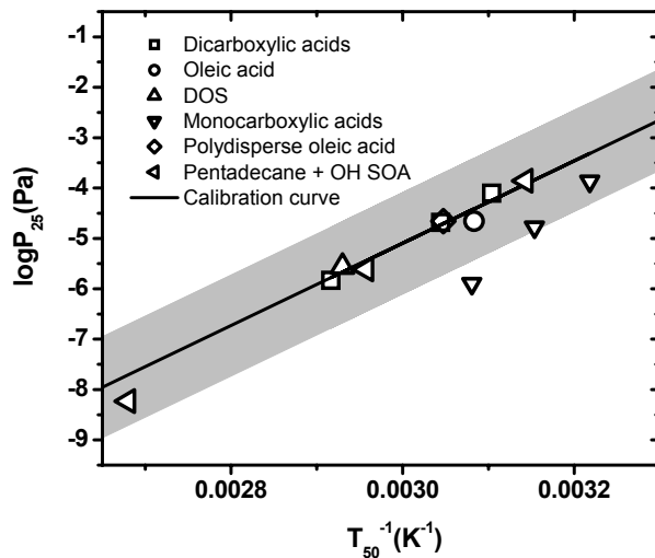
Fig. 6. \log P_{25} vs. T_{50} for various aerosols used in this study. The shaded region indicates the region \pm 1 order of magnitude in P_{25} from the calibration curve.
