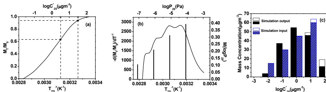
Fig. 8. Calculation of volatility distributions from the TD vaporization profile. (a) Simulated TD vaporization profile for a mixture of 4 compounds with saturation concentrations of 10^{-2} , 10^{-1} , 10^0 , and 10^1 \mu g m^{-3} at 25^\circ C . The \log P_{25} distribution, M(\log P_{25}) , shown on the right axis in (b) is calculated by taking the derivative of M_T/M_0 with respect to T_{TD}^{-1} (shown on the left axis), converting the x-axis from T_{TD} to \log P_{25} using Eq. (1), and dividing d(M_T/M_0)/d(T_{TD}^{-1}) by the slope in Eq. (1). The vertical bars in (b) indicate the vapor pressures and mass fractions of the compounds used as input for the simulation. The mass fractions of the particle mass concentration belonging to each order of magnitude C_{25}^* bin, necessary for the volatility basis set analysis (c) are calculated by taking the difference between M_T/M_0 at the edges of the bin; the dashed lines in (a) indicate those values for the C_{25}^*=10^1 bin. Filled and empty areas of the bars indicate particle phase and gas phase material, respectively. The distribution shown by solid bars in (c) was calculated from the curve in (a) by this procedure, and the distribution shown by the patterned bars in (c) was used as input for the simulation.
