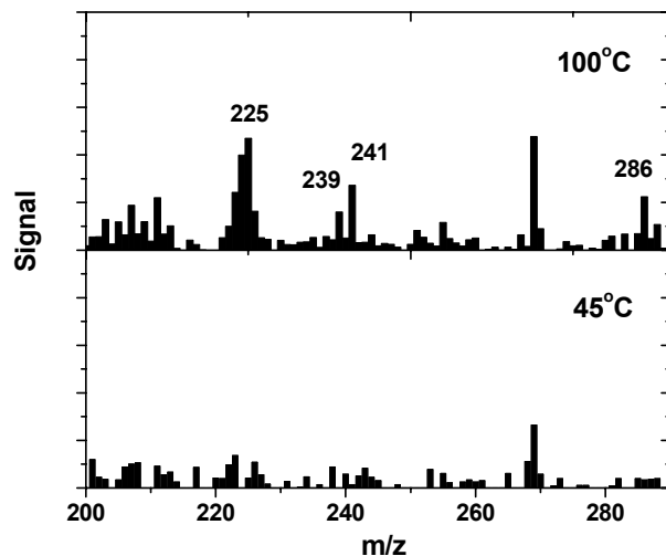
Fig. 12. Mass spectra of material volatilized at 45°C and 100°C from SOA formed from the reaction of pentadecane with OH radicals. The spectra were calculated by subtracting the mass spectrum of aerosol sampled after passing through the TD from that sampled after passing through the TD bypass tube.
