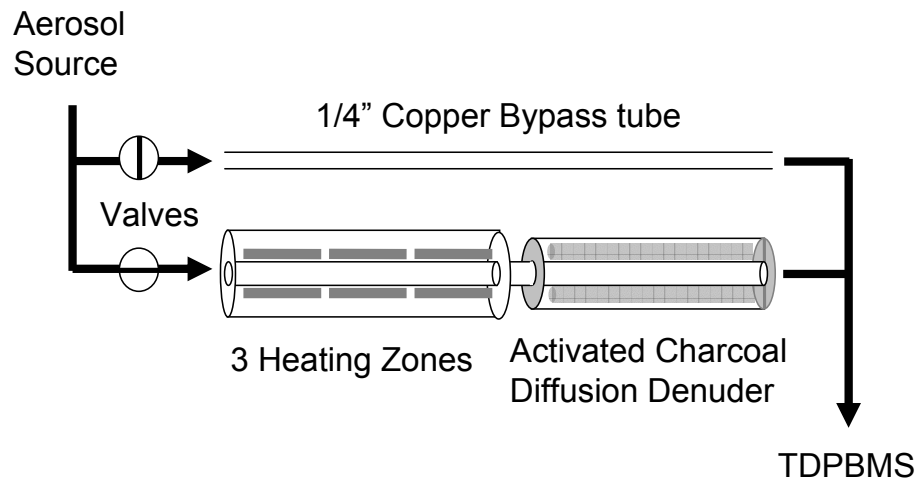
Fig. 1. Schematic of the thermodenuder (TD) system. The aerosol source is either an atomizer/DMA or an environmental chamber.
