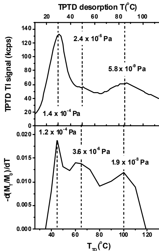
Fig. 10. (top) TPTD desorption profile for laboratory-generated SOA formed from the reaction of pentadecane with OH radicals (Lim and Ziemann, 2005) and (bottom) negative of the derivative of the TD vaporization profile with respect to T_{TD} .
