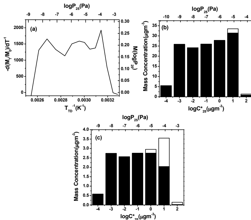
Fig. 11. (a) \log P_{25} distribution and (b) Volatility basis set distribution for laboratory-generated SOA formed from the reaction of pentadecane with OH radicals. (c) Calculated volatility distribution for the same aerosol after 10-fold dilution. Filled and empty areas of the bars in (b) and (c) indicate particle phase and gas phase material, respectively. The particle mass concentration was \sim 150 \mu\text{g m}^{-3} .
