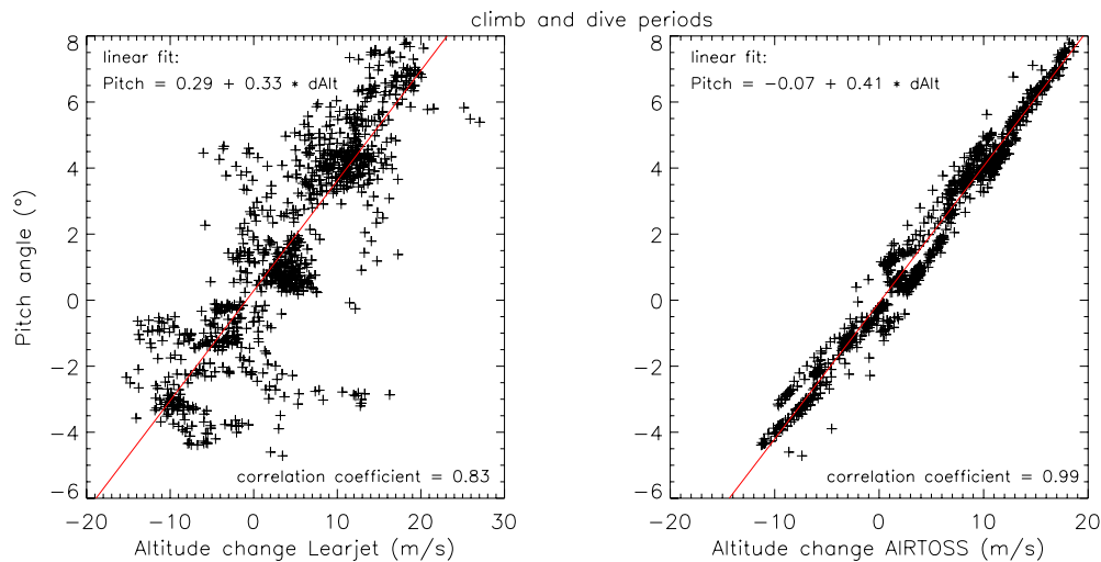
Fig. 8. Correlation between pitch angle and altitude change measured on Learjet (left) and AIRTOSS (right) during climb and dive periods on 6 September 2007.
