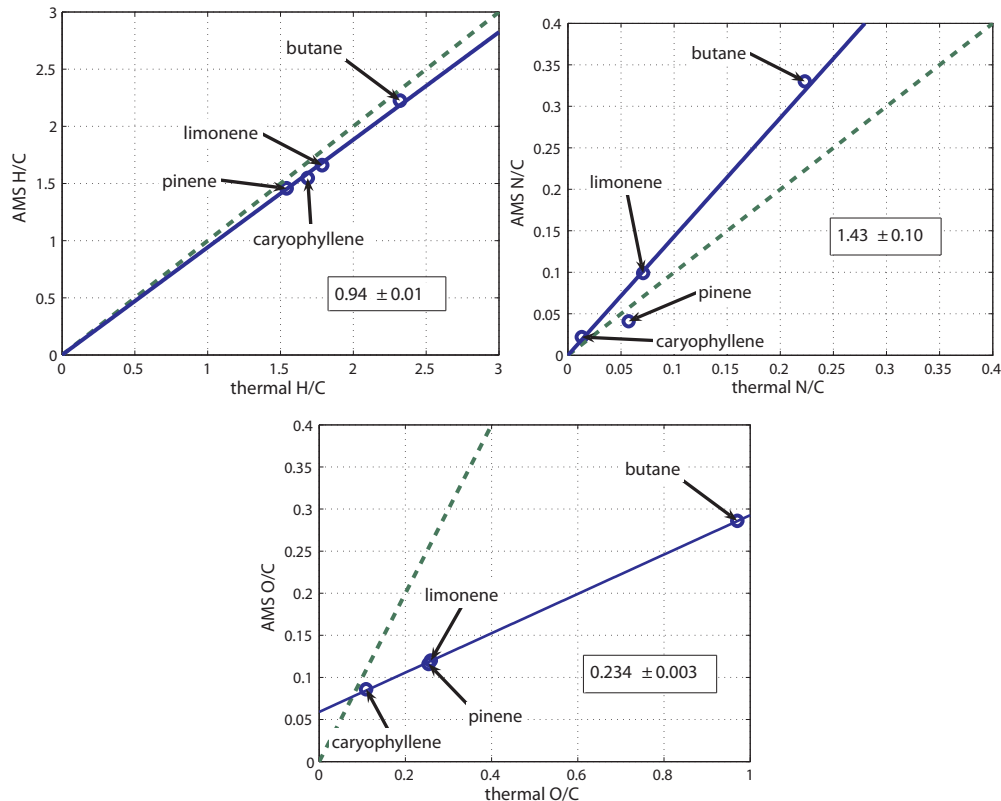
Fig. 3. Comparison of atomic ratios measured with the AMS, to atomic ratios measured by combustion elemental analysis. Here we plot the elemental ratios calculated assuming equal response to CHN and O (corrections to elemental analysis recommended by Aiken et al. (2008) have not been applied to the data). Green dashed line is a 1:1, and solid blue is a linear fit to the data with y-intercept forced to zero.
