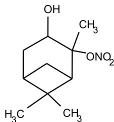
3-hydroxy-pinene-2-nitrate
