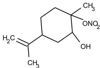
2-hydroxy-limonene-1-nitrate
