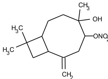
3-hydroxy-caryophyllene-4-nitrate
