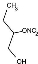
1-hydroxy-butane-2-nitrate
