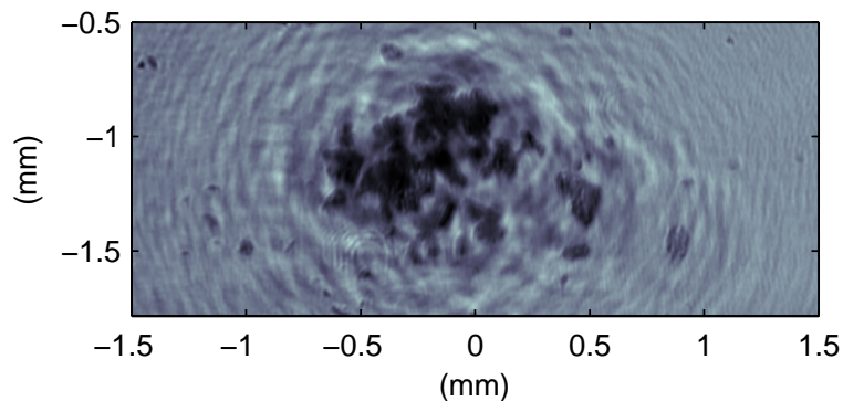
Fig. 2. An ice particle in the process of shattering about 10 mm from one of HOLODEC's windows.
