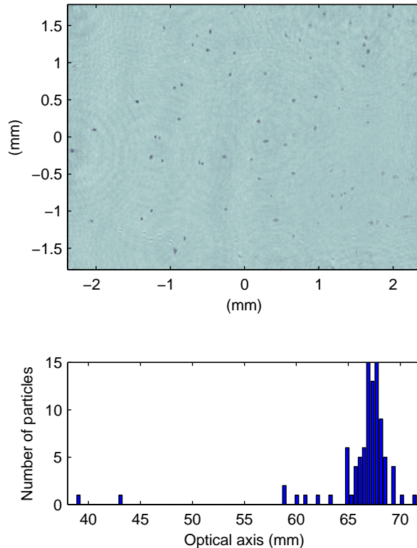
Fig. 1. The top panel shows a hologram from Research Flight 2003-09-17 reconstructed to 66.5 mm. The reconstructed image has many particles in focus at one depth and many others nearly in focus. The bottom panel is a histogram of the z-positions of all particles in the sample volume. This is suggestive of shards of a single impacted crystal tracing an aerodynamic surface about the instrument housing.
