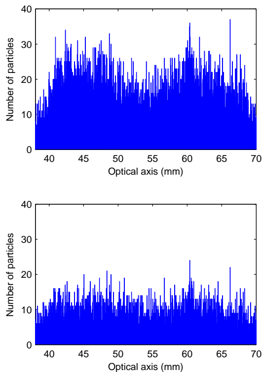
Fig. 3. In the top and bottom panels are histograms of optical-axis positions of particles from Research Flight 2003-09-17. The top panel shows all particles and the bottom panel excludes particles in holograms containing shattered particles. Note that rejecting shattered particles yields a more uniform distribution of particles along the optical axis.
