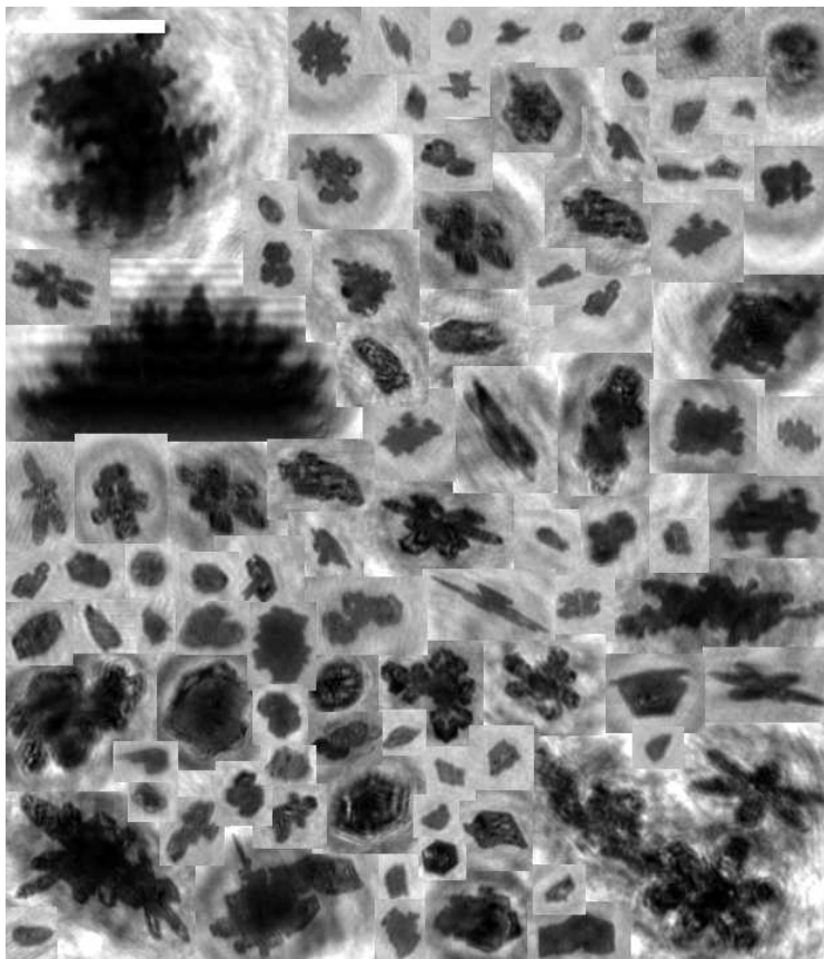
Fig. 10. Reconstructed images of Ice particles larger than 100\ \mu\text{m} in equivalent diameter from Research Flight 2003-09-05. They appear as reconstructed by the automated particle finding algorithm. The white scale bar in the upper left is 0.5 mm in length.
