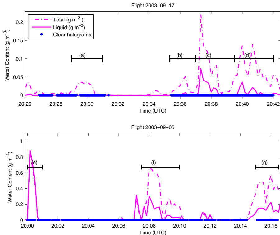
Fig. 5. Total (ice plus liquid) and liquid water content for the 2003-09-17 and 2003-09-05 Research Flights as measured by the Nevzorov probe. The brackets labeled (a) to (g) denote regions with varying microphysical properties for which HOLODEC size distributions have been calculated (cf. Figs. 8 and 9).
