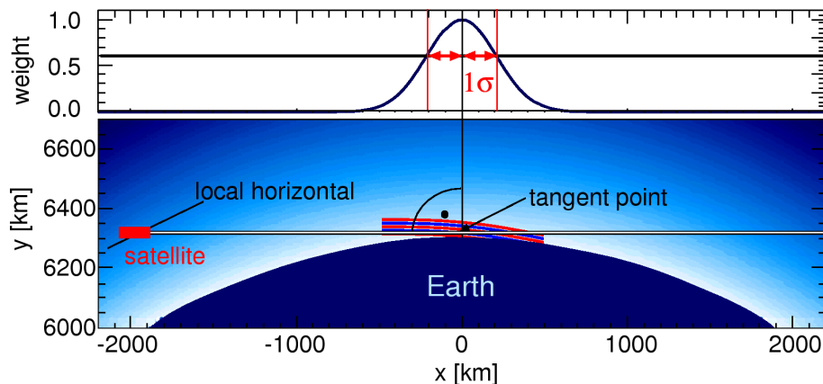
Fig. 1. Viewing geometry of a limb-sounding satellite. The upper panel shows the Gaussian-shaped weighting function along the limb ray. The lower panel indicates sounding of a GW of 400 km horizontal and 25 km vertical wavelength. The figure is up to scale. Note that the phase fronts of the GW are curved and coaligned with the limb ray to the left of the tangent point. For discussion see text.
