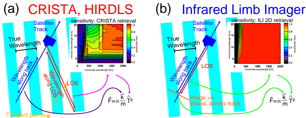
Fig. 2. Schematic drawing comparing GW sounding by (a) current generation satellites as e.g. CRISTA and HIRDLS with (b) a future ILI. The GW wave fronts are indicated by the light-blue shading, the satellite track by the dark-blue arrow, an exemplarily LOS in red, and various tangent points for subsequent profiles in orange. We here have chosen an orientation where wave fronts and satellite-track are oriented differently. The curved arrows from the LOS to the sensitivity function and further to the MF-equation as well as from the satellite track to the MF-equation indicate the main error sources of conventional limb sounders (panel a): degraded sensitivity and missing knowledge on the horizontal wave vector. For an ILI (panel b) backward view and dense along-track sampling result in the correct temperature amplitude; the across-track information by the image is used to determine the full wave vector. A more detailed discussion is given in the text.
