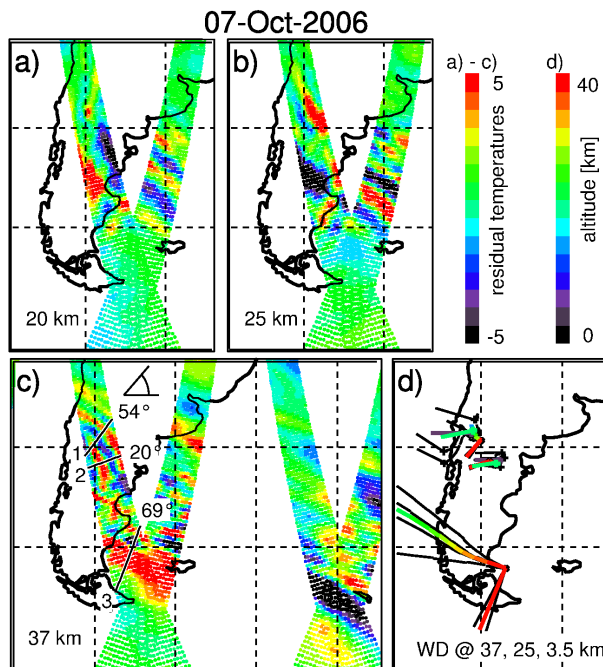
Fig. 5. ECMWF temperatures detrended by wavenumber 0–6 sampled on an ILI measurement grid for altitudes of 20 km (a), 25 km (b) and 37 km (c). At 37 km for three cases the GW propagation direction was determined and sections along these lines labeled 1, 2, and 3 are indicated by black lines. Wave parameters determined from these sections (see also Fig. 6) serve as input for back-tracing of the GWs to their source altitude. The results are shown in (d). For details see text.
