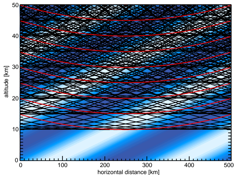
Fig. 3. Multiple limb rays for a horizontal sampling of 50 km and vertical sampling of 5 km (i.e. 10 times less than envisaged for an ILI) projected onto a GW of 300 km horizontal and 20 km vertical wavelength. For details see text.
