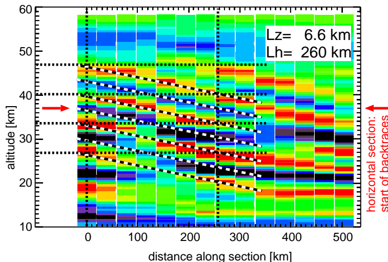
Fig. 6. Vertical section along the black line labeled “1” in Fig. 5c. From this section horizontal and vertical wavelength of the dominant GW can be determined and used as input parameter for backward ray tracing studies (see also Fig. 5). For details see text.
