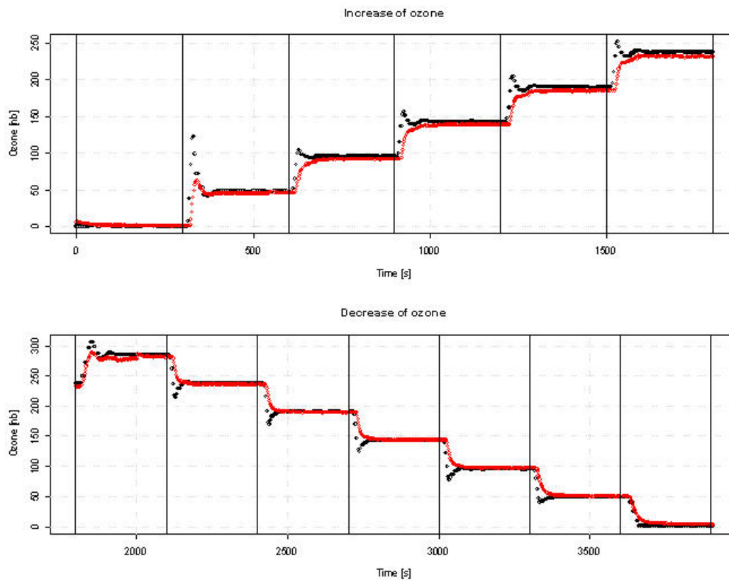
Fig. 1. Response of an ECC ozonesonde (ENSCI-0.5%).
