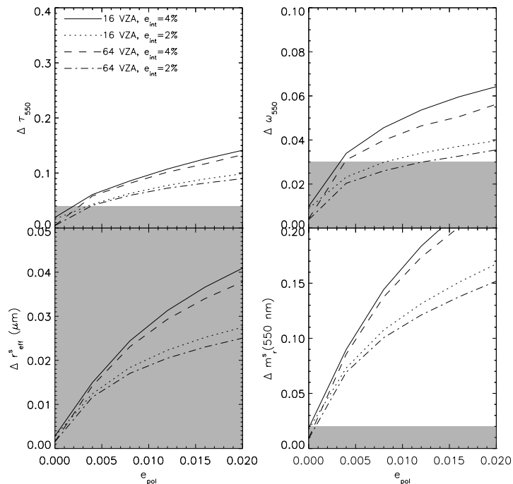
Fig. 5. Same as Fig. 4 but for errors that are correlated for different wavelengths and different viewing angles. Here, an exponential decay is assumed of the correlation with wavelength and viewing angle, where the correlation is reduced to 1/e for wavelength differences of 100 nm and viewing angle differences of 60^\circ .
