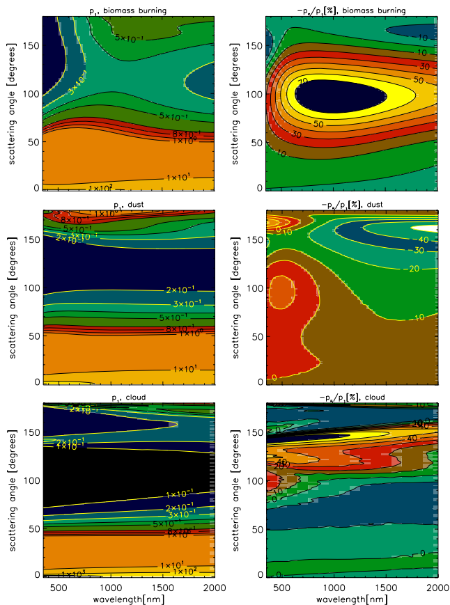
Fig. 1. Element p_1 (left panels) and signed degree of linear polarization -p_5/p_1 (right panels) of the scattering phase matrix as a function of wavelength and scattering angle for biomass burning aerosols (upper panels), dust aerosols (middle panels), and cloud particles (lower panel).
