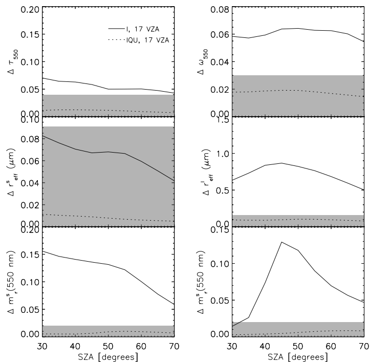
Fig. 3. As in Fig. 2, but for retrievals with unknown surface properties, and only considering multiple-viewing-angle measurements.
