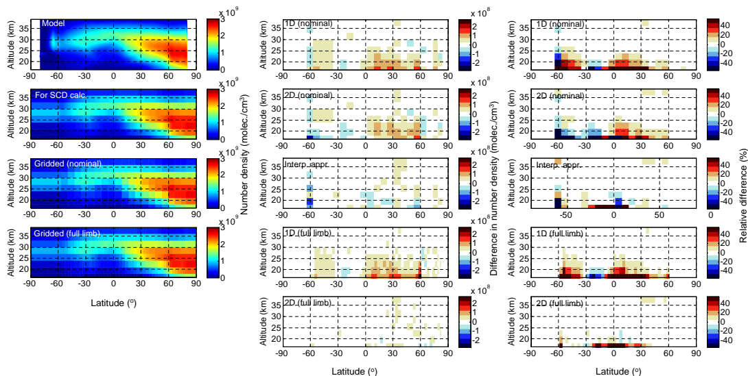
Fig. 19. Same as Fig. 15 but for 15 June 2007.
