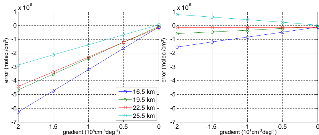
Fig. 13. The systematic error in the retrieved number density of \text{NO}_2 as function of the simulated gradient strength between 40^\circ and 50^\circ for the 1-D (left) and 2-D (right) retrieval approach. On the x-axis the gradient strength at the peak of the simulated profile (28.5 km) is given. The colored lines display the difference to the true simulated values at the respective altitudes (16.5 km to 25.5 km, see legend).
