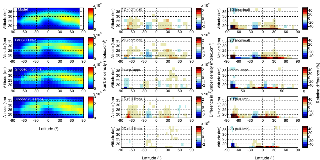
Fig. 20. Same as Fig. 15 but for 15 September 2007.
