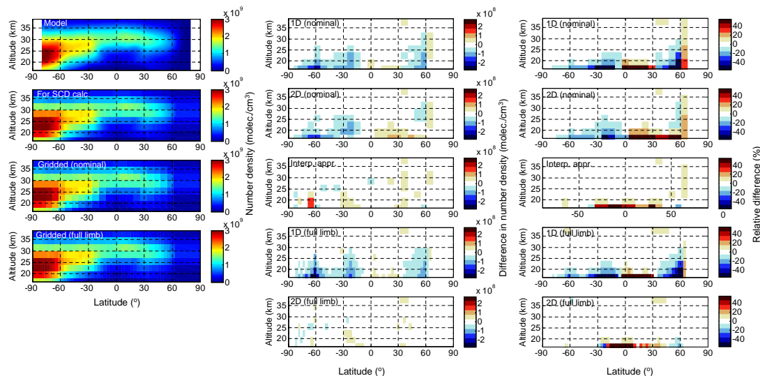
Fig. 15. Left panel: \text{NO}_2 number density field simulated by EMAC atmospheric chemistry general circulation model for 15 December 2007 (top), gridded for the simulation of SCDs with fine horizontal resolution (second row), and gridded to the resolution of the SCIAMACHY limb measurements in the nominal and full limb operational modes (third and bottom row). In the middle and right panels absolute and relative differences between the \text{NO}_2 distribution retrieved from the simulated SCDs and the true (simulated) number density field are shown. The first three panels from top show results for the simulated measurements with the distance of 7.5^\circ of the orbital cycle between consecutive scanning sequences. From top to bottom the differences plotted are for the 1-D approach, the 2-D approach and the interpolation approach. In the two bottom panels, the results for the distance of 3.3^\circ (i.e. full limb mode) are shown for the 1-D and 2-D approach.
