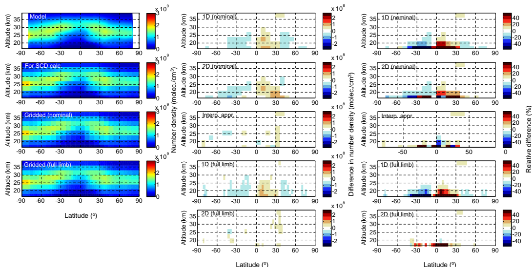
Fig. 18. Same as Fig. 15 but for 15 March 2007.
