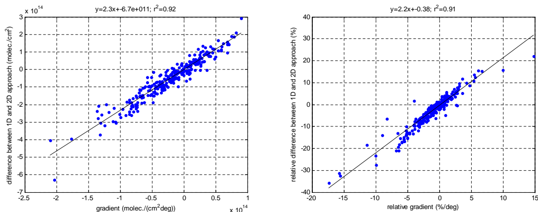
Fig. 10. Scatter plot between the gradient in the stratospheric NO 2 columns between 15 and 40 km as observed for the 2-D retrieval (between two consecutive scanning sequences) and the difference between the NO 2 columns retrieved by the 1-D and 2-D approach. On the left panel: correlation plots between absolute values, on the right: the same for relative values (normalized by the vertical column acquired by the 2-D retrieval).
