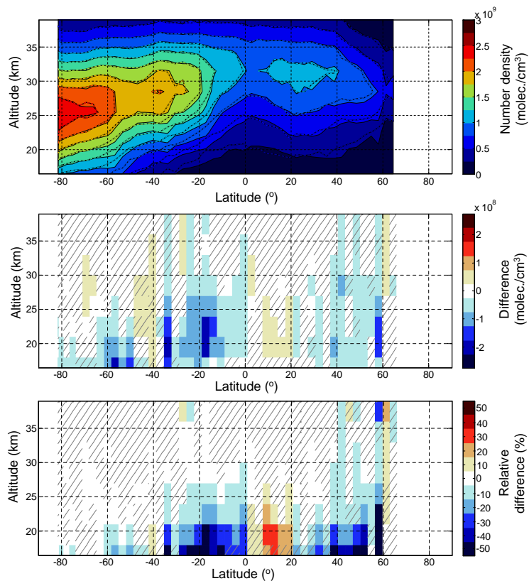
Fig. 6. Top panel: vertical and latitudinal distribution of the mean NO 2 number density for all six full limb orbits on 14 December 2008 retrieved by the 2-D approach (color plot with solid contourlines) and the 1-D approach (dashed contourlines). Middle and bottom panels: absolute and relative difference between results from the 1-D and 2-D approach for the retrieval boxes. Boxes where the retrieval error is larger than the difference are shaded by a diagonal pattern.
