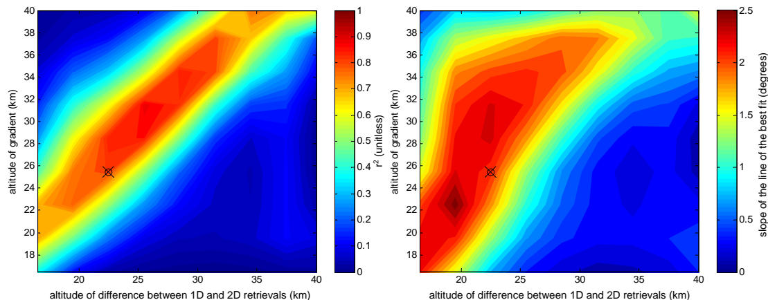
Fig. 9. Left: correlation coefficient ( r^2 ) between gradients (calculated by Eq. 4) occurring at different altitudes and the difference between the 1-D and 2-D retrieval. Right: same as before but now the slope of the line of the best fit is shown. Values for the example plotted in Fig. 8 are indicated with a crossed circle.
