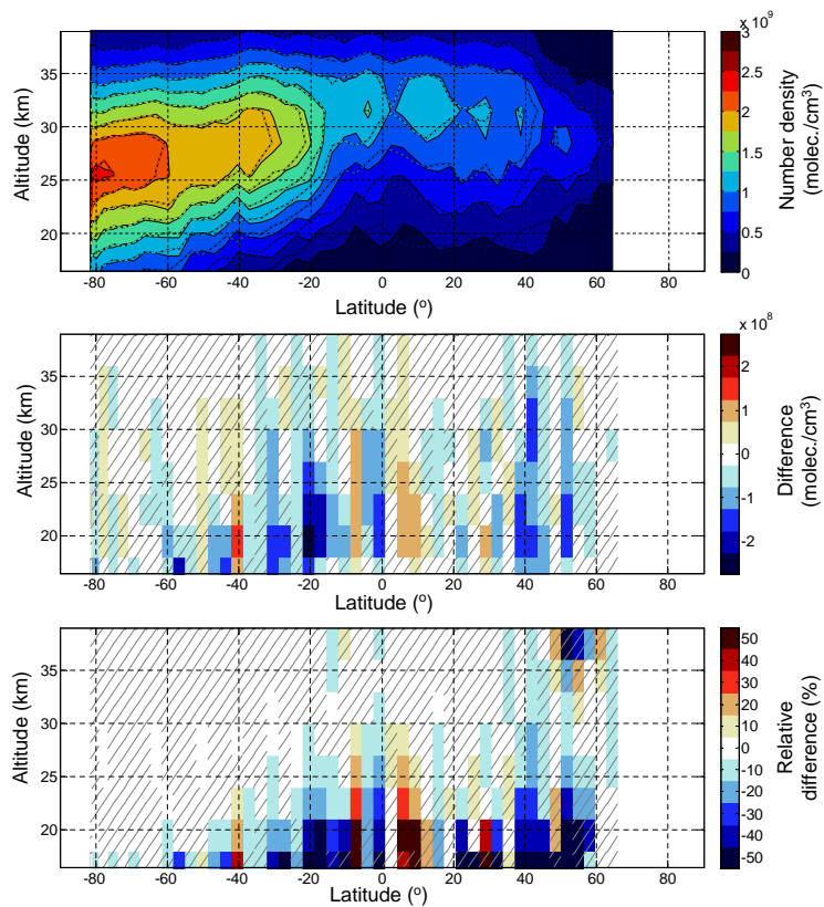
Fig. 5. Same as Fig. 4 but for orbit 35503.
