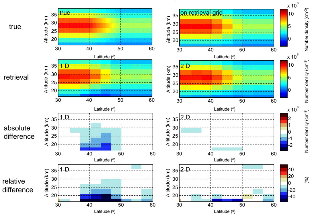
Fig. 11. Upper panel left: assumed \text{NO}_2 distribution with a negative gradient towards the instrument. Upper panel right: the same profiles but gridded on the SCIAMACHY retrieval grid. Second panel: \text{NO}_2 profiles obtained by the 1-D retrieval (left) and 2-D retrieval (right). The absolute and relative differences between the original (true) profile averaged on the SCIAMACHY retrieval grid and the retrievals for the simulations are shown in the third and bottom panel, respectively.
