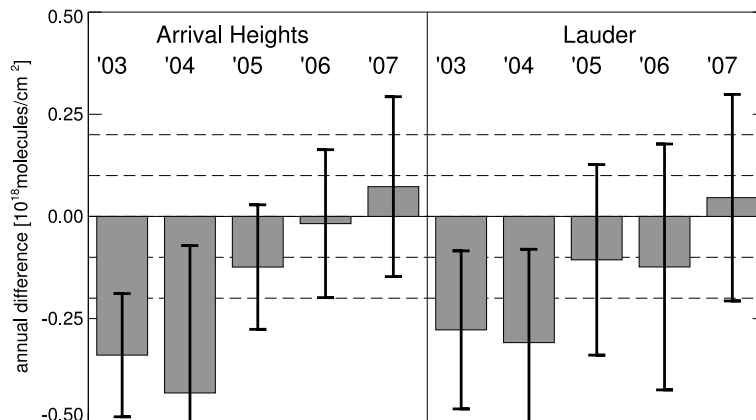
Fig. 5e. Annual mean SCIAMACHY-GBS CO total column differences for the years 2003–2007 for Arrival Heights and Lauder in 10^{18} molecules/cm ^2 based on the results presented in Fig. 5a. The dashed lines indicate the \pm 1\text{-}\sigma or 2\text{-}\sigma SCIAMACHY precision ( 0.1 \times 10^{18} molecules/cm ^2 ). The error bars indicate the 1\text{-}\sigma rms differences.
