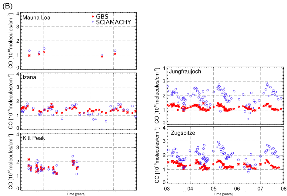
Fig. 5b. As Fig. 5A but for five Northern Hemisphere mountain stations. For Izaña and Mauna Loa SCIAMACHY CO columns with cloud top heights comparable to the station altitude were used (see text).
