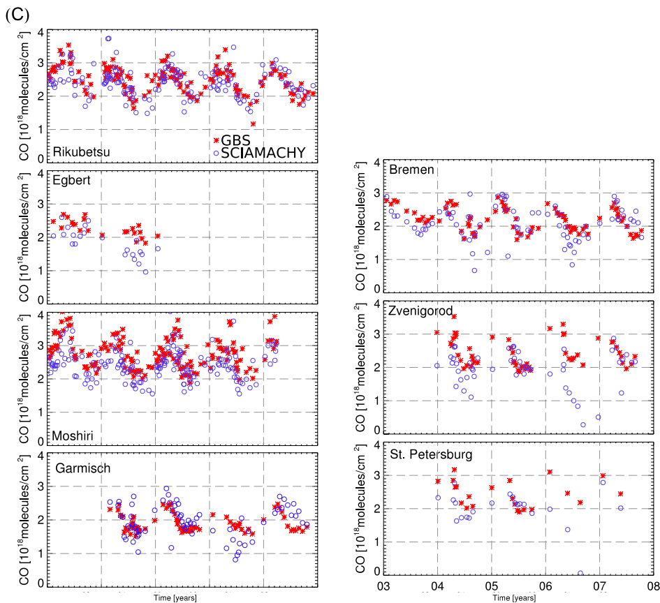
Fig. 5c. As Fig. 5A but for seven Northern Hemisphere mid-latitude stations.
