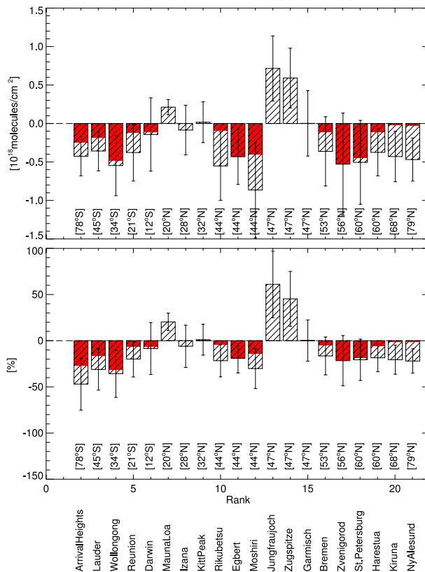
Fig. 6. Average differences between SCIAMACHY and GBS CO column measurements over the 2003–2007 period for an 8 \times 8^\circ sampling area (Table 2). The dashed bars indicate the average differences around the mean, the error bars indicate the root-mean-square of the differences and the solid red bars indicate the differences after adding the estimated TM4 column below the cloud for SCIAMACHY ocean measurements (not applied for Northern Hemisphere mountain stations).
