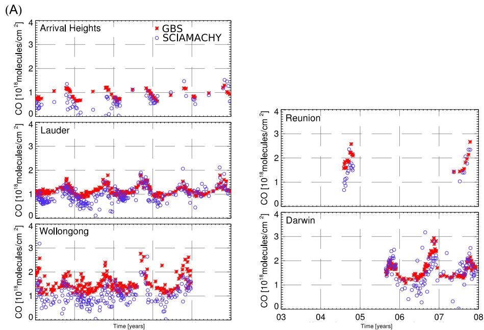
Fig. 5a. Time series of the SCIAMACHY-GBS comparison for five Southern Hemisphere stations for the results presented in Fig. 4. For SCIAMACHY ocean measurements the estimated TM4 column below the cloud has been added to the SCIAMACHY CO partial column.
