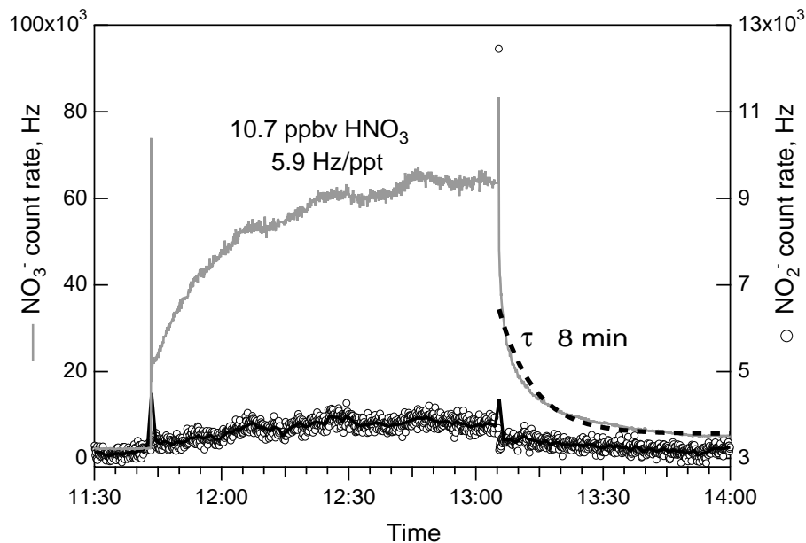
Fig. 5. The response of the NI-PT-CIMS to addition of the nitric acid standard directly before the ion flow tube. The nitric acid signal is shown in gray, the system response to removal of the nitric acid can be fit with an exponential line (dashed line). The signal in the nitrous acid channel (mass 46) is shown as open circles with the solid black line denoting the 60-s average.
