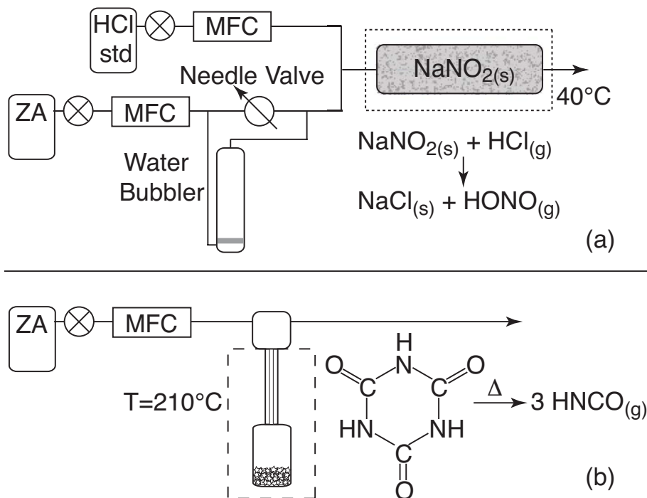
Fig. 2. Systems used to produce dilute streams of HCl and HONO (a), and HNCO (b) for the calibration of the NI-PT-CIMS instrument.
