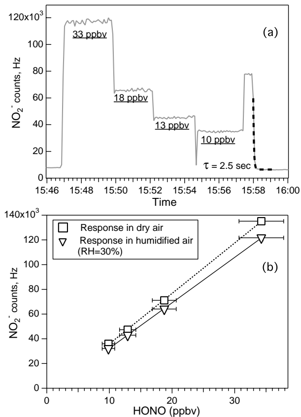
Fig. 4. Panel (a) shows the response of the NI-PT-CIMS to the HONO standard (gray line), introduced through the entire inlet. The simple exponential fit to the HONO signal when the standard was removed (dashed line) is also shown. Panel (b) shows the results of HONO calibrations under dry (squares) and 30% humidity (triangles).
