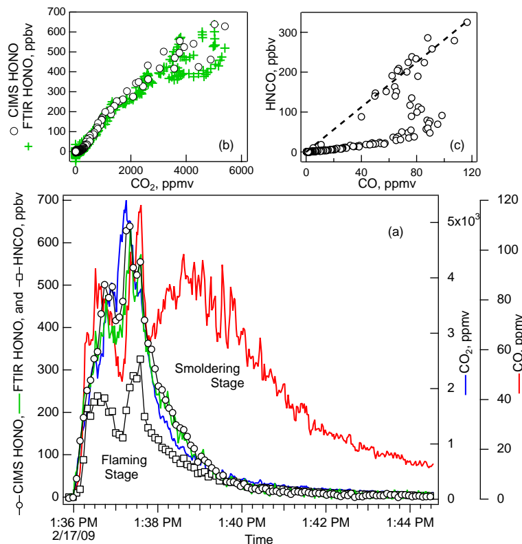
Fig. 8. A timeline (a) for the emission of: HONO measured by CIMS (open circles) and by FTIR (green line), HNCO (open squares), CO 2 (blue line) and CO (red) during a biomass burning experiment. Also shown is (b) the correlation of both HONO measurements with CO 2 and (c) the correlation of HNCO with CO, showing the correlation with flaming-stage CO of 0.28% (dashed line).
